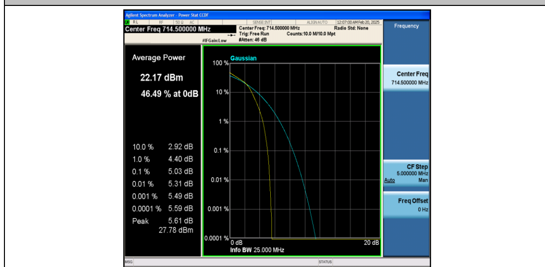
Band12-3MHz-16QAM-23165-15RB#0-PASS
