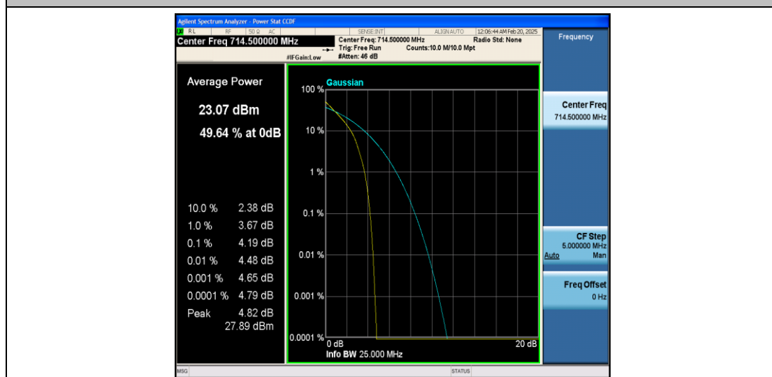
Band12-3MHz-QPSK-23165-15RB#0-PASS
