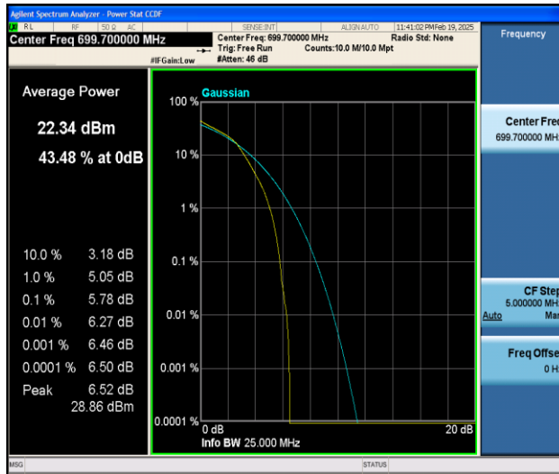
Band12-1.4MHz-16QAM-23017-6RB#0-PASS
