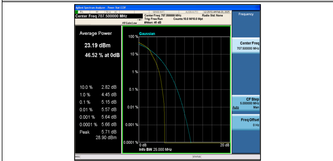
Band12-5MHz-16QAM-23095-1RB#0-PASS
