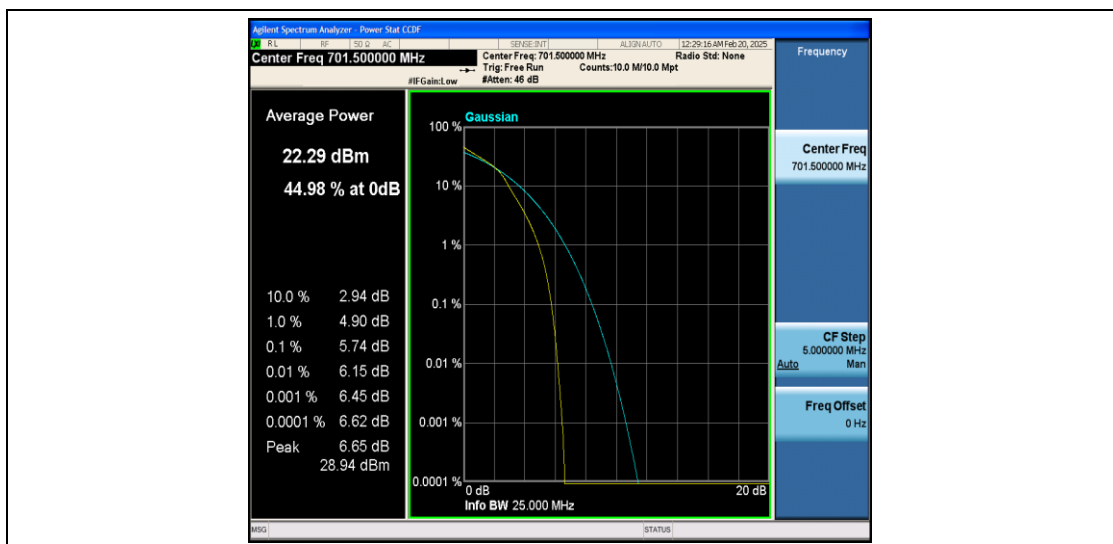
Band12-5MHz-16QAM-23035-25RB#0-PASS
