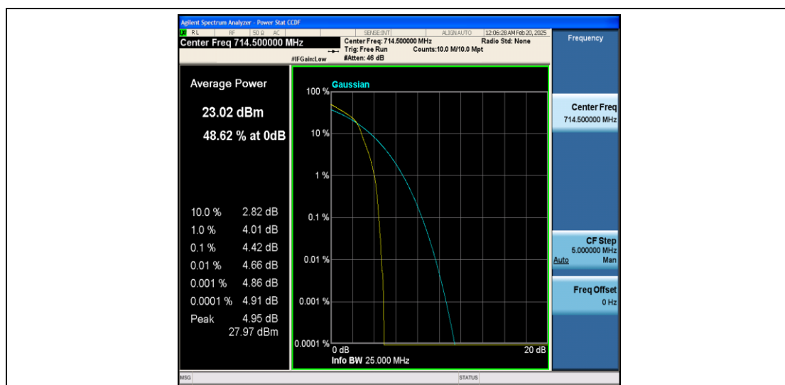
Band12-3MHz-16QAM-23165-1RB#0-PASS
