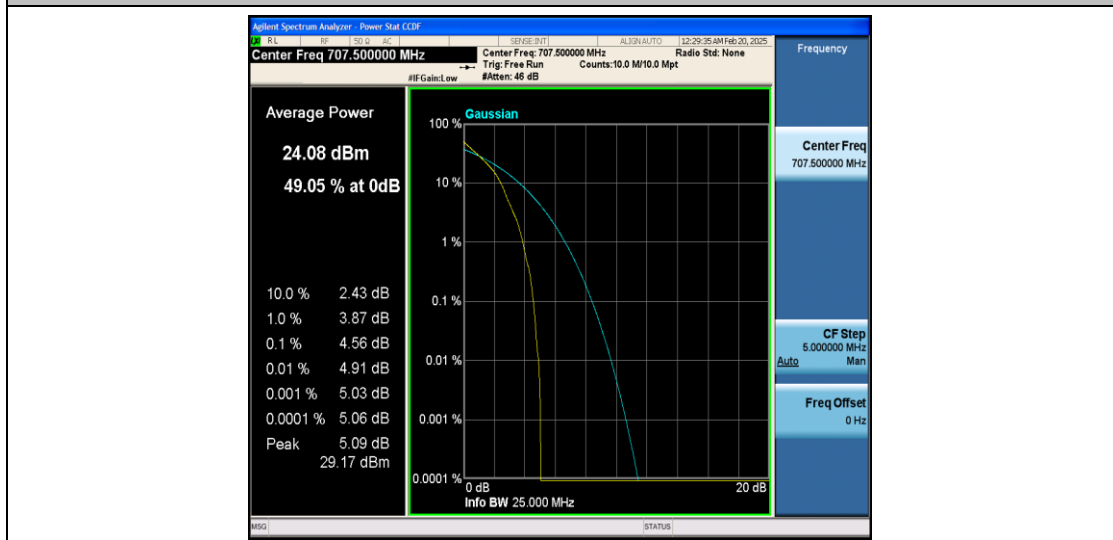
Band12-5MHz-QPSK-23095-1RB#0-PASS
