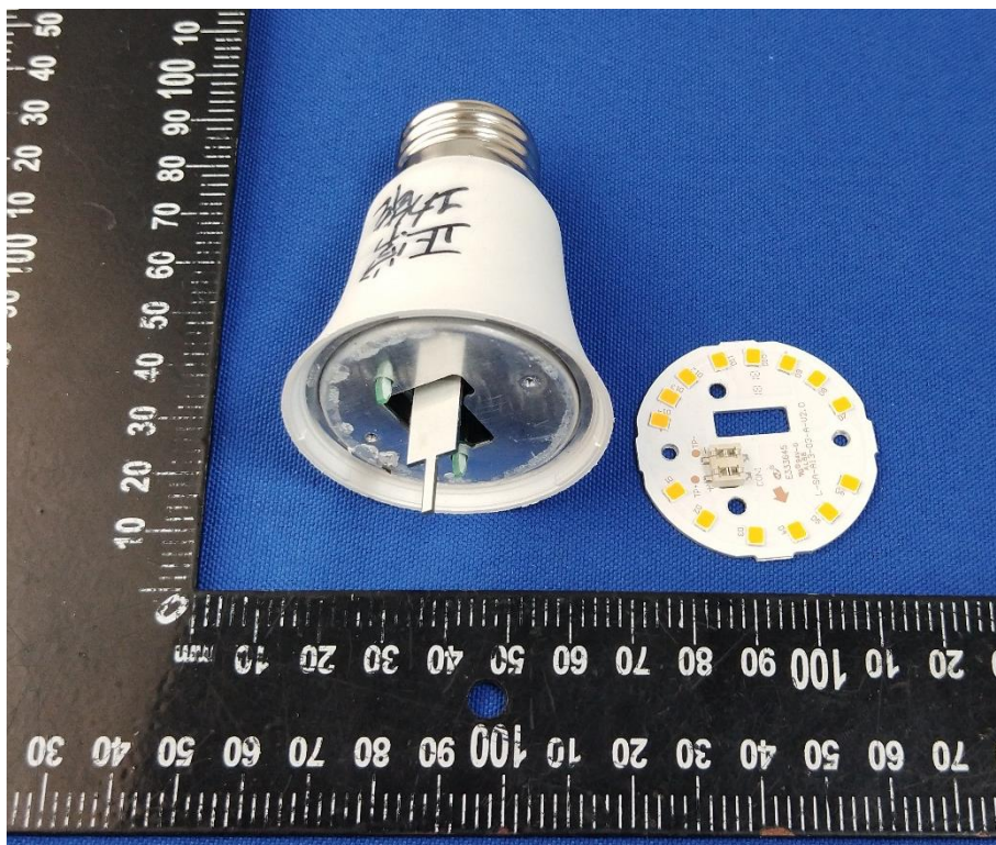
EUT UNCOVER VIEW 2
