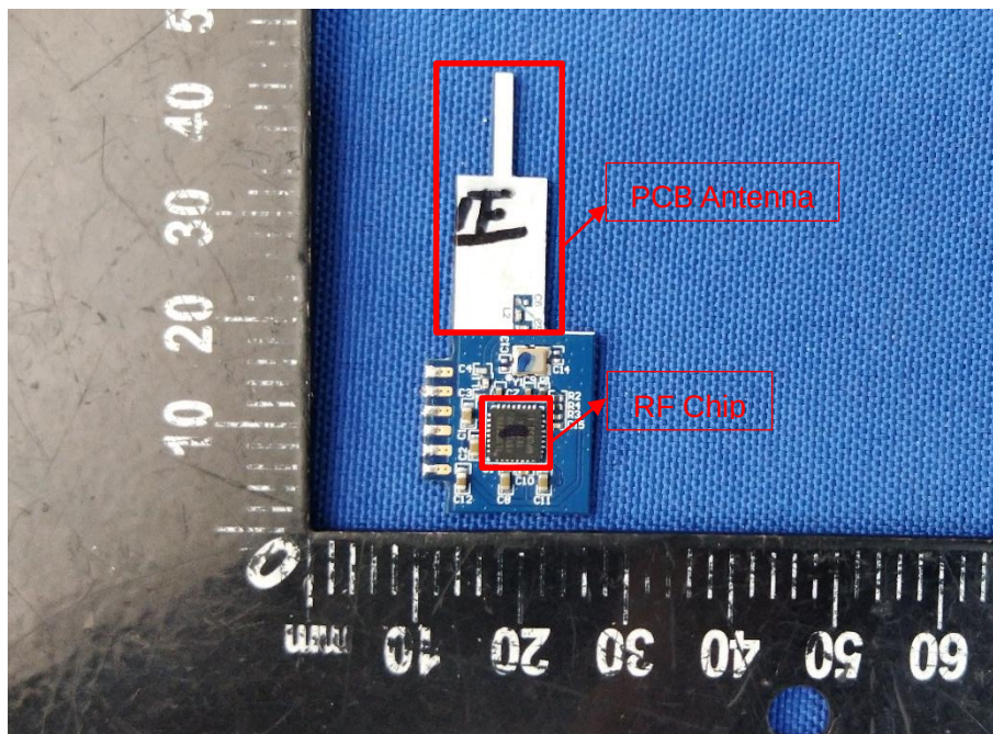
MAIN BOARD TOP VIEW 3
