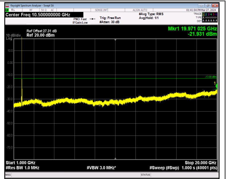
Band66_20MHz_16QAM_132572_1RB#0_1000~20000_1000~20000
