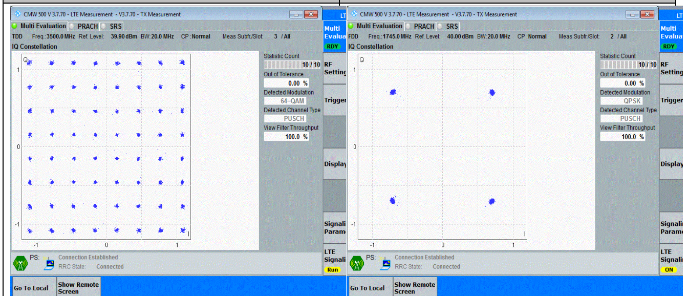
42(3450-3550)-20MHz-64QAM-42590-100RB#0-PASS
