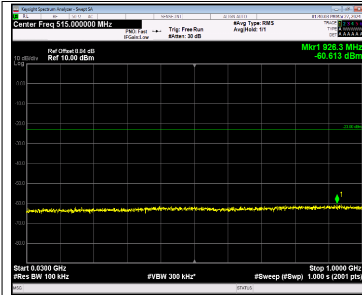
Band66_20MHz_64QAM_132322_1RB#0_30~1000_30~1000
