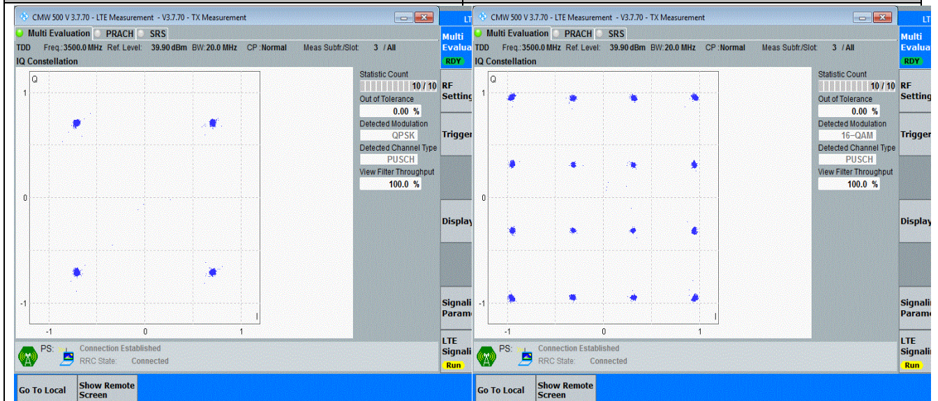
42(3450-3550)-20MHz-QPSK-42590-100RB#0-PASS
