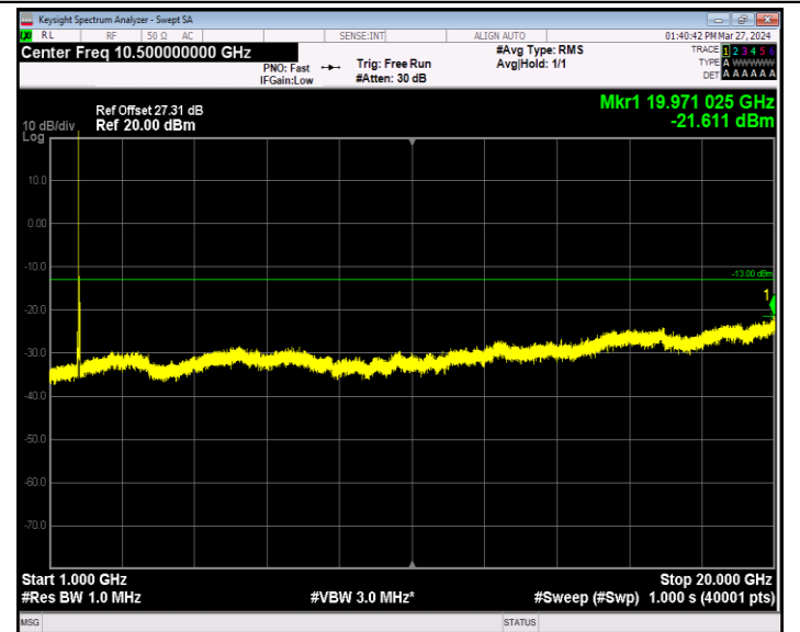
Band66_20MHz_QPSK_132572_1RB#0_1000~20000_1000~2000
