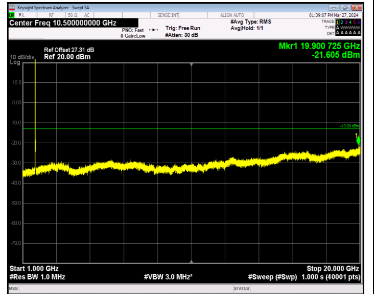
Band66_20MHz_64QAM_132072_1RB#0_1000~20000_1000~20000
