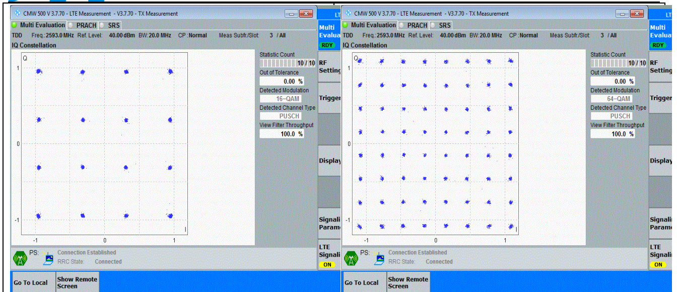
Band41-20MHz-16QAM-40620-100RB#0-PASS
