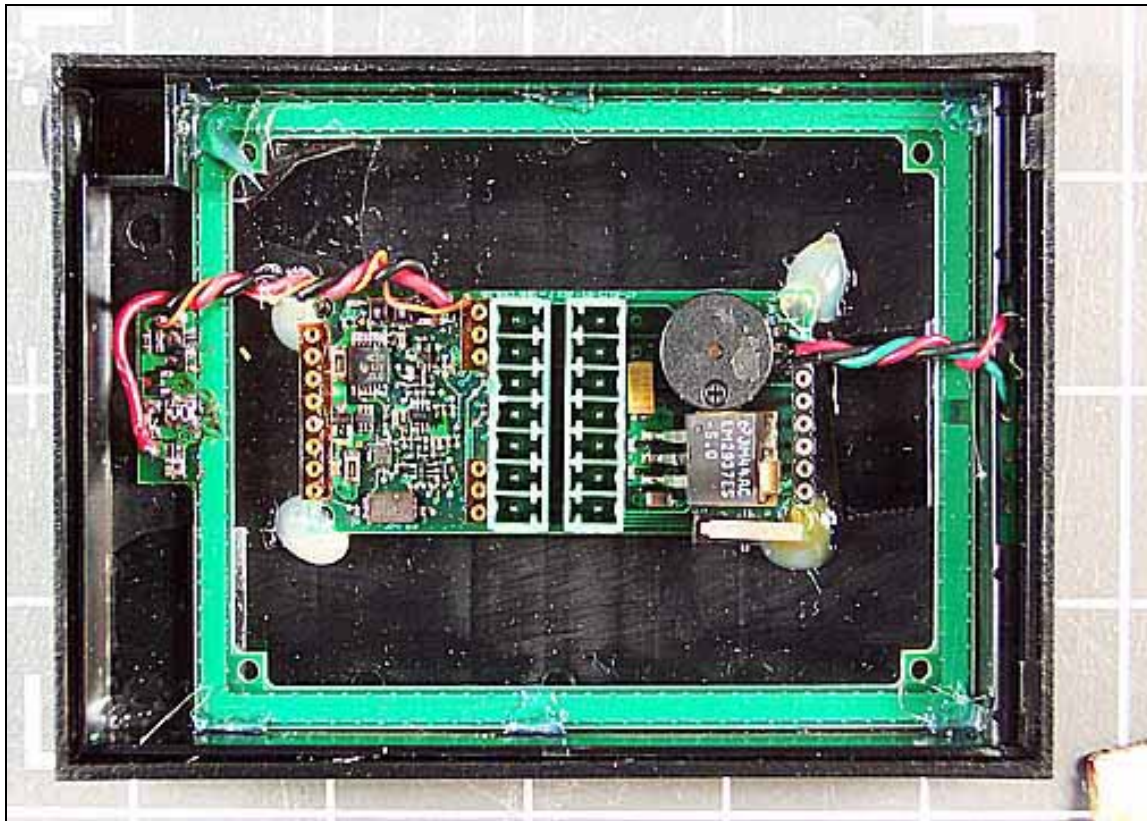
6121BxU iCLASS RW400 Inside Back Cover Without Module
