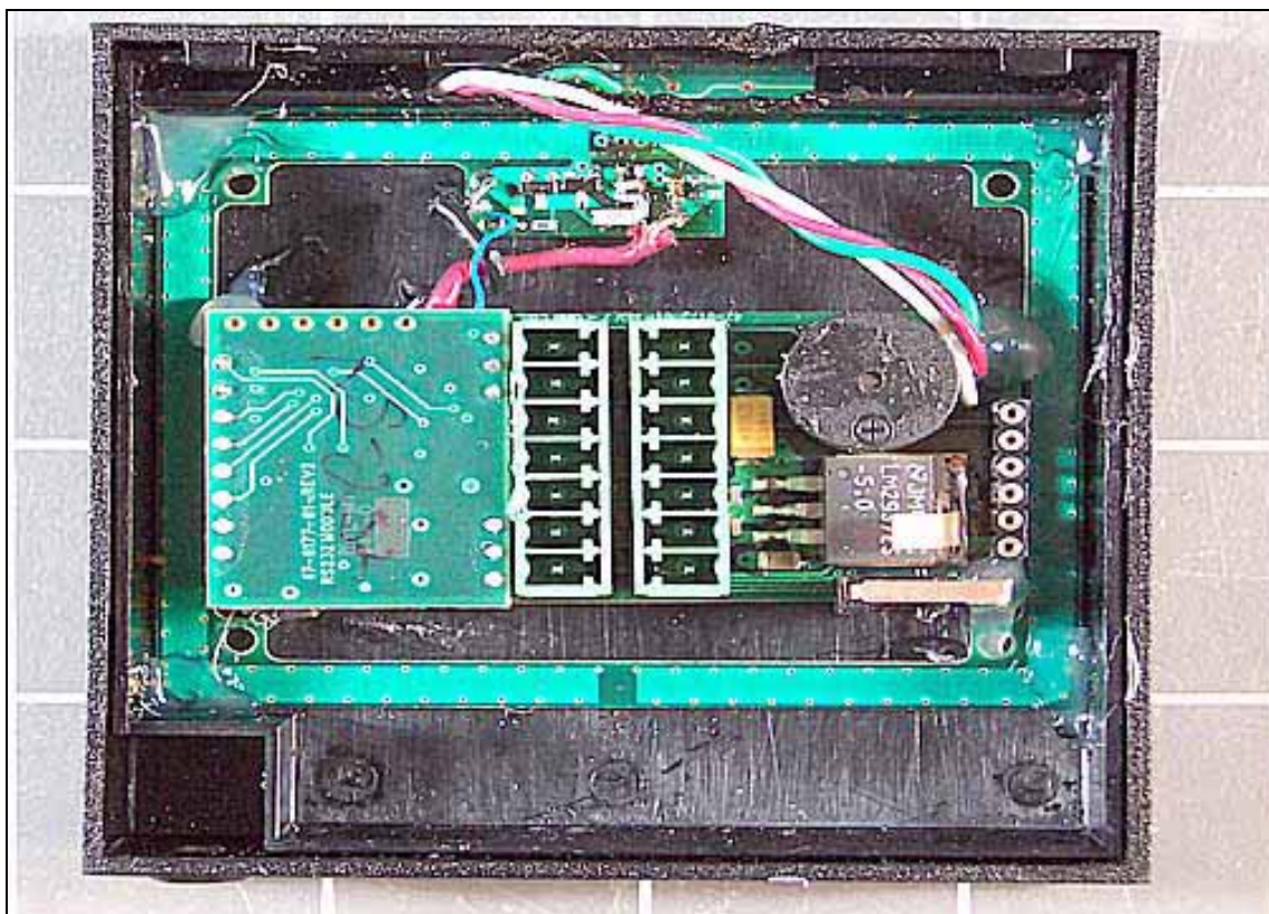
6111BxU iCLASS RW300 Inside Back Cover
