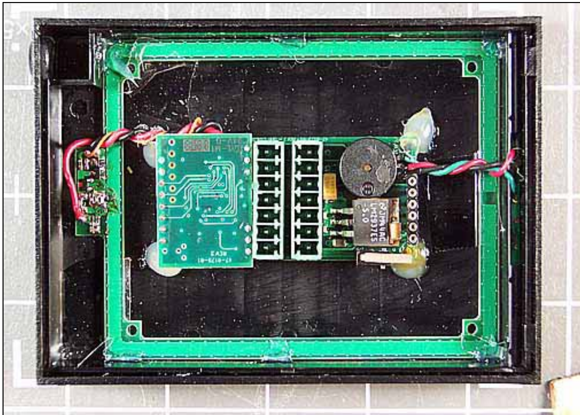
6121BxU iCLASS RW400 Inside Back Cover
