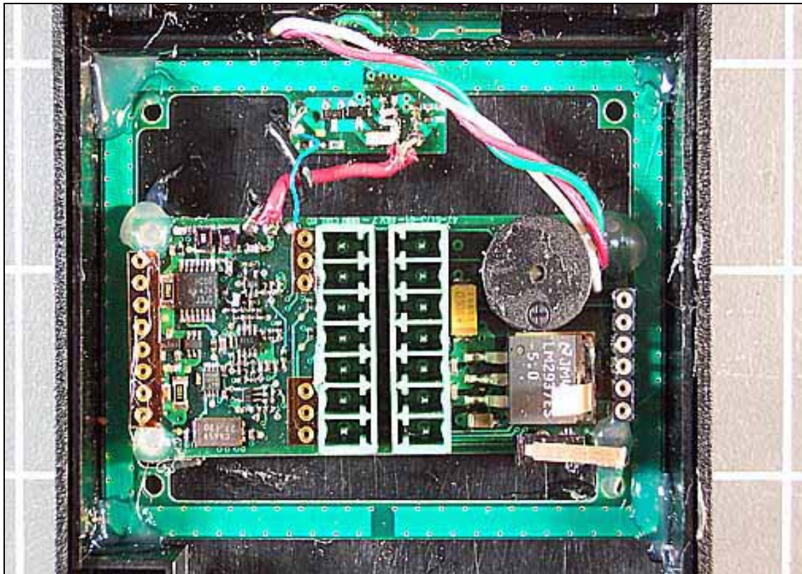
6111BxU iCLASS RW300 Inside Back Cover Without Module
