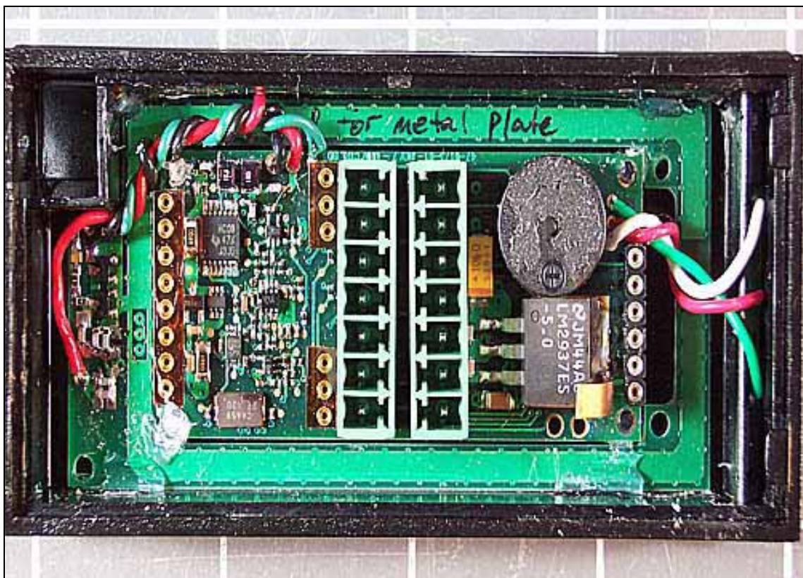
6101BxU iCLASS RW100 Inside Back Cover Without Module
