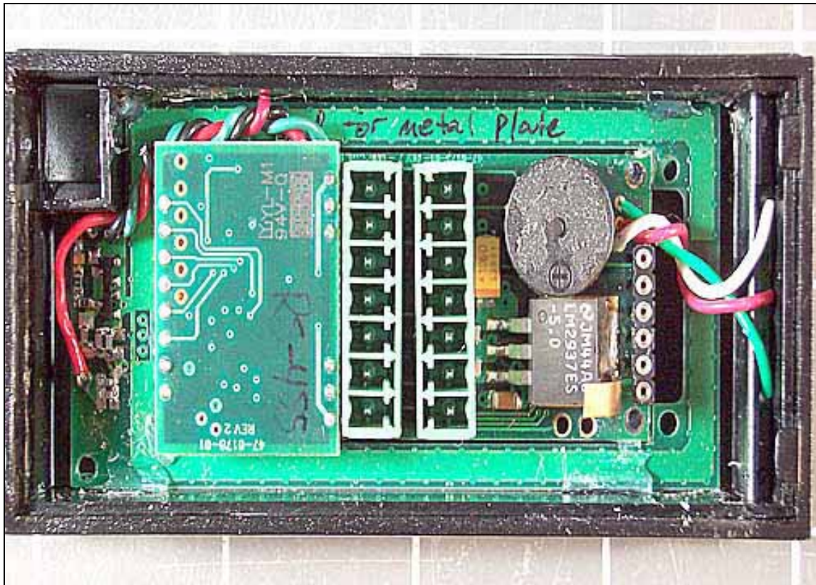
6101BxU iCLASS RW100 Inside Back Cover
