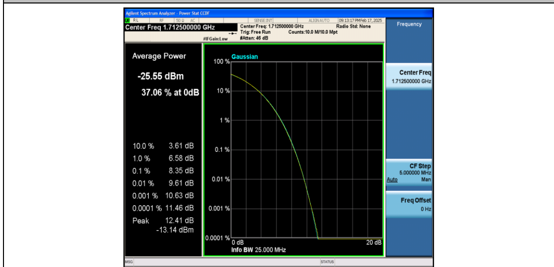
Band66-5MHz-16QAM-131997-25RB#0-PASS
