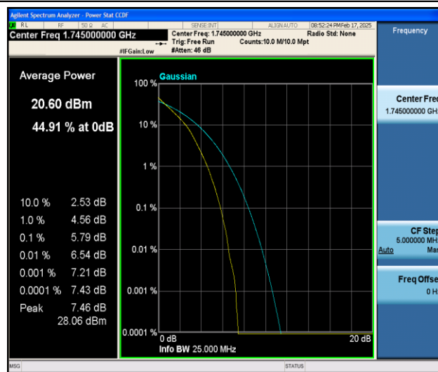
Band66-3MHz-QPSK-132322-15RB#0-PASS
