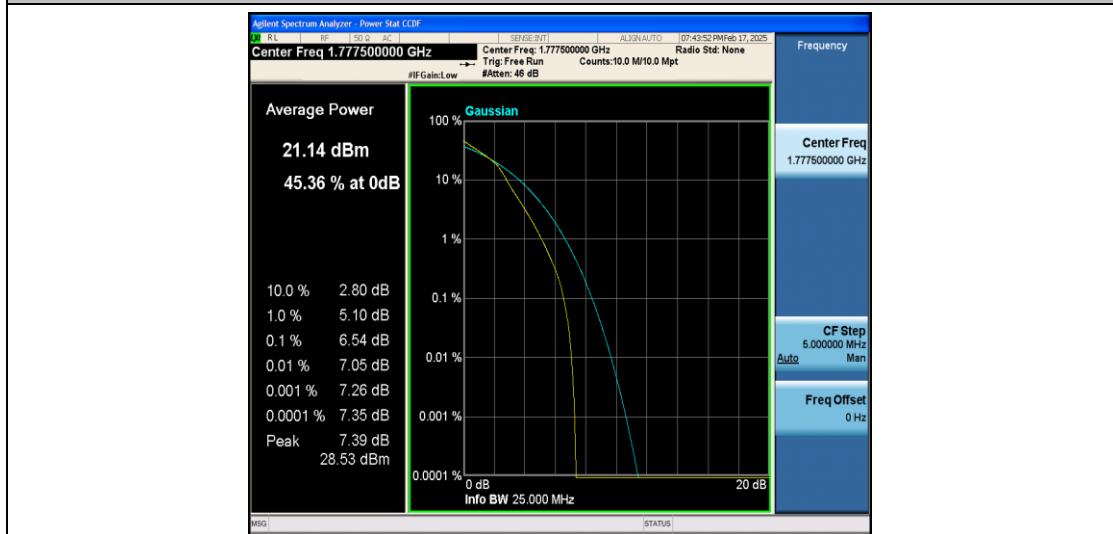
Band66-5MHz-16QAM-132647-25RB#0-PASS
