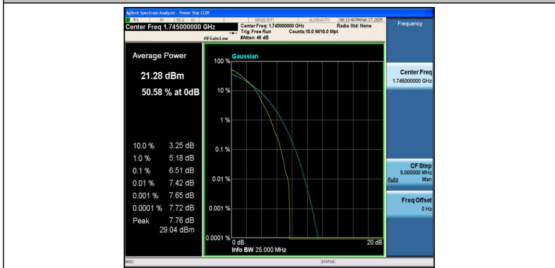
Band66-5MHz-QPSK-132322-1RB#0-PASS
