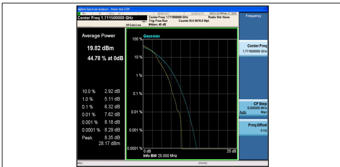
Band66-3MHz-16QAM-131987-1RB#0-PASS
