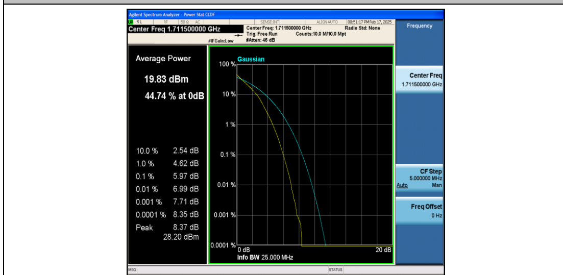
Band66-3MHz-QPSK-131987-15RB#0-PASS
