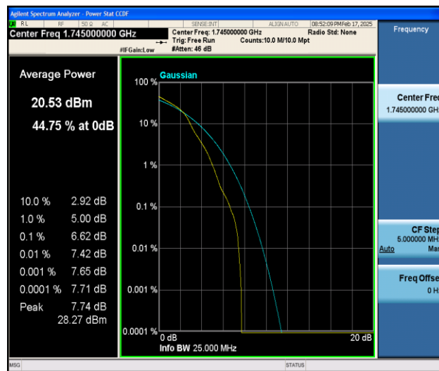
Band66-3MHz-16QAM-132322-1RB#0-PASS
