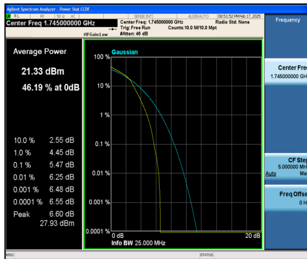
Band66-3MHz-QPSK-132322-1RB#0-PASS
