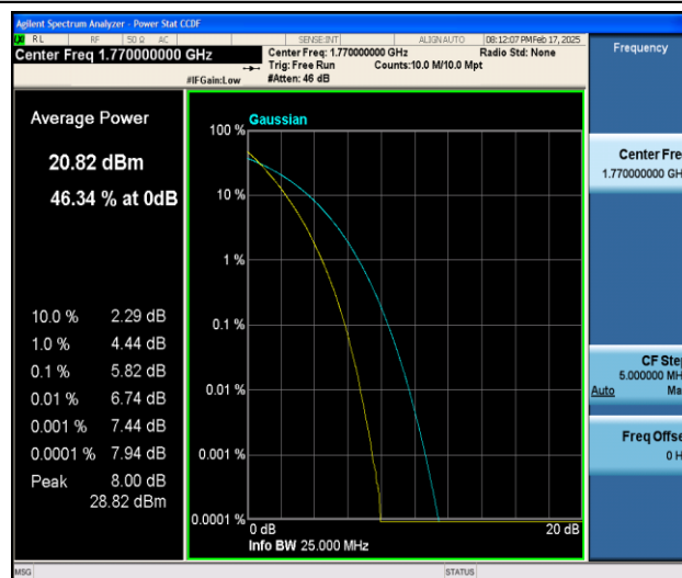
Band66-20MHz-QPSK-132572-100RB#0-PASS
