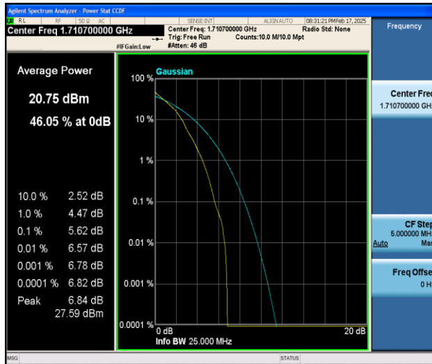
Band66-1.4MHz-QPSK-131979-1RB#0-PASS
