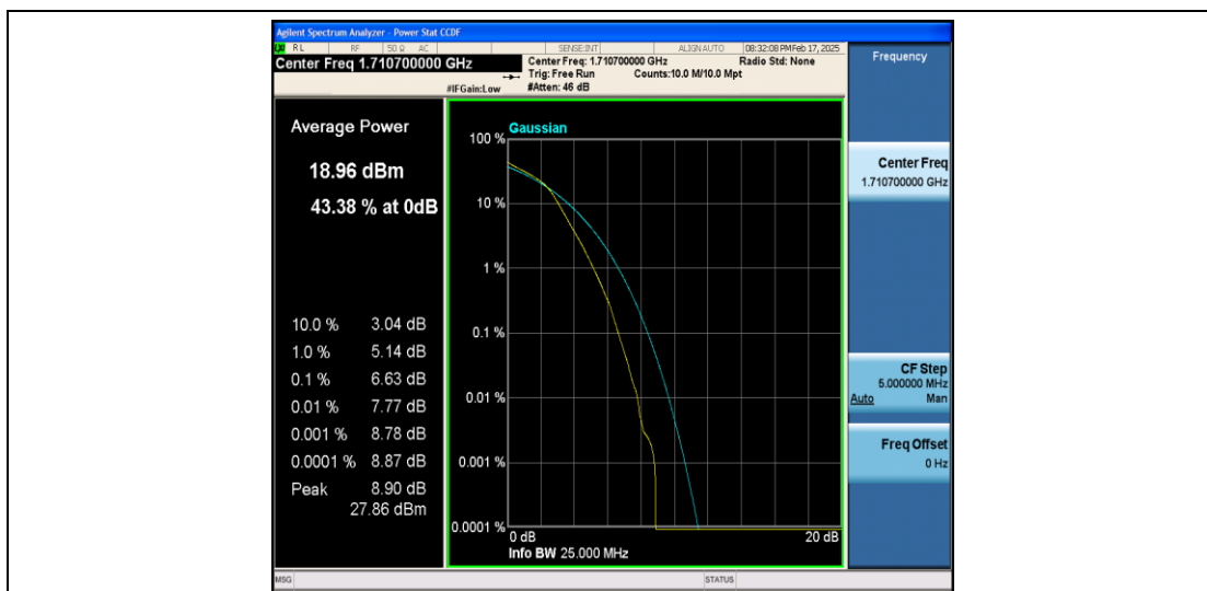
Band66-1.4MHz-16QAM-131979-6RB#0-PASS
