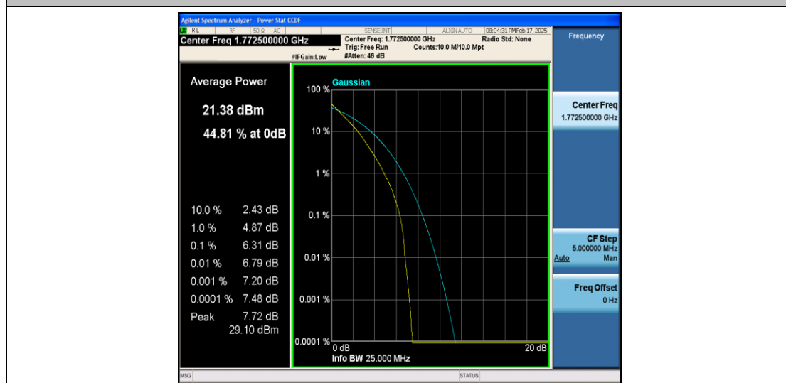
Band66-15MHz-QPSK-132597-75RB#0-PASS
