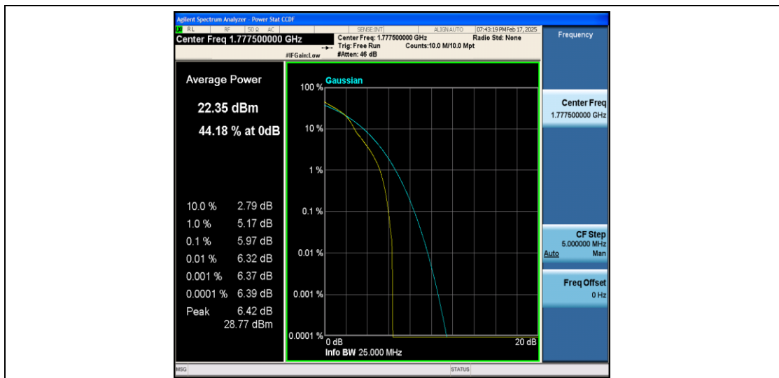
Band66-5MHz-16QAM-132647-1RB#0-PASS
