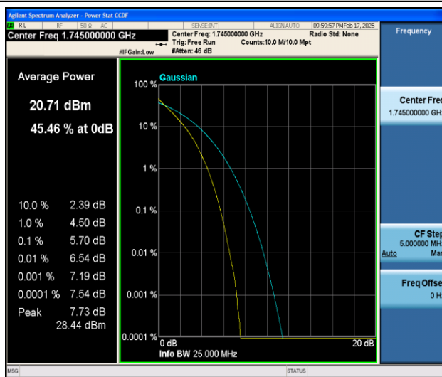
Band66-10MHz-QPSK-132322-50RB#0-PASS
