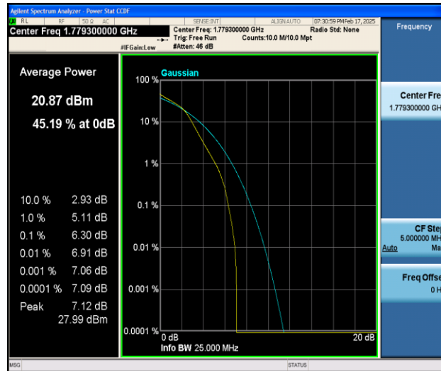
Band66-1.4MHz-16QAM-132665-6RB#0-PASS
