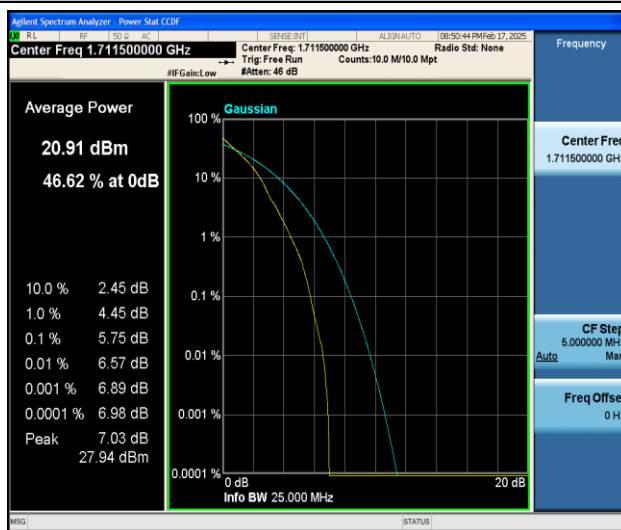
Band66-3MHz-QPSK-131987-1RB#0-PASS
