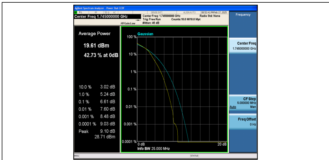
Band66-3MHz-16QAM-132322-15RB#0-PASS
