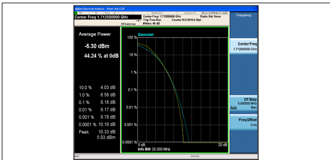
Band66-5MHz-QPSK-131997-25RB#0-PASS
