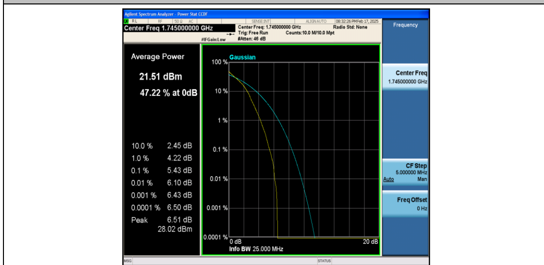
Band66-1.4MHz-QPSK-132322-1RB#0-PASS
