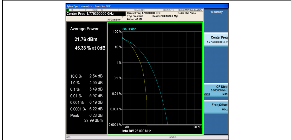
Band66-1.4MHz-QPSK-132665-6RB#0-PASS
