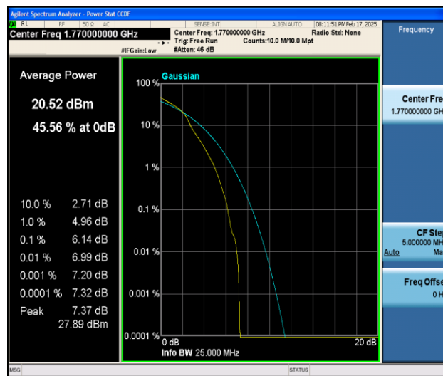
Band66-20MHz-16QAM-132572-1RB#0-PASS
