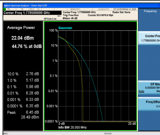
Band66-3MHz-16QAM-132657-1RB#0-PASS
