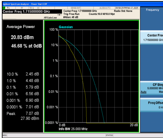
Band66-10MHz-QPSK-131022-1RB#0-PASS
