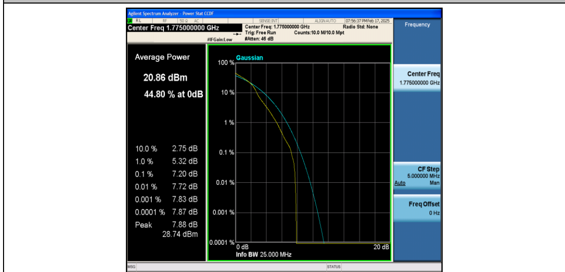
Band66-10MHz-16QAM-132622-1RB#0-PASS
