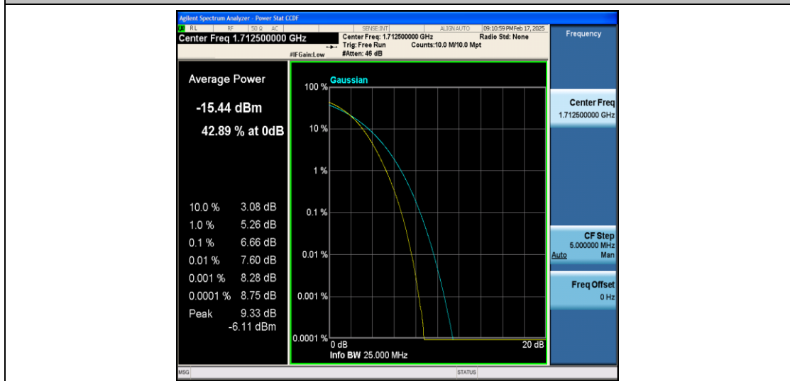
Band66-5MHz-16QAM-131997-1RB#0-PASS
