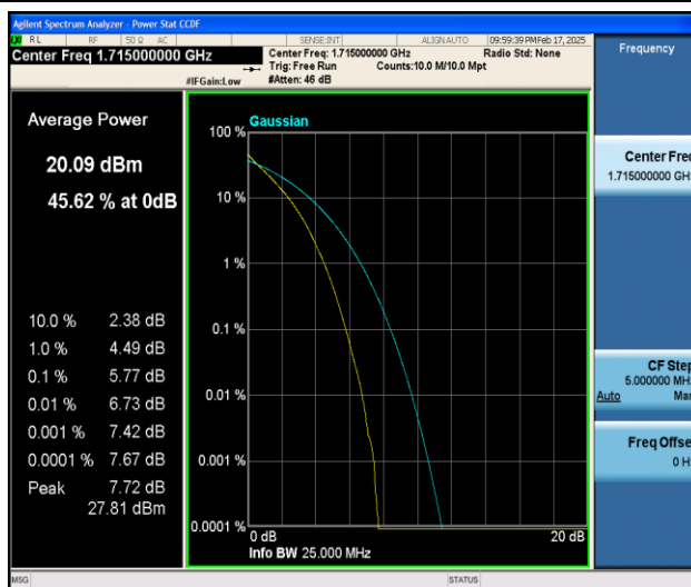
Band66-10MHz-QPSK-131022-50RB#0-PASS
