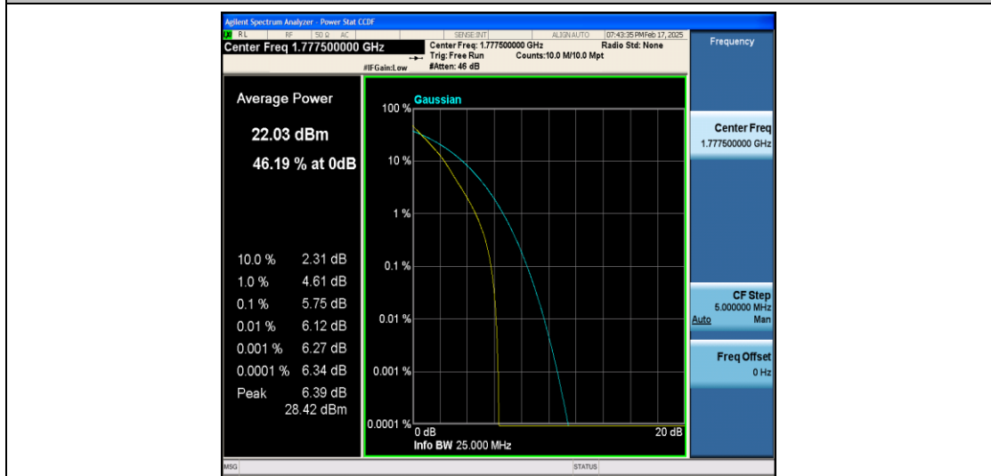
Band66-5MHz-QPSK-132647-25RB#0-PASS
