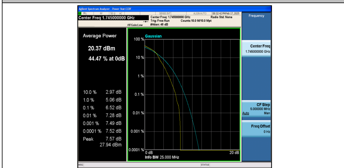
Band66-1.4MHz-16QAM-132322-1RB#0-PASS
