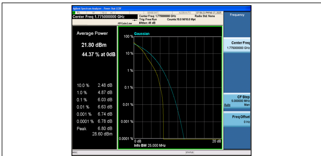
Band66-10MHz-QPSK-132622-1RB#0-PASS
