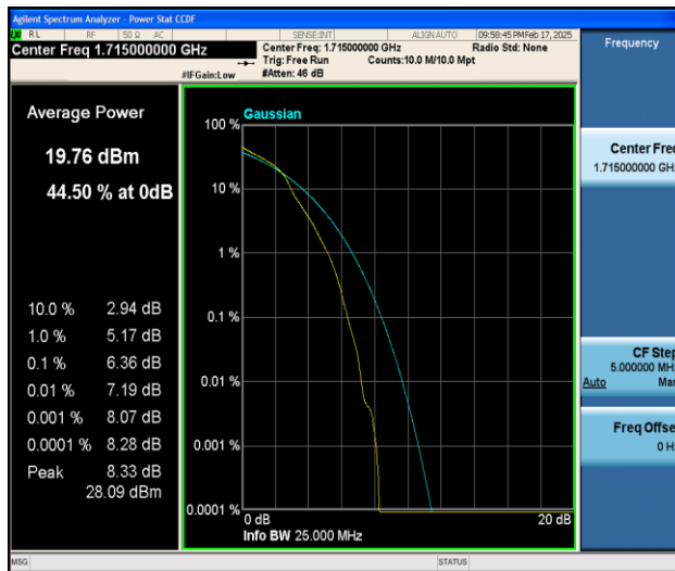
Band66-10MHz-16QAM-131022-1RB#0-PASS
