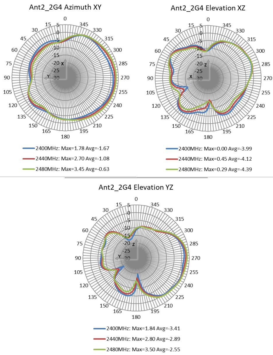
Figure 3: Model N01FVAE Radiation Patterns at 2.4 GHz & 2.44 GHz & 2.48 GHz
