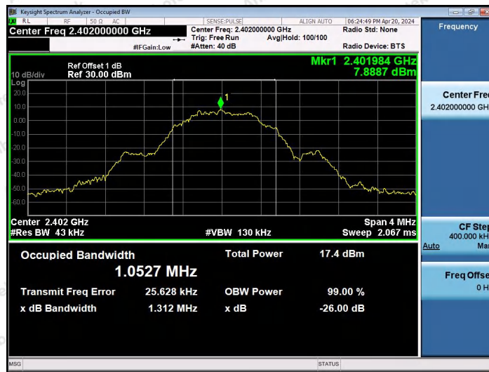
BLE_1M-Ant2-2402
