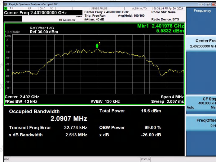
BLE_2M-Ant2-2402
