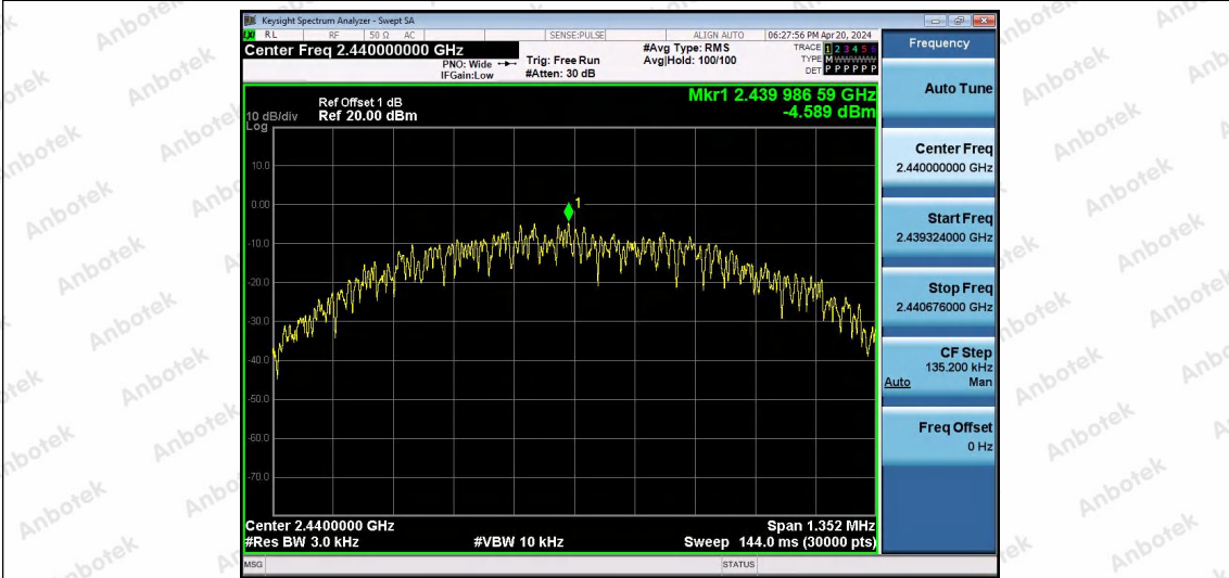
BLE_1M-Ant2-2440-PASS
