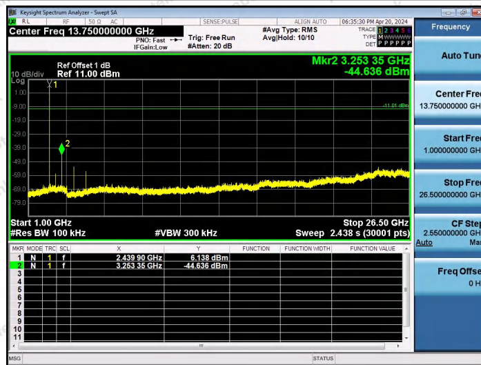
BLE_2M-Ant2-2440-1000~26500-PASS
