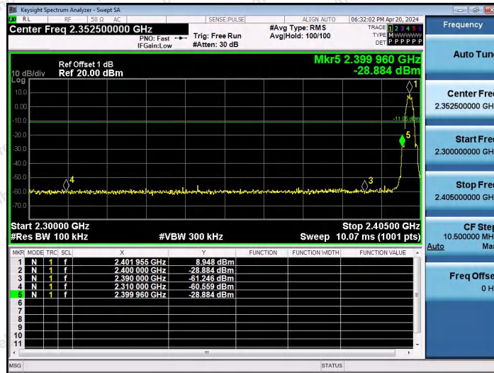
BLE_2M-Ant2-240-PASS
