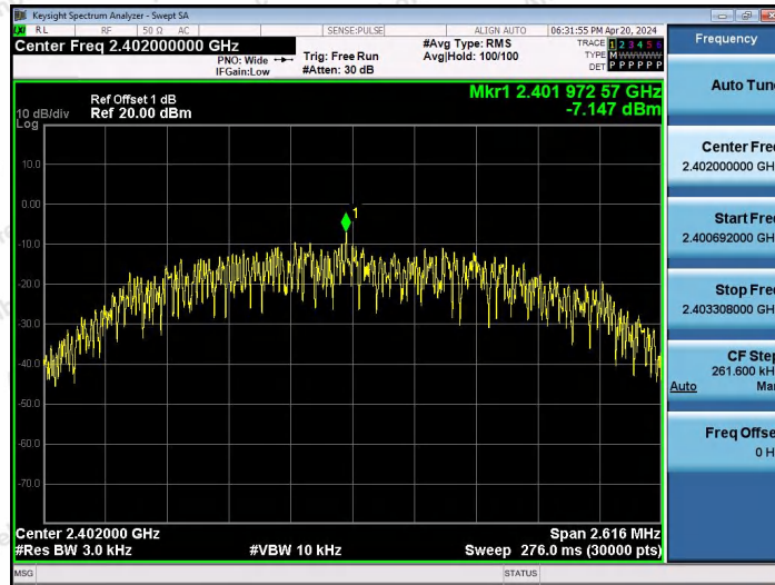
BLE_2M-Ant2-2402-PASS
