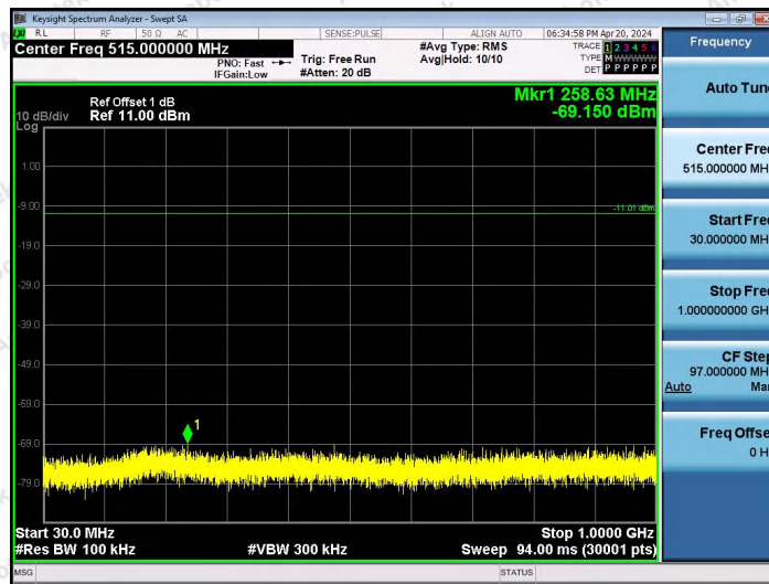
BLE_2M-Ant2-2440-30~1000-PASS
