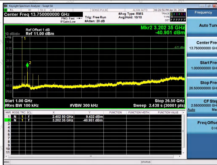
BLE_1M-Ant2-2402-1000~26500-PASS
