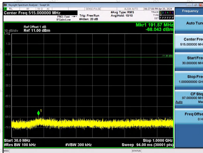
BLE_2M-Ant2-2480-30~1000-PASS
