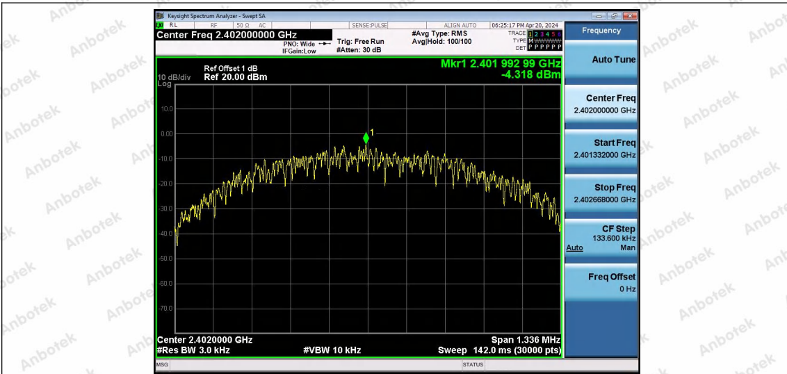
BLE_1M-Ant2-2402-PASS
