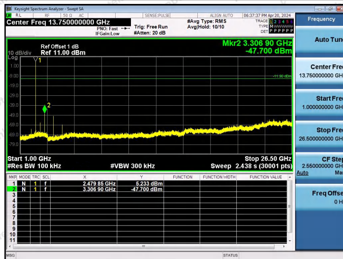
BLE_2M-Ant2-2480-1000~26500-PASS
