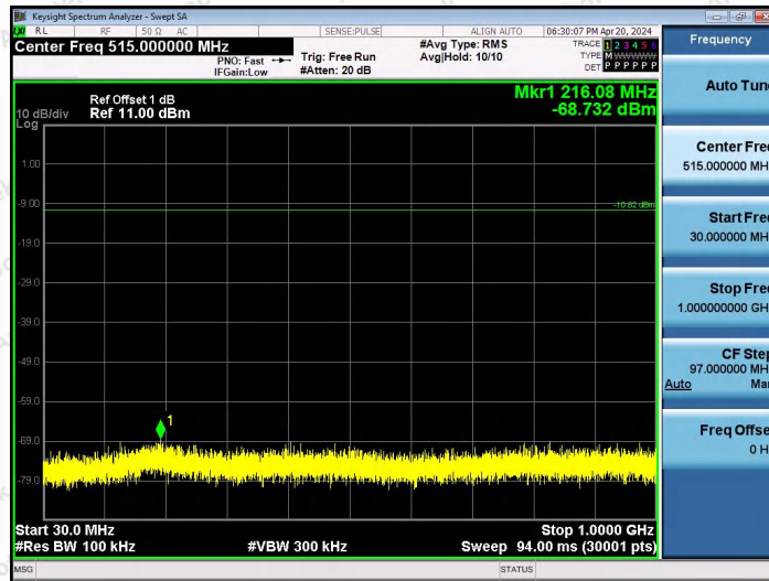
BLE_1M-Ant2-2480-30~1000-PASS
