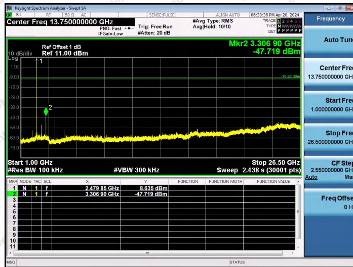
BLE_1M-Ant2-2480-1000~26500-PASS
