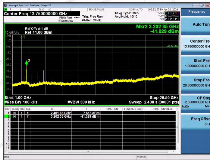
BLE_2M-Ant2-2402-1000~26500-PASS
