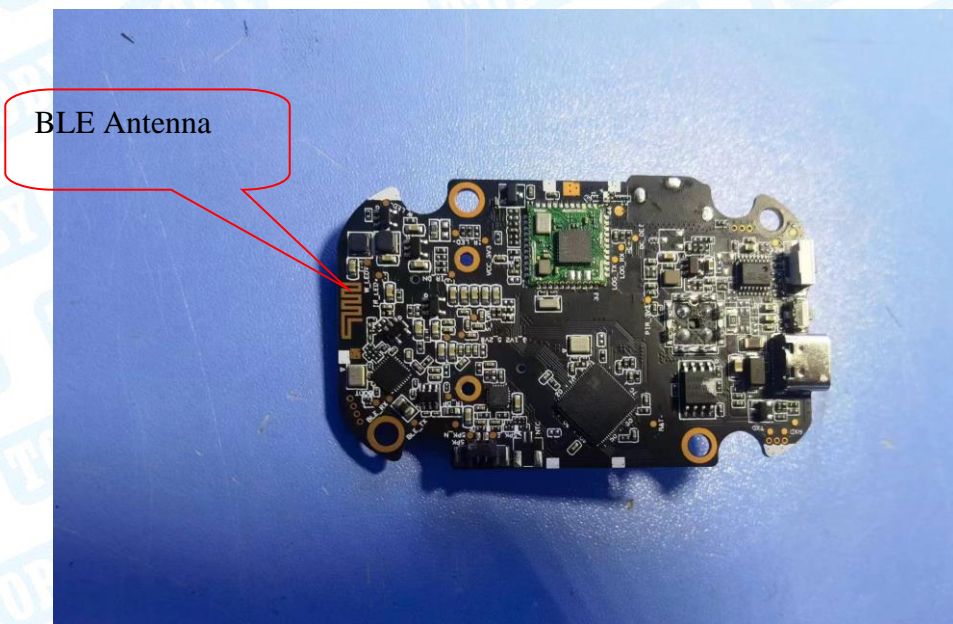
Photo 14 Appearance of PCB
