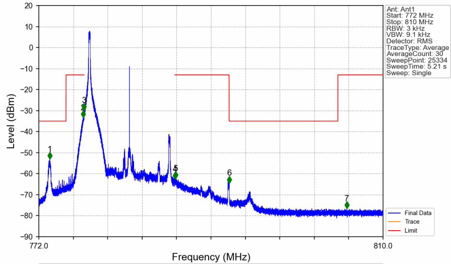
Band13_10MHz_16QAM_MCH_782MHz_RB_1_0_NTNV
