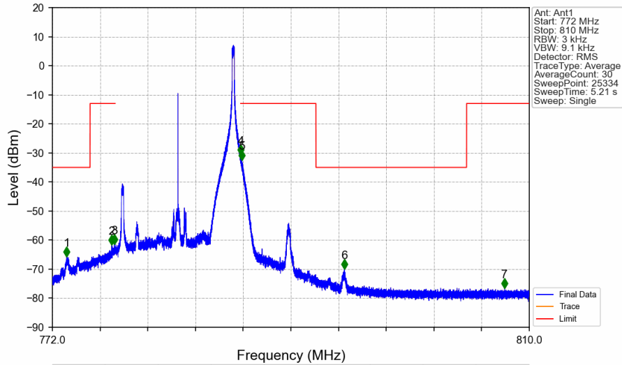
Band13_10MHz_16QAM_MCH_782MHz_RB_1_49_NTNV
