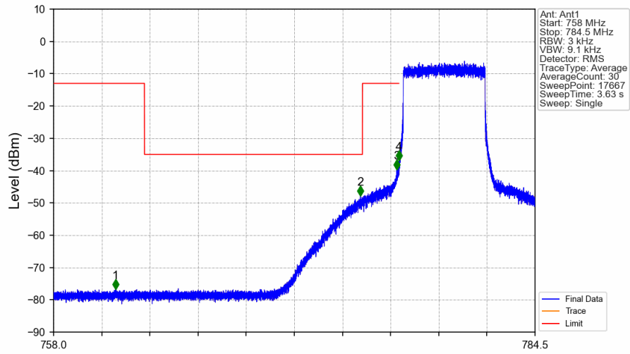
Band13_5MHz_16QAM_LCH_779.5MHz_RB_25_0_NTNV
