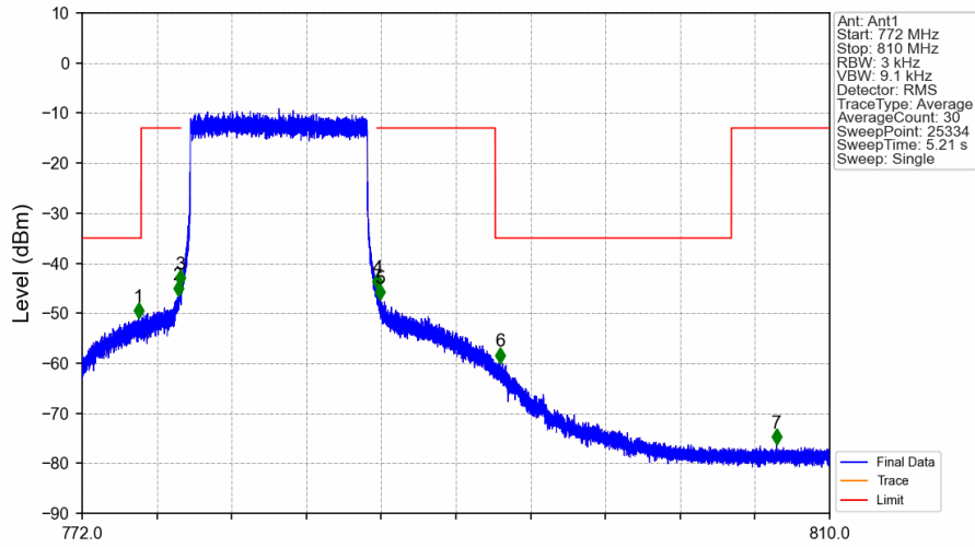
Band13_10MHz_16QAM_MCH_782MHz_RB_50_0_NTNV
