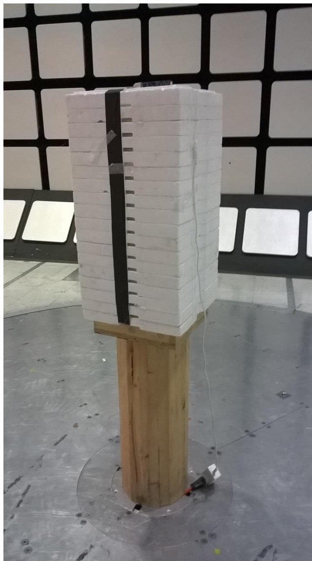
Figure 2 - Radiated Emissions Test Setup, 1 - 25 GHz
