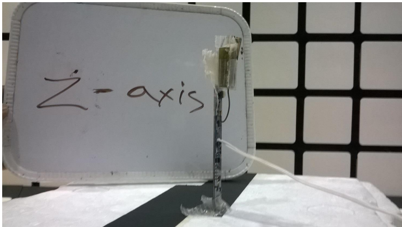
Figure 5 - Radiated Emissions Test Setup, Z-axis
