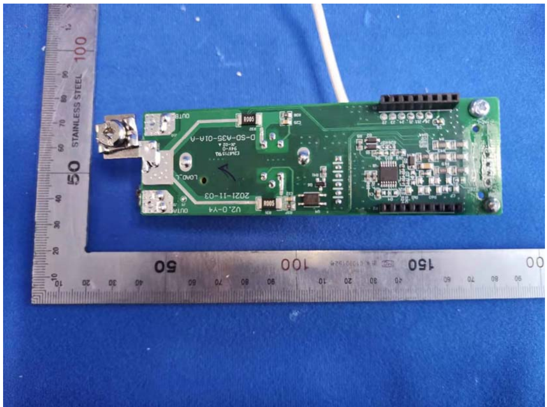
FIGURE 10 QO FORWARD PHASE DIMMER, PIGTAIL (M/N: GPM-Q2FPD05-21) MAINBOARD BACK
