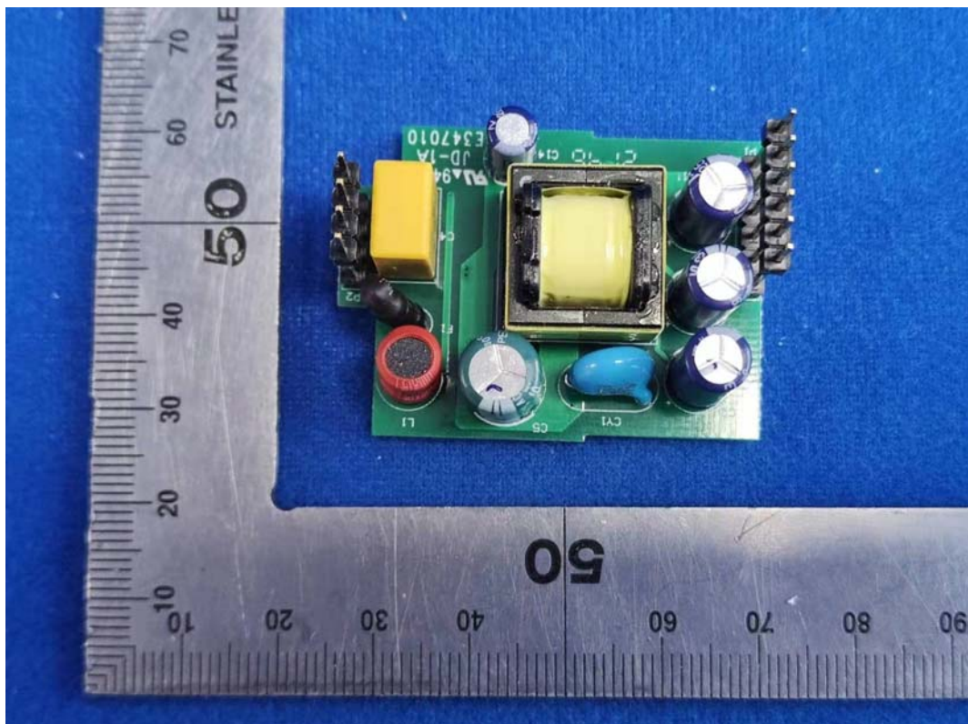
FIGURE 13 QO FORWARD PHASE DIMMER, PIGTAIL (M/N: GPM-Q2FPD05-21) CONTROL BOARD BACK
