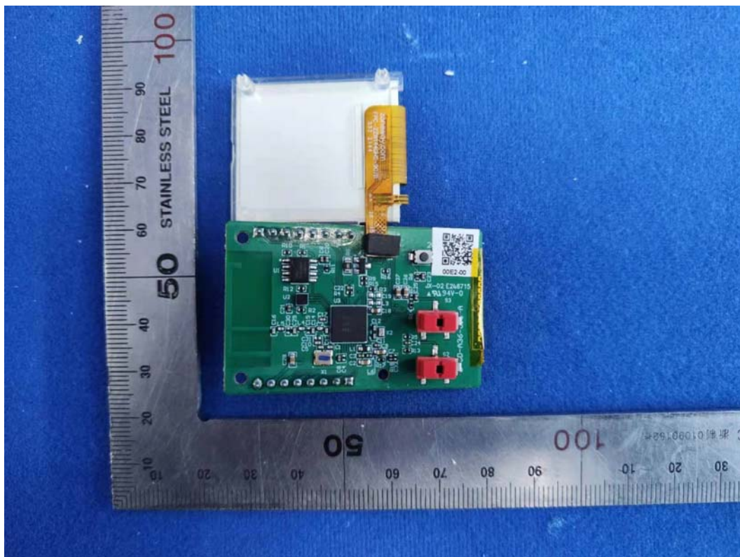
FIGURE 14 QO FORWARD PHASE DIMMER, PIGTAIL (M/N: GPM-Q2FPD05-21) RF BOARD FRONT
