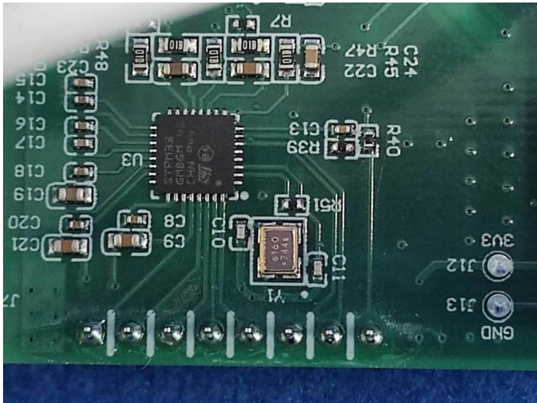
FIGURE 11 QO FORWARD PHASE DIMMER, PIGTAIL (M/N: GPM-Q2FPD05-21) CHIP & CRYSTAL ON MAINBOARD
