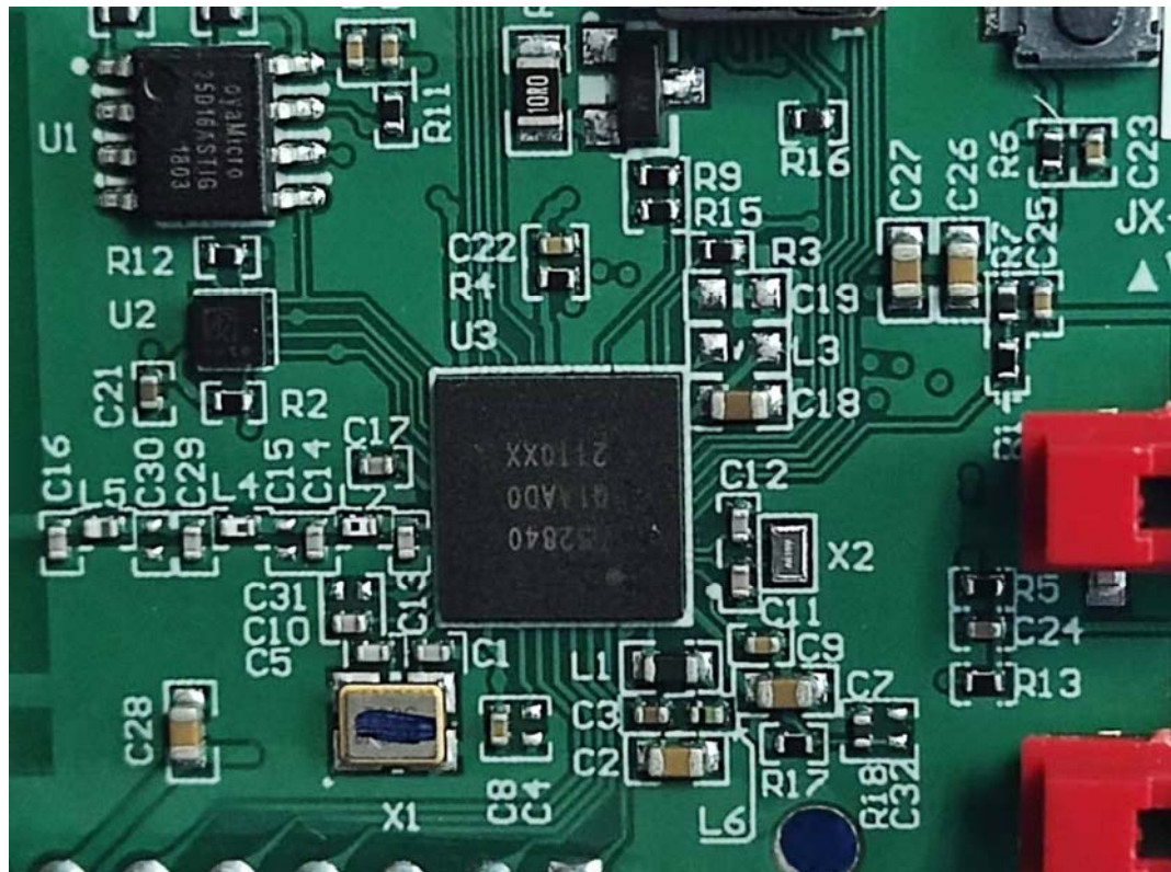
FIGURE 16 QO FORWARD PHASE DIMMER, PIGTAIL (M/N: GPM-Q2FPD05-21) CHIP & CRYSTAL ON RF BOARD
