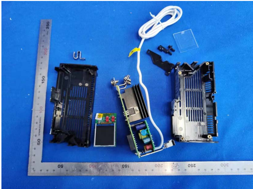
FIGURE 8 QO FORWARD PHASE DIMMER, PIGTAIL (M/N: GPM-Q2FPD05-21) COVER REMOVE
