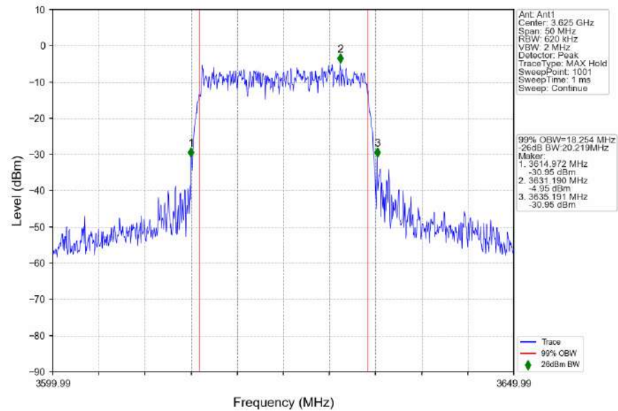
n48_30kHz_SISO_NTNV_20MHz_CP-OFDM_64_QAM_3624.99MHz_Outer_Full
