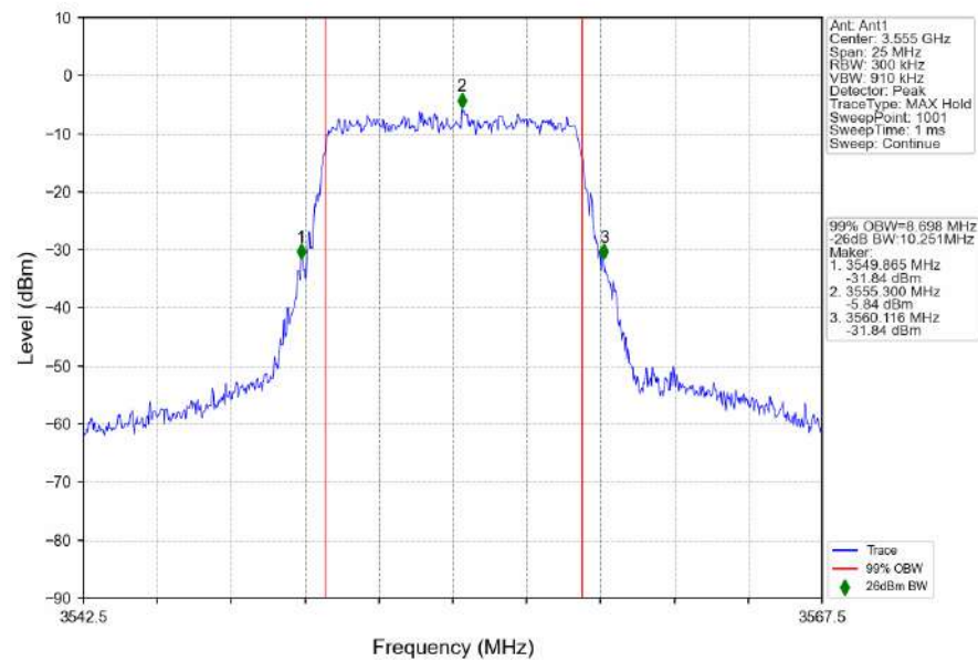
n48_30kHz_SISO_NTNV_10MHz_CP-OFDM_256_QAM_3555MHz_Outer_Full
