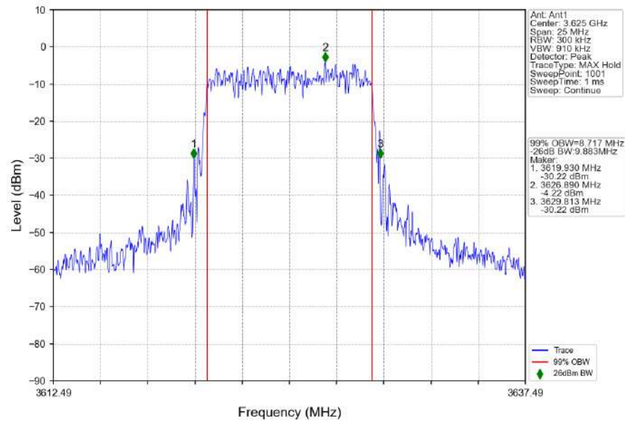
n48_30kHz_SISO_NTNV_10MHz_CP-OFDM_QPSK_3624.99MHz_Outer_Full
