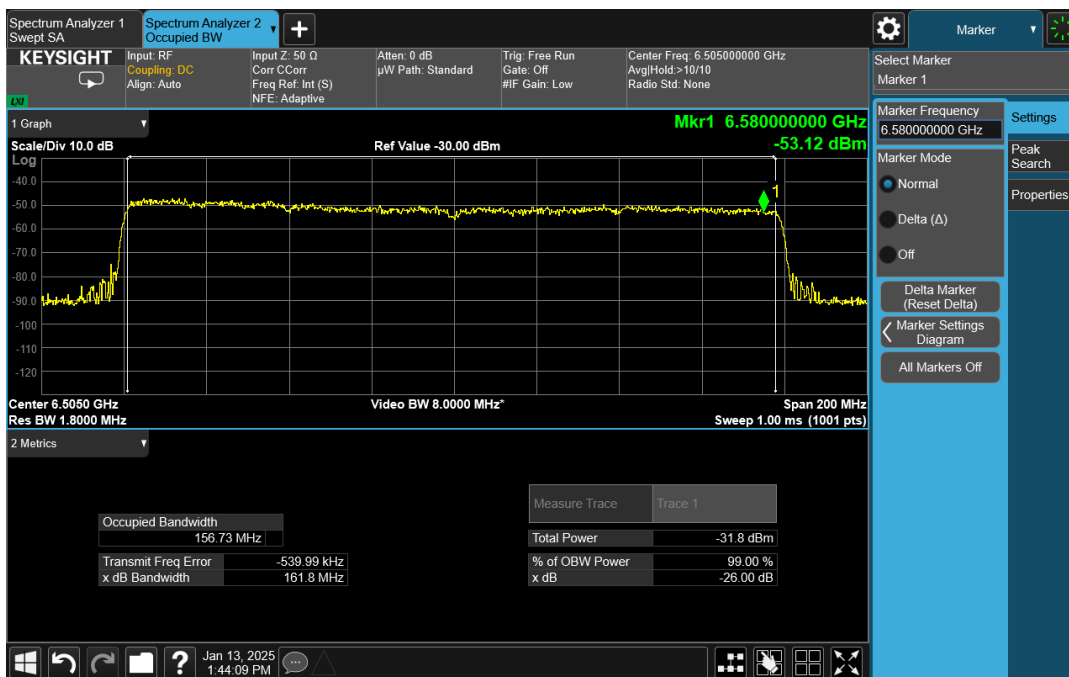
Plot 3: AWGN Signal BW 160 MHz
