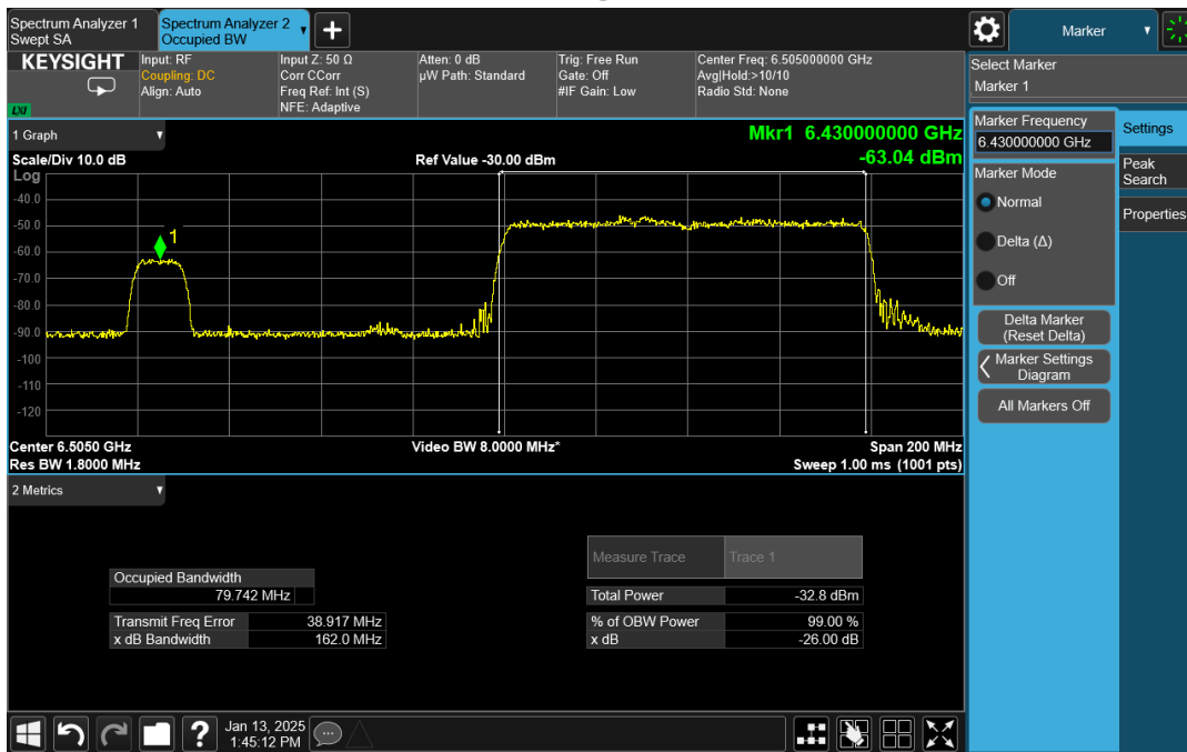
Plot 4: AWGN Signal BW Reduction 160 MHz
