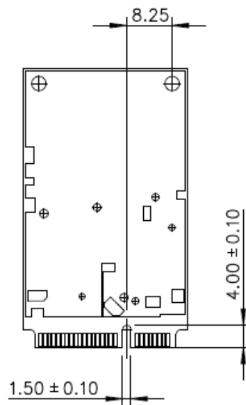
Figure 2. PCB dimension(Bottom view)
