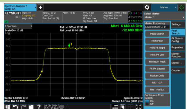
Channel 147 (6685MHz)
