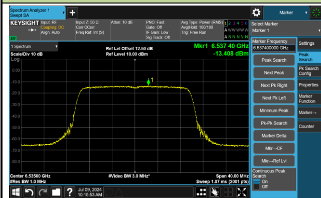
Channel 117 (6535MHz)
