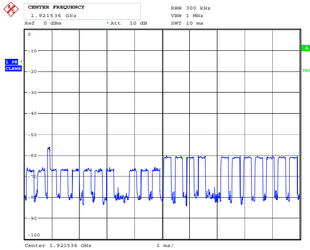
EUT Transmits on Free TRANSMIT Slot, BEFORE
