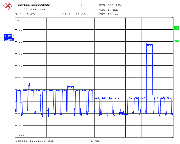
EUT Transmits on Free RECEIVE Slot, AFTER
