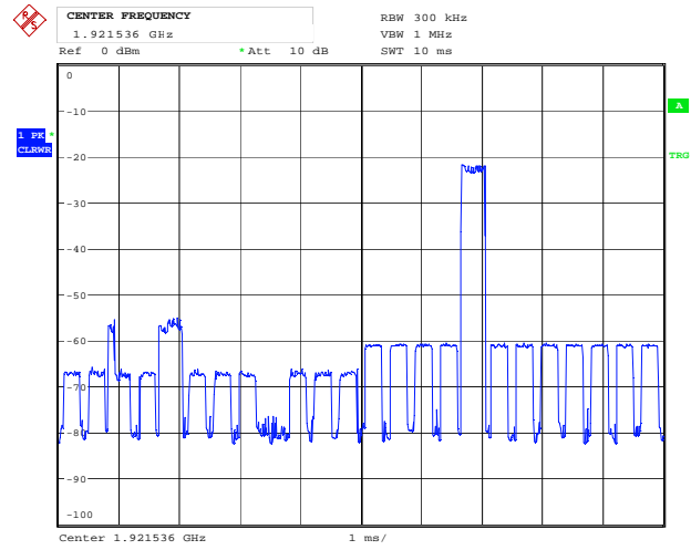
EUT Transmits on Free TRANSMIT Slot, AFTER
