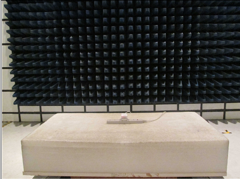
Radiated Emission Test (Frequency below 1GHz)
