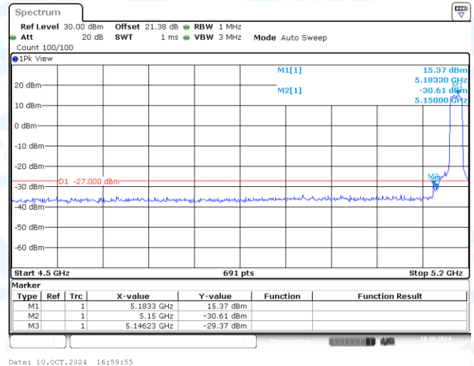
11N20MIMO-Ant2-5180-PASS
