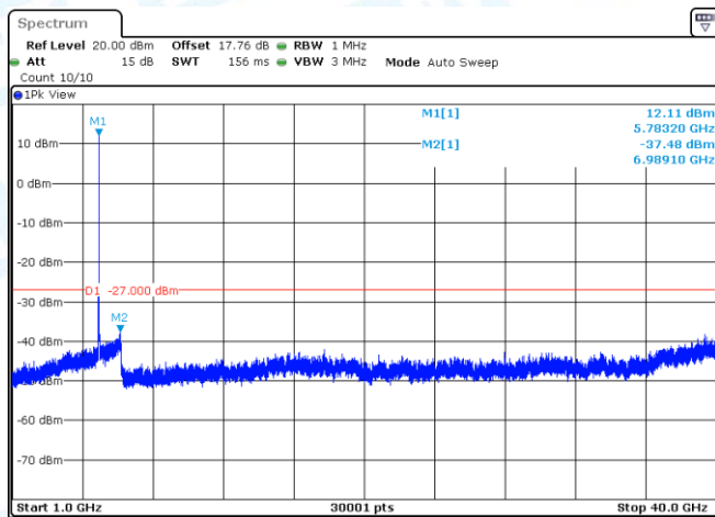
11A-CDD-Ant2-5785-1000~40000-PASS
