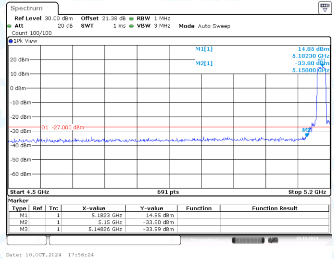
11AC20MIMO-Ant2-5180-PASS
