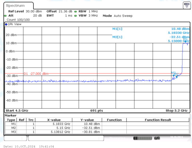
11AC40MIMO-Ant2-5190-PASS
