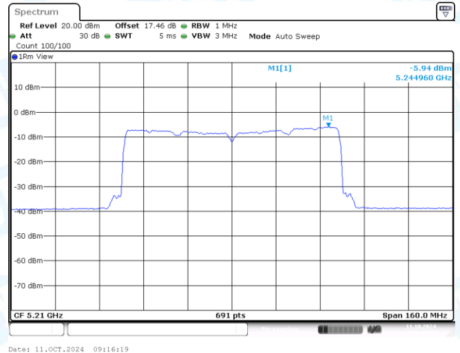
11AX80MIMO-Ant2-5210-PASS
