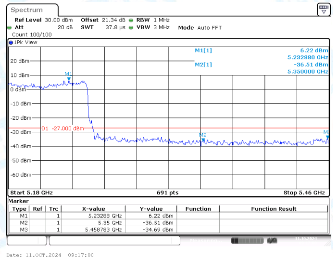
11AX80MIMO-Ant2-5210-PASS
