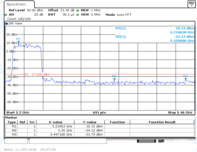
11AX40MIMO-Ant2-5230-PASS
