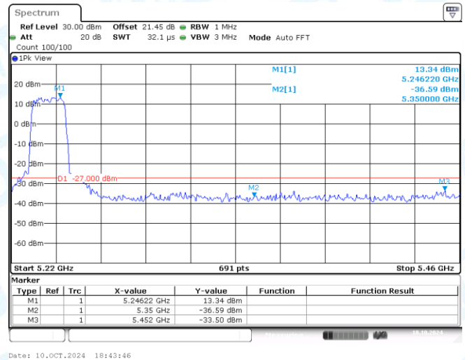
11AC20MIMO-Ant2-5240-PASS
