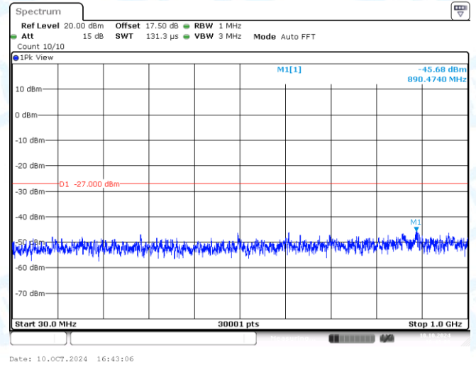
11A-CDD-Ant2-5180-30~1000-PASS
