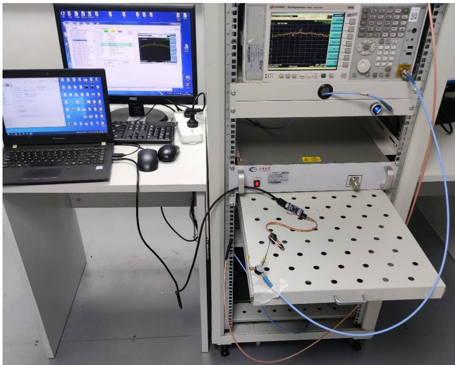
Conducted Test
