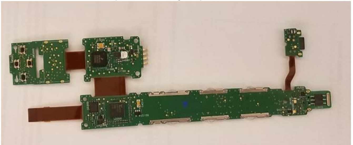
ADX2 Circuit Board Bottom (with shields in place)
