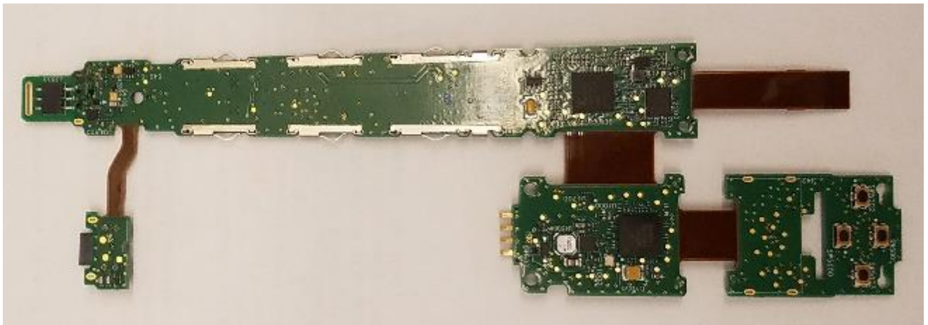
Shure ADX2 Circuit Board Bottom
