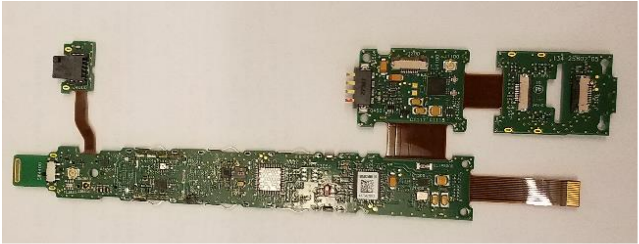
Photos: Shure ADX2 Circuit Board Top (shields removed)
