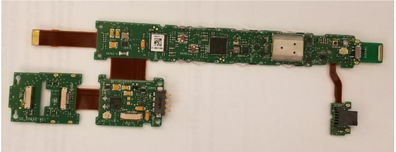
ADX2 Circuit Board Top (with shields in place)
