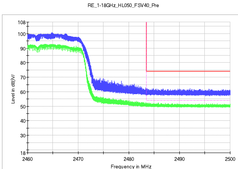
Figure 14: Radiated Band-Edge, TM9, V
