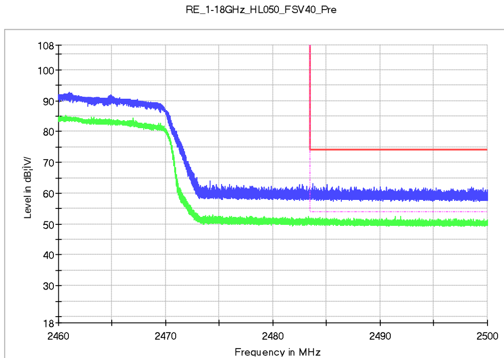
Figure 17: Radiated Band-Edge, TM12, H
