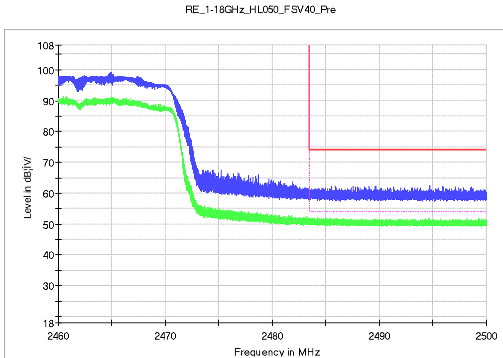
Figure 13: Radiated Band-Edge, TM9, H
