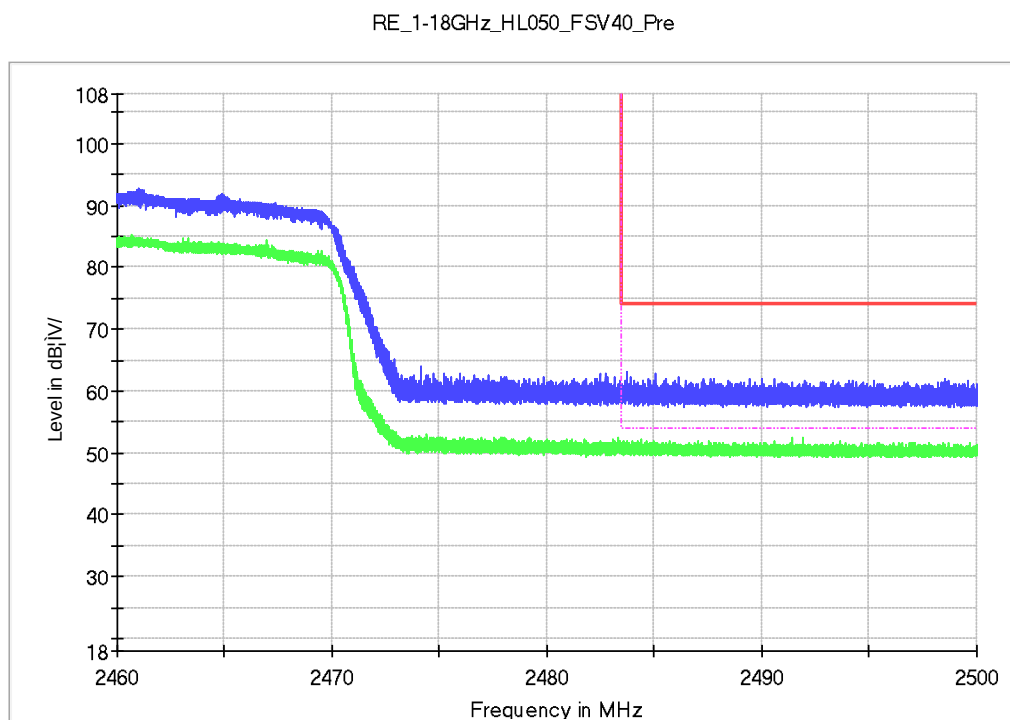
Figure 18: Radiated Band-Edge, TM12, V
