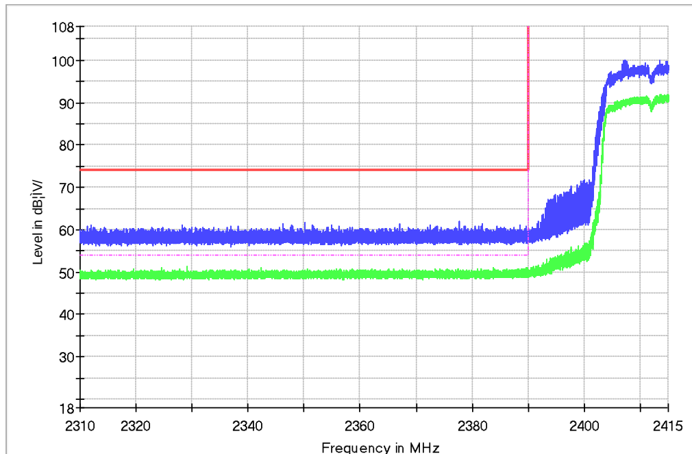
Figure 7: Radiated Band-Edge, TM4, H
