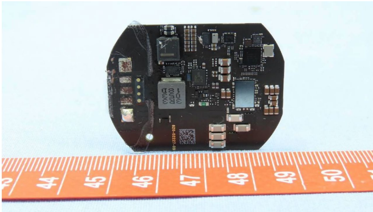
C223 PCB (MagSafe iPhones – 360 kHz) – Bottom View
