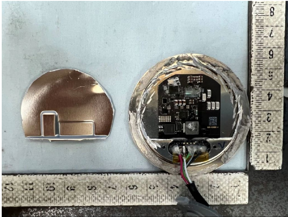
C223 Coil Antenna (MagSafe iPhones – 360 kHz) – Bottom View
