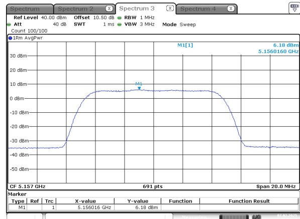
10M_5157MHz
