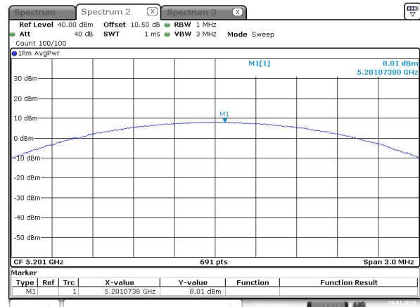
1.4M_5201MHz
