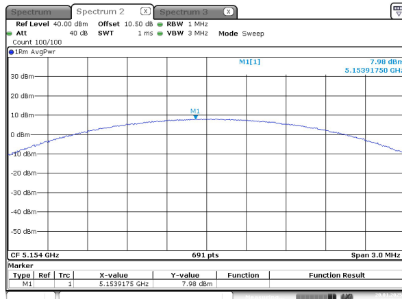
1.4M_5154MHz
