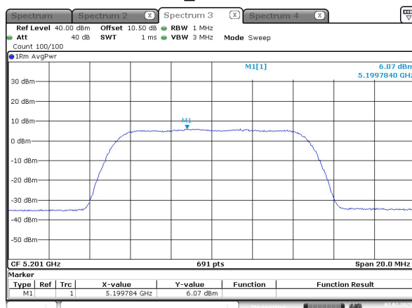
10M_5201MHz
