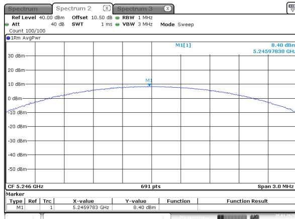
1.4M_5246MHz
