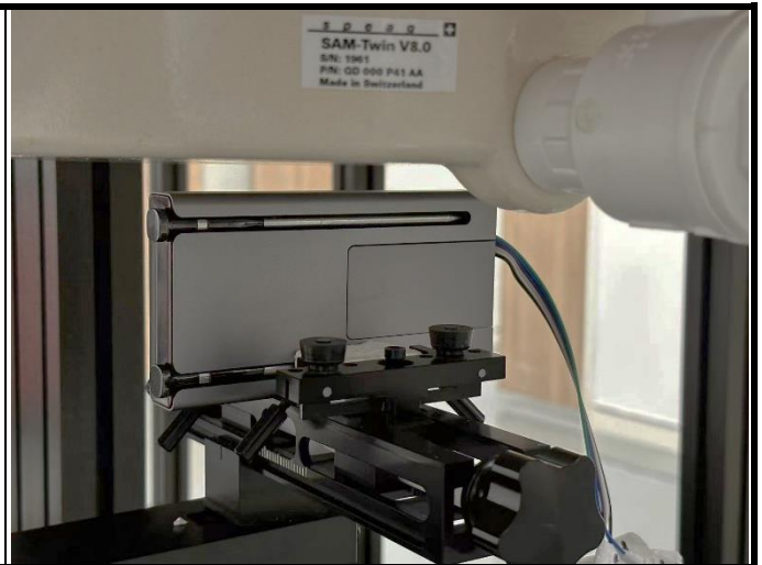
Left Side of EUT + Probe with 10mm Gap
