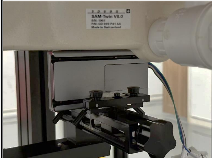
Left Side of EUT + Probe with 0 cm Gap
