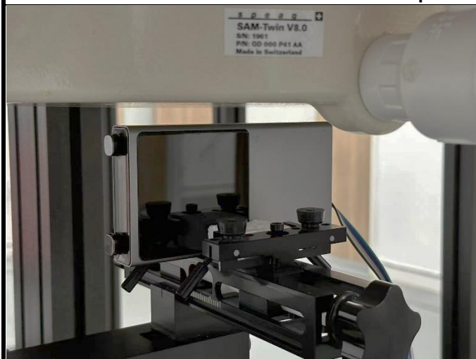
Right Side of EUT + Probe with 10mm Gap
