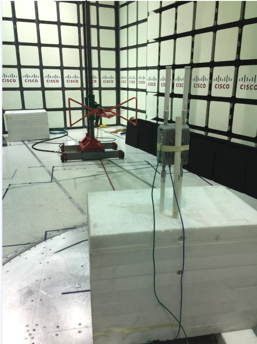
Radiated Emissions setup 30MHz – 1GHz
