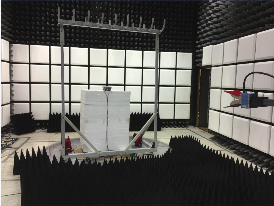
Radiated Emissions setup above 1GHz
