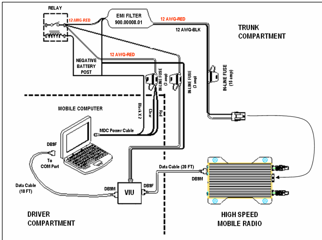
Figure 13: VIU Connections
