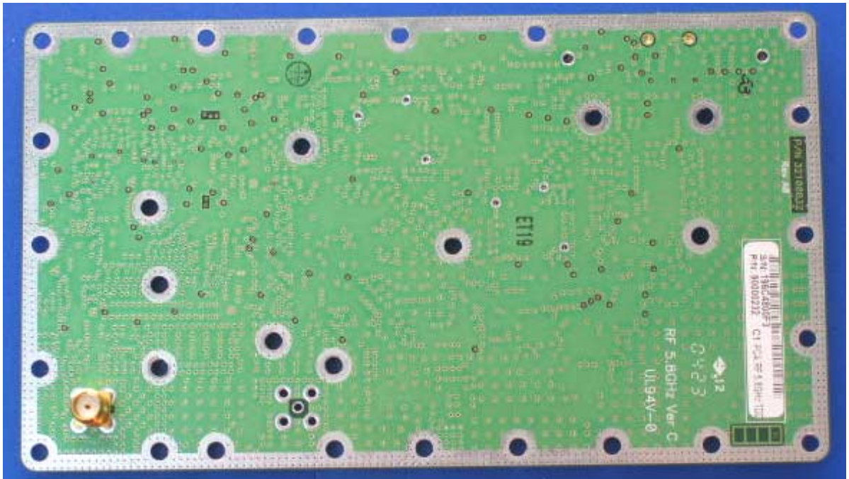
Photograph No.9 “SPR 5.8GHz TDD Ext”, RF module second side view
