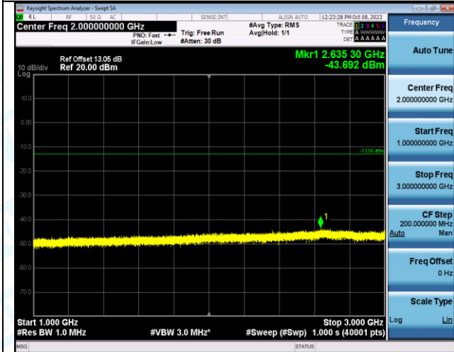
Band2_15MHz_QPSK_19125_1RB#74_1000~3000_1000~3000
