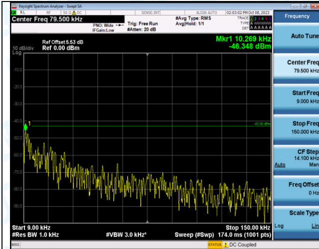
Band2_20MHz_QPSK_18900_1RB#99_0.009~0.15_0.009 ~0.15
