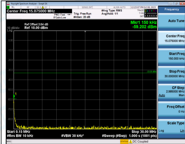
Band2_15MHz_QPSK_19125_1RB#74_0.15~30_0.15~30
