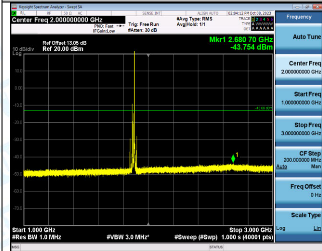
Band2_20MHz_16QAM_18900_1RB#99_1000~3000_100
