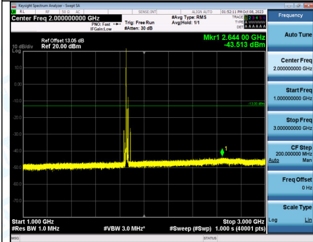
Band2_20MHz_16QAM_18700_1RB#0_1000~3000_1000~3000
