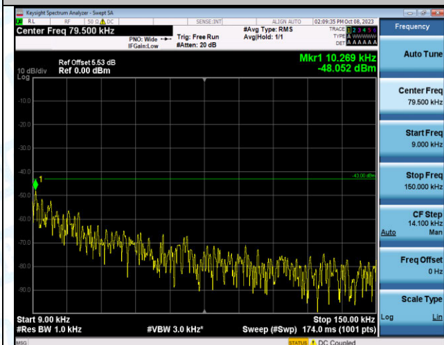
Band2_20MHz_QPSK_19100_1RB#0_0.009~0.15_0.009~
