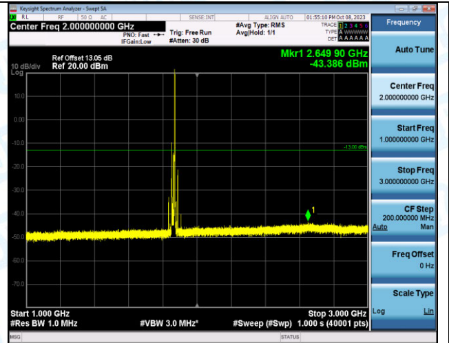
Band2_20MHz_QPSK_18700_1RB#99_1000~3000_1000~3000 ~3000
