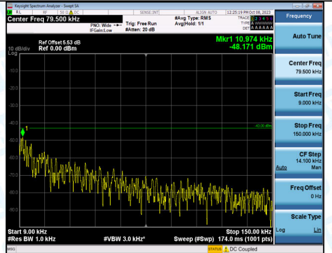
Band2_15MHz_QPSK_18675_75RB#0_0.009~0.15_0.009~0.15
