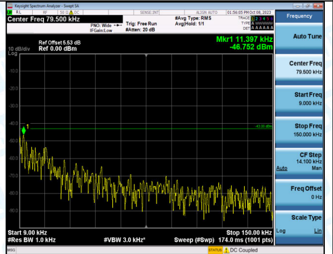
Band2_20MHz_16QAM_18700_1RB#99_0.009~0.15_0.009~0.15 9~0.15
