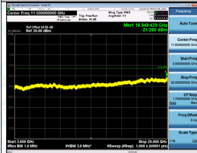
Band2_20MHz_QPSK_18900_1RB#99_3000~20000_300 0~20000
