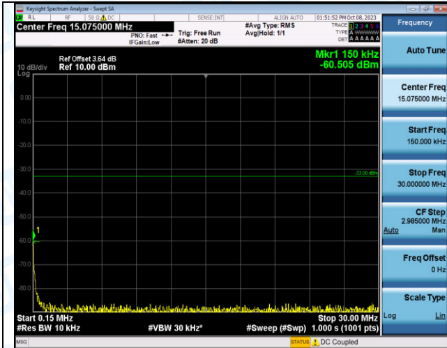
Band2_20MHz_16QAM_18700_1RB#0_0.15~30_0.15~30
