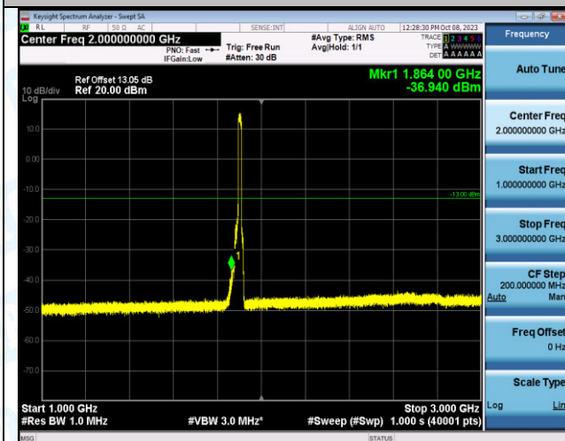
Band2_15MHz_QPSK_19125_75RB#0_1000~3000_1000 ~3000
