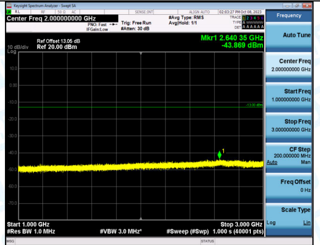
Band2_20MHz_QPSK_18900_1RB#99_1000~3000_1000 ~3000
