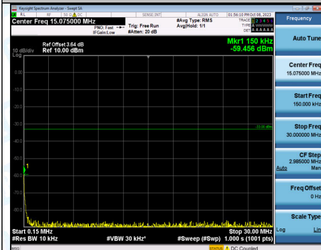
Band2_20MHz_16QAM_18700_1RB#99_0.15~30_0.15~30 0
