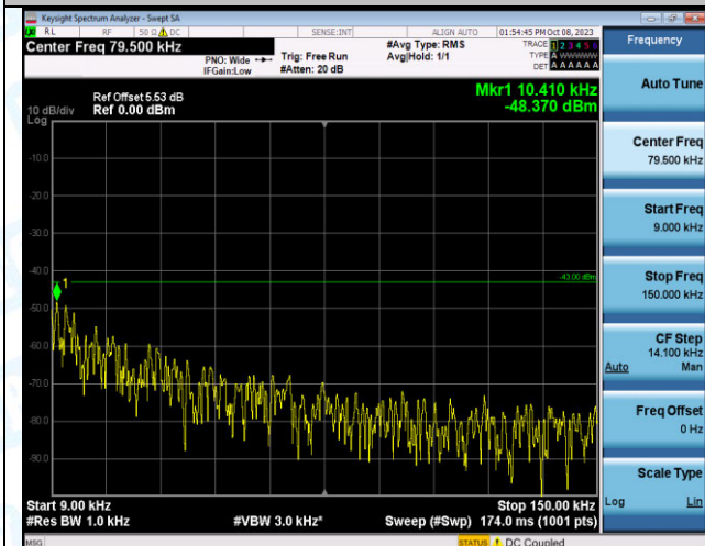
Band2_20MHz_QPSK_18700_1RB#99_0.009~0.15_0.009~0.15
