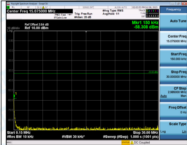
Band2_20MHz_16QAM_18900_1RB#99_0.15~30_0.15~3
