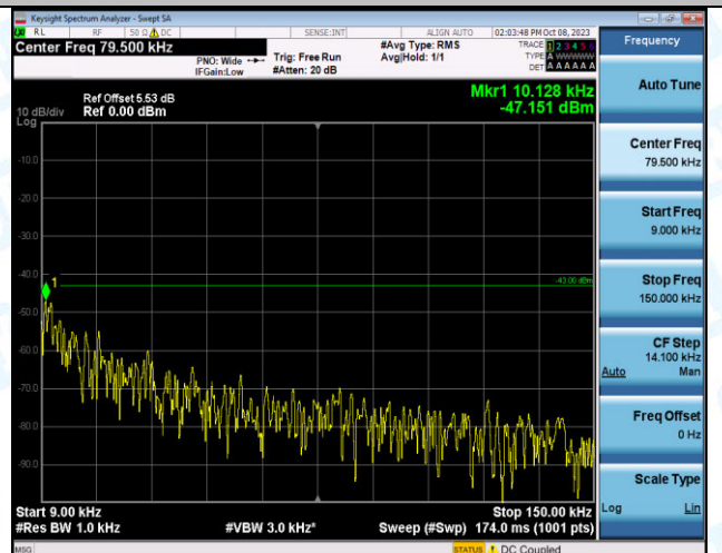
Band2_20MHz_16QAM_18900_1RB#99_0.009~0.15_0.00 9~0.15
