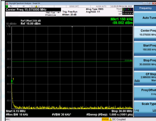
Band2_15MHz_QPSK_18675_75RB#0_0.15~30_0.15~30
