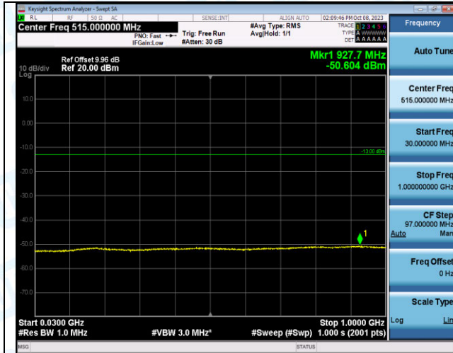
Band2_20MHz_QPSK_19100_1RB#0_30~1000_30~1000
