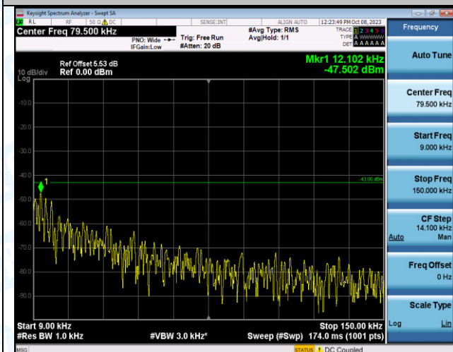
Band2_15MHz_16QAM_19125_1RB#74_0.009~0.15_0.009~0.15 9~0.15
