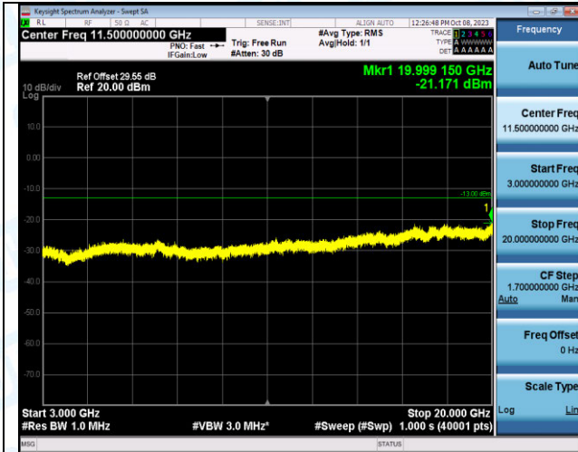
Band2_15MHz_QPSK_18900_75RB#0_3000~20000_300 0~20000
