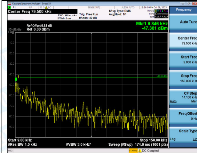
Band2_15MHz_QPSK_18900_75RB#0_0.009~0.15_0.009 ~0.15
