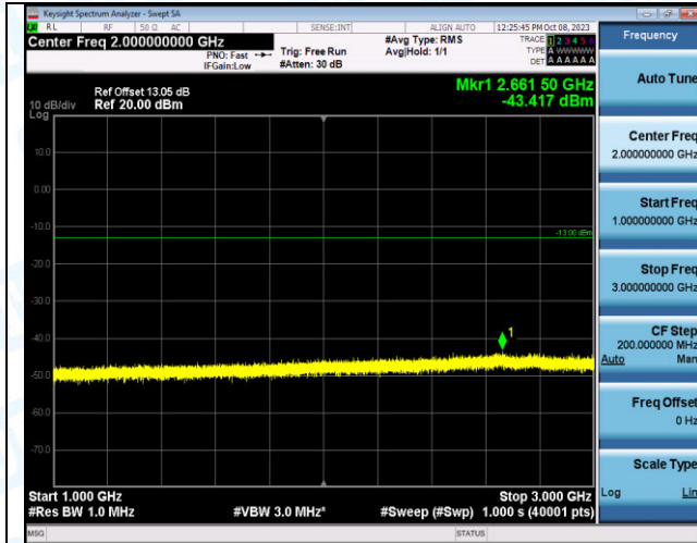
Band2_15MHz_QPSK_18675_75RB#0_1000~3000_1000 ~3000
