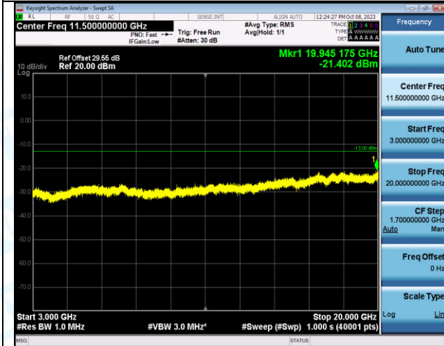
Band2_15MHz_16QAM_19125_1RB#74_3000~20000_3000~20000
