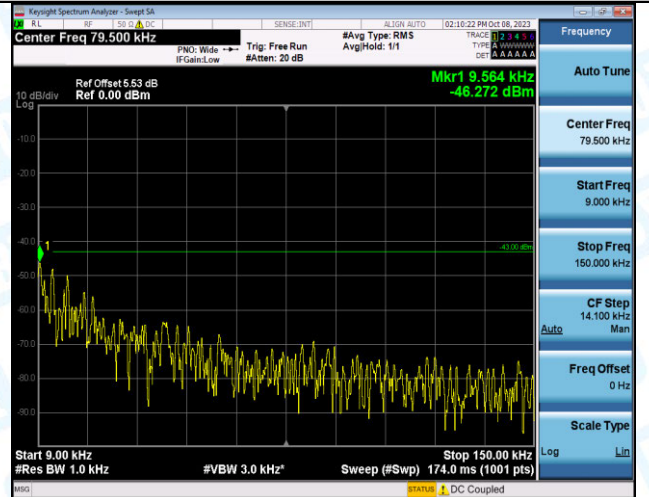
Band2_20MHz_16QAM_19100_1RB#0_0.009~0.15_0.009~0.15
