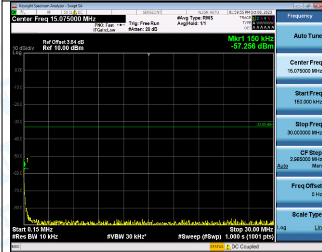
Band2_20MHz_16QAM_18900_1RB#0_0.15~30_0.15~30
