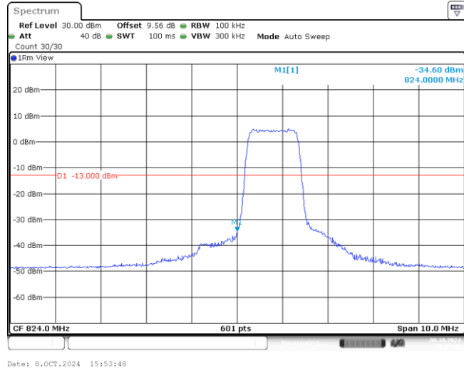
Band26-5MHz-16QAM-26815-6-0-Low--34.60-PASS
