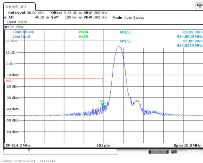
Band26-10MHz-QPSK-26740-1-0-Low--39.39,-36.80-PASS
