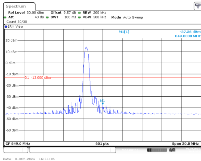
Band26-10MHz-QPSK-26990-1-0-High--37.36-PASS
