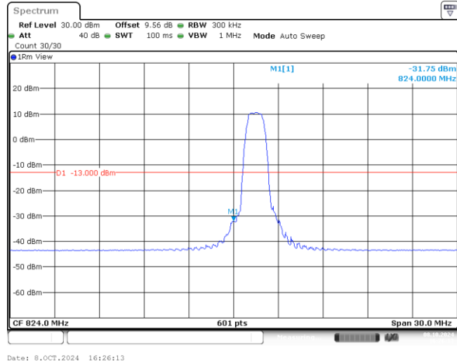
Band26-15MHz-QPSK-26865-6-0-Low--31.75-PASS
