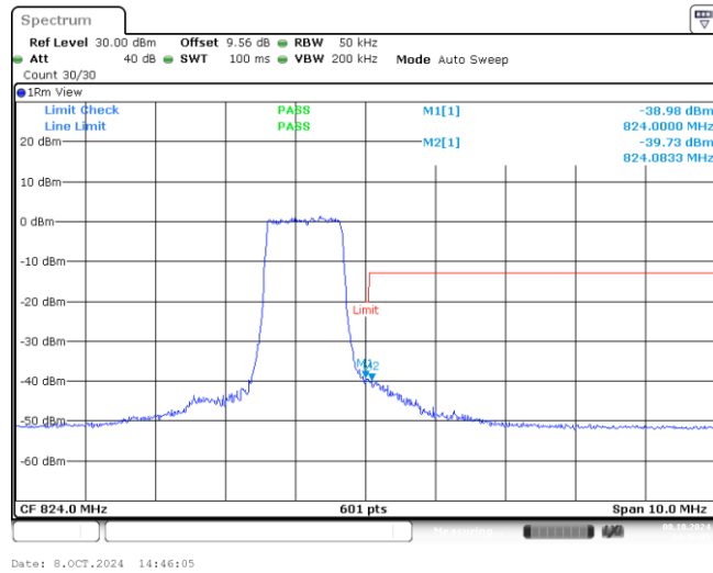
Band26-3MHz-QPSK-26775-6-0-High--38.98,-39.73-PASS
