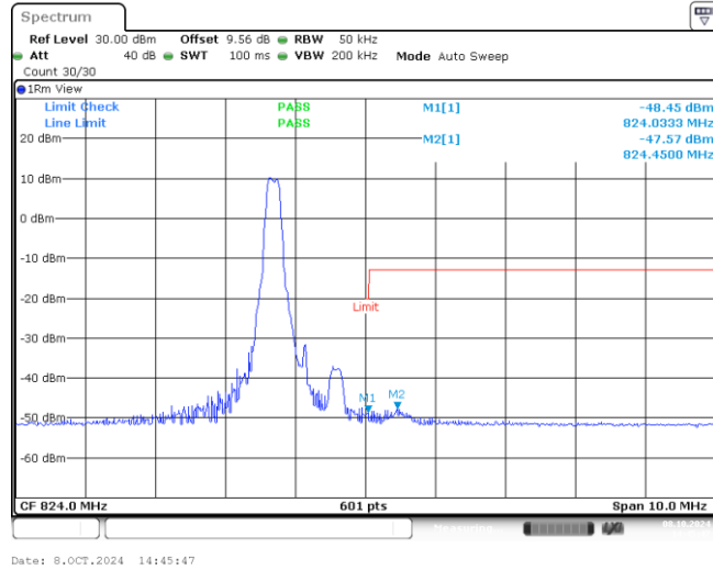
Band26-3MHz-QPSK-26775-1-0-High--48.45,-47.57-PASS
