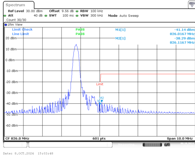
Band26-5MHz-QPSK-26785-1-0-High--41.14,-38.29-PASS
