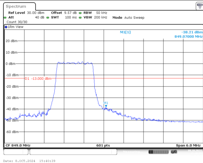
Band26-3MHz-QPSK-27025-6-0-High--38.21-PASS
