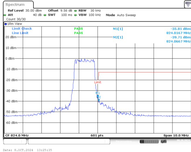
Band26-1.4MHz-QPSK-26783-6-0-High--35.81,-39.71-PASS
