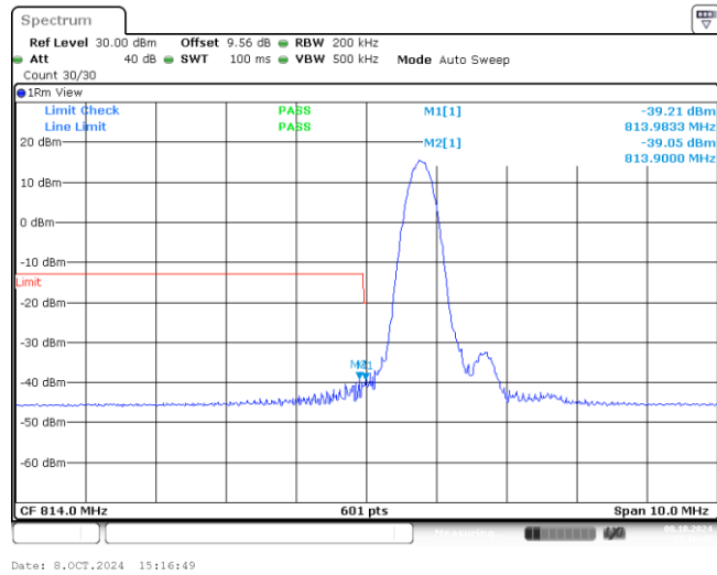
Band26-10MHz-16QAM-26740-1-0-Low--39.21,-39.05-PASS
