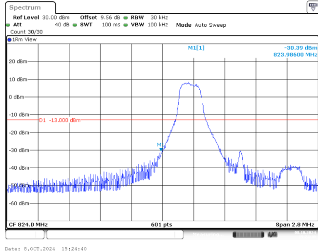
Band26-1.4MHz-16QAM-26797-1-0-Low--30.39-PASS
