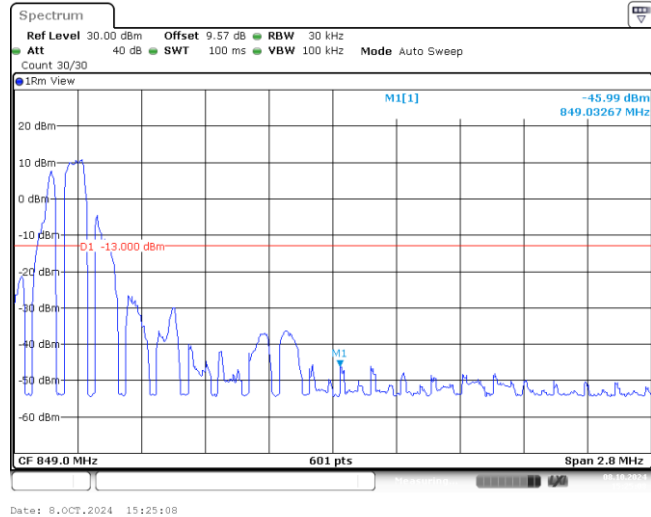
Band26-1.4MHz-QPSK-27033-1-0-High--45.99-PASS
