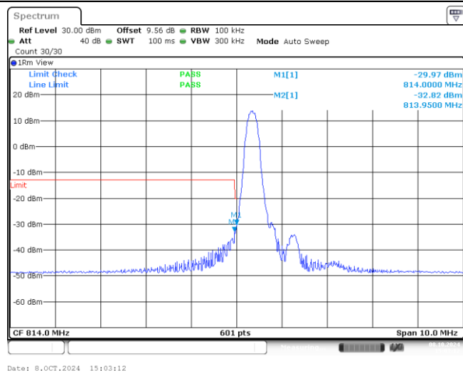
Band26-5MHz-QPSK-26715-1-0-Low--29.97,-32.82-PASS
