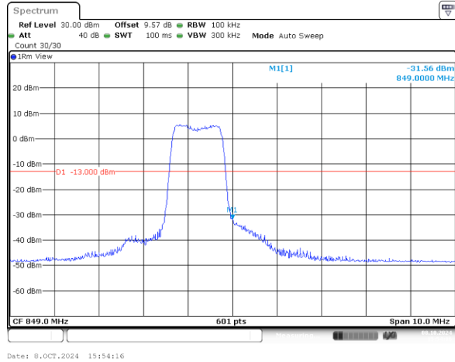
Band26-5MHz-QPSK-27015-6-0-High--31.56-PASS
