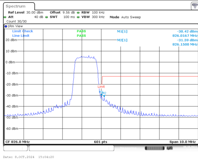
Band26-5MHz-QPSK-26785-6-0-High--30.42,-31.59-PASS
