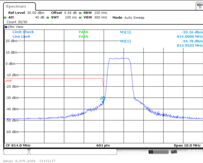
Band26-5MHz-16QAM-26715-6-0-Low--33.16,-34.78-PASS
