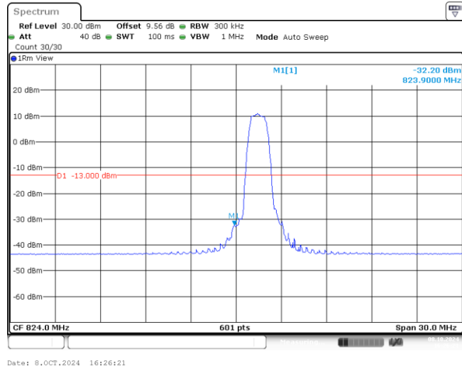
Band26-15MHz-16QAM-26865-6-0-Low--32.20-PASS
