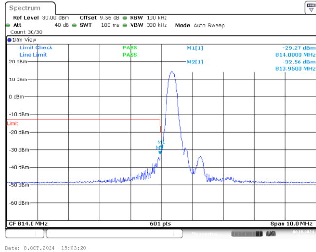
Band26-5MHz-16QAM-26715-1-0-Low--29.27,-32.56-PASS
