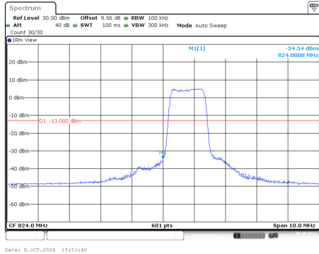
Band26-5MHz-QPSK-26815-6-0-Low--34.54-PASS
