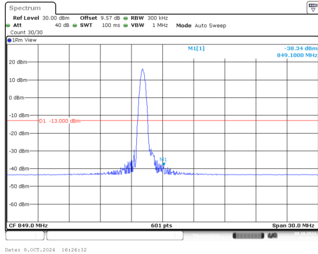
Band26-15MHz-QPSK-26965-1-0-High--38.34-PASS
