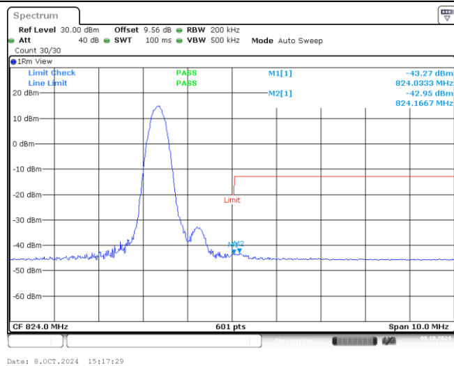
Band26-10MHz-16QAM-26740-1-0-High--43.27,-42.95-PASS
