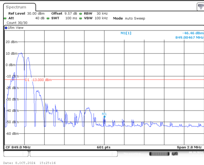
Band26-1.4MHz-16QAM-27033-1-0-High--46.46-PASS
