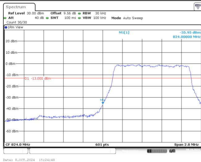
Band26-1.4MHz-QPSK-26797-6-0-Low--35.95-PASS
