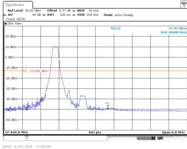
Band26-3MHz-QPSK-27025-1-0-High--47.84-PASS
