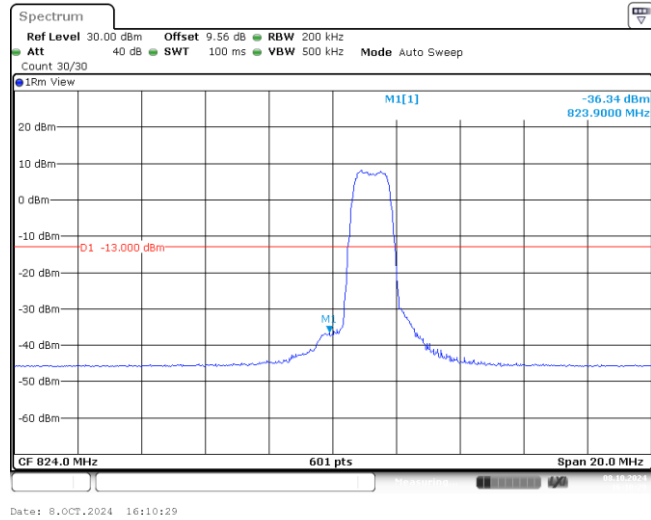
Band26-10MHz-QPSK-26840-6-0-Low--36.34-PASS
