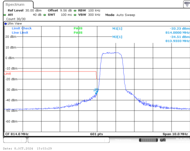
Band26-5MHz-QPSK-26715-6-0-Low--33.23,-34.51-PASS
