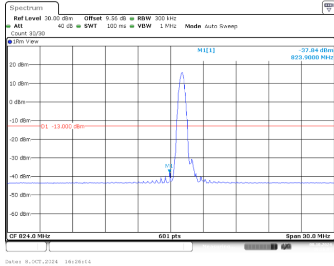
Band26-15MHz-16QAM-26865-1-0-Low--37.84-PASS
