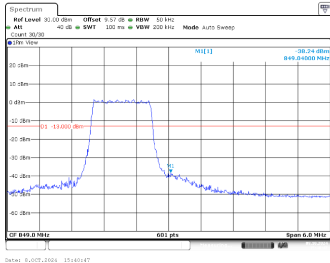
Band26-3MHz-16QAM-27025-6-0-High--38.24-PASS
