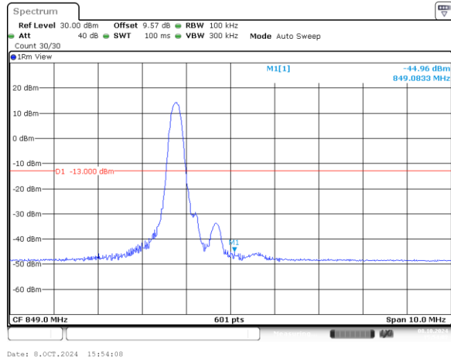
Band26-5MHz-16QAM-27015-1-0-High--44.96-PASS
