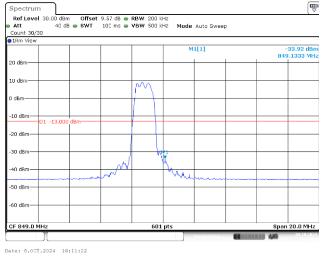
Band26-10MHz-QPSK-26990-6-0-High--33.92-PASS
