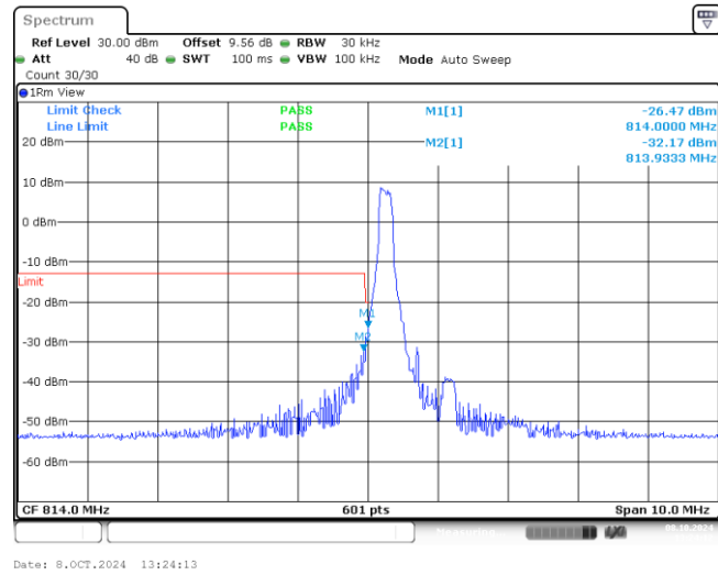
Band26-1.4MHz-QPSK-26697-1-0-Low--26.47,-32.17-PASS
