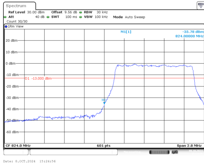
Band26-1.4MHz-16QAM-26797-6-0-Low--35.78-PASS
