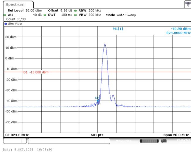
Band26-10MHz-QPSK-26840-1-0-Low--40.90-PASS
