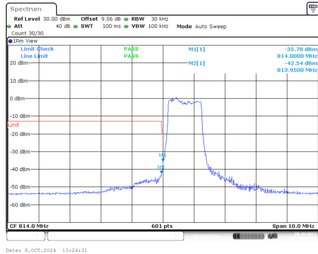
Band26-1.4MHz-QPSK-26697-6-0-Low--35.78,-42.54-PASS
