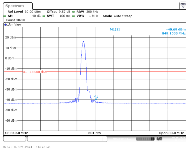
Band26-15MHz-16QAM-26965-1-0-High--40.69-PASS
