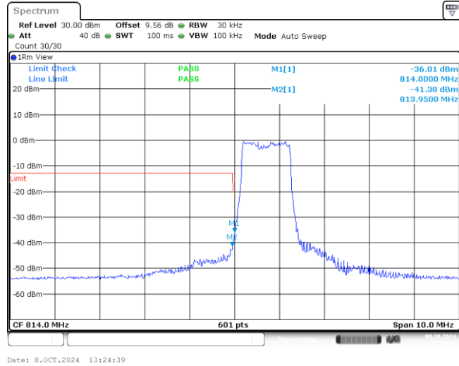
Band26-1.4MHz-16QAM-26697-6-0-Low--36.01,-41.38-PASS
