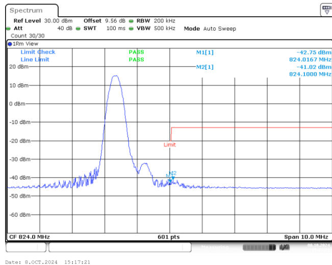
Band26-10MHz-QPSK-26740-1-0-High--42.75,-41.02-PASS
