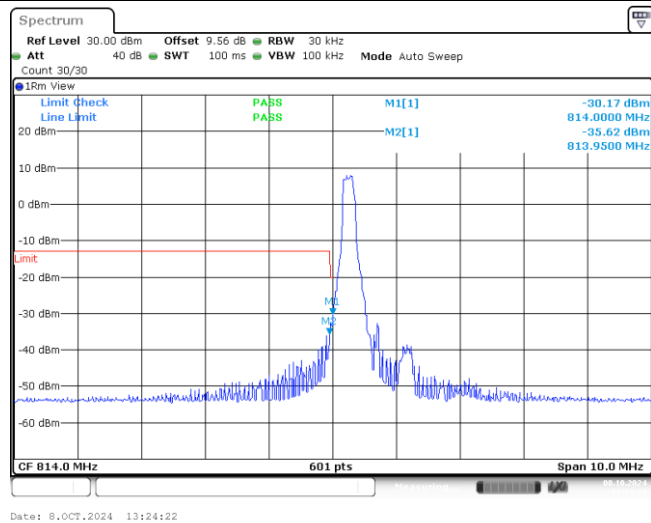
Band26-1.4MHz-16QAM-26697-1-0-Low--30.17,-35.62-PASS
