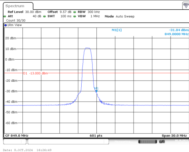
Band26-15MHz-QPSK-26965-6-0-High--31.04-PASS
