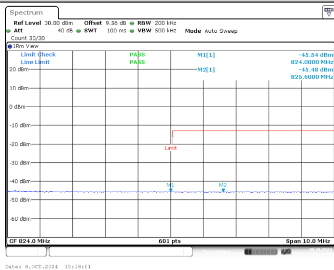
Band26-10MHz-QPSK-26740-6-0-Low--45.54,-45.48-PASS
