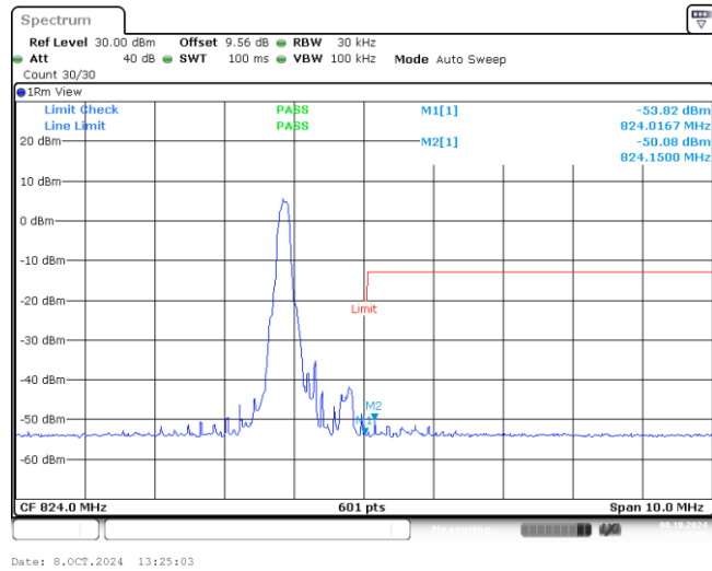
Band26-1.4MHz-16QAM-26783-1-0-High--53.82,-50.08-PASS
