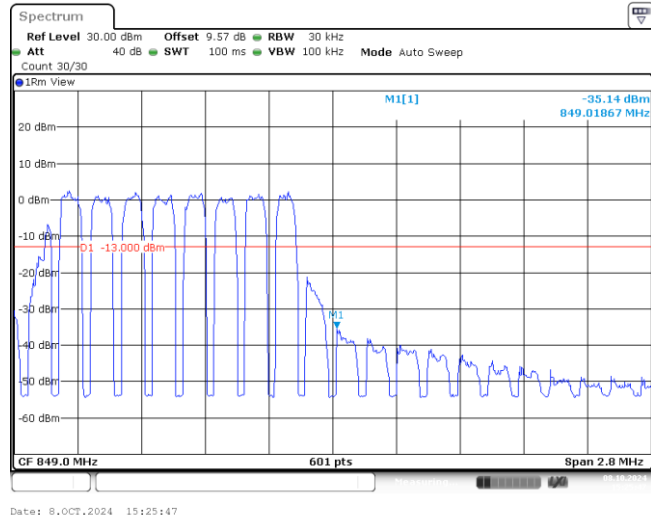
Band26-1.4MHz-QPSK-27033-6-0-High--35.14-PASS
