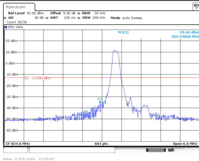
Band26-3MHz-QPSK-26805-1-0-Low--35.60-PASS
