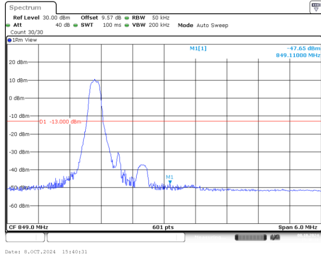
Band26-3MHz-16QAM-27025-1-0-High--47.65-PASS
