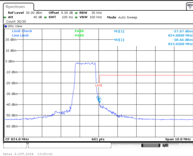
Band26-1.4MHz-16QAM-26783-6-0-High--37.07,-38.66-PASS
