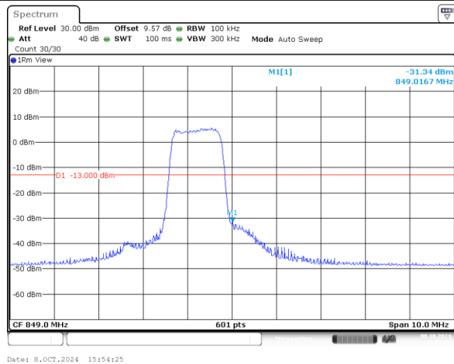
Band26-5MHz-16QAM-27015-6-0-High--31.34-PASS
