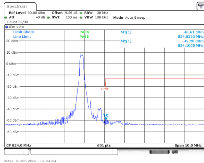
Band26-1.4MHz-QPSK-26783-1-0-High--48.61,-49.28-PASS
