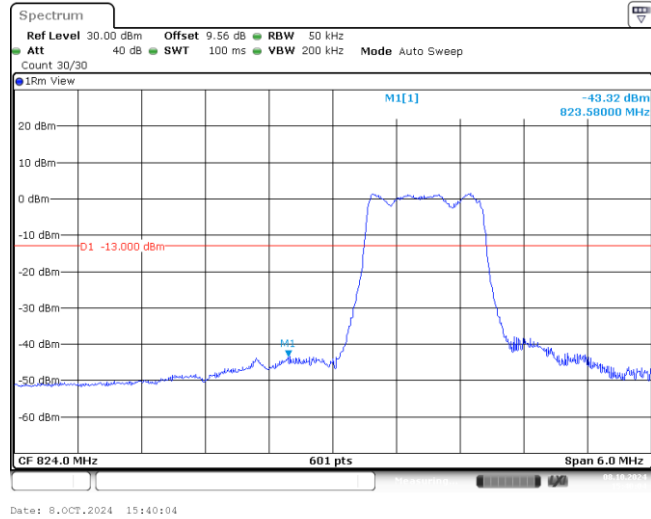
Band26-3MHz-QPSK-26805-6-0-Low--43.32-PASS
