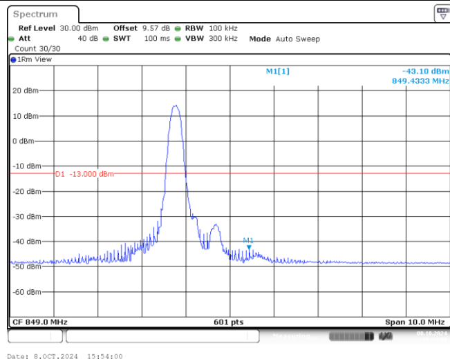
Band26-5MHz-QPSK-27015-1-0-High--43.10-PASS
