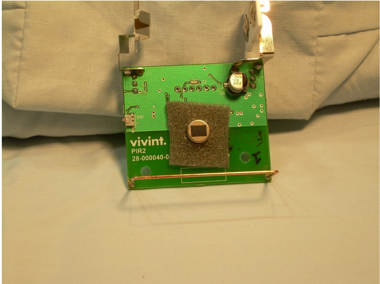
View of the Sensor/Antenna Side of the PCB
