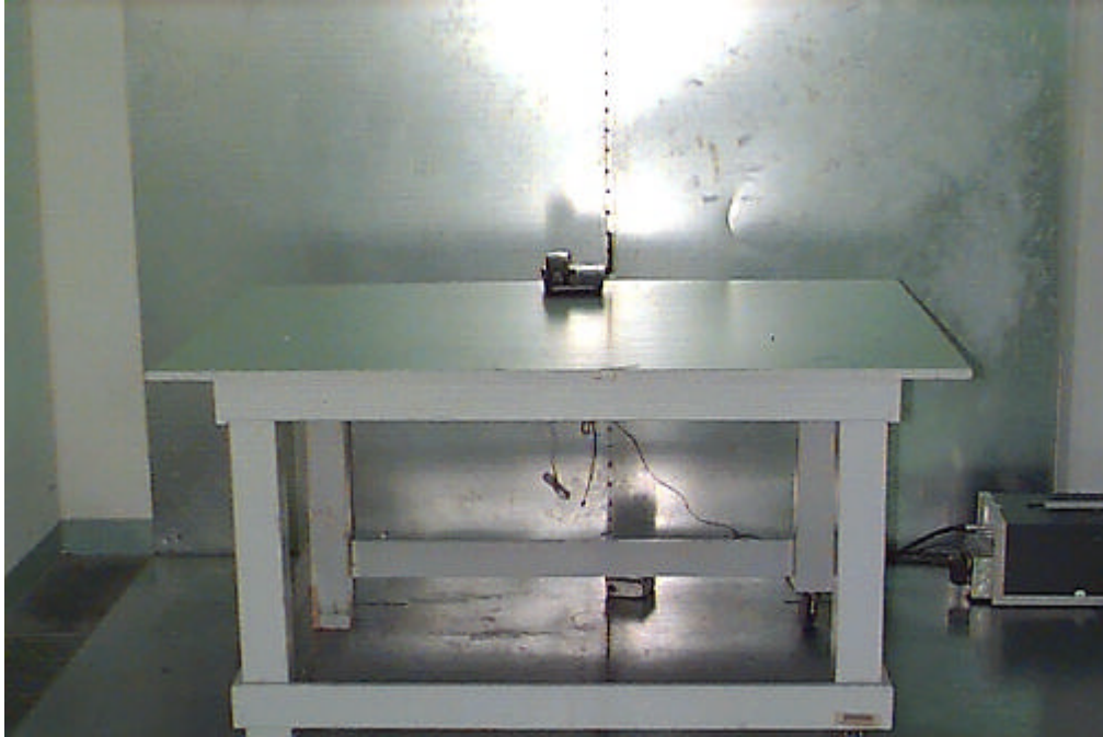
Conducted Emissions Test Set-up Front View
