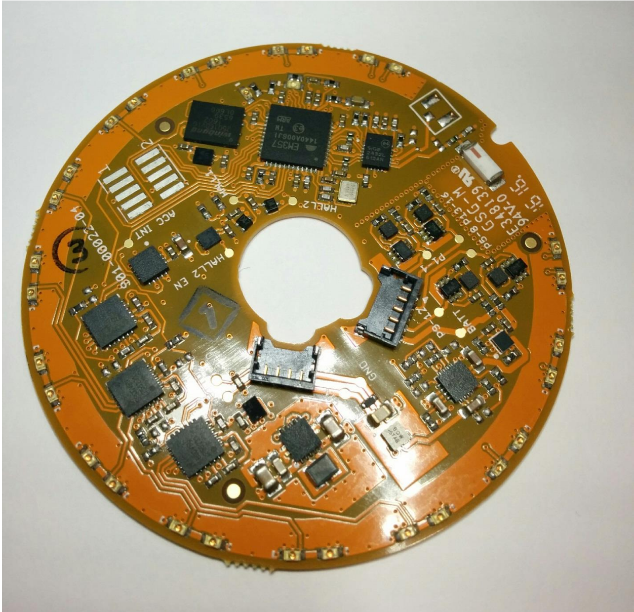
Figure 3: Internal view, PCB top
