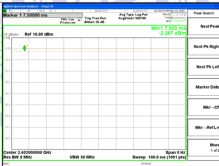
Duty_Cycle_NVNT_ANT1_1Mbps_2402
