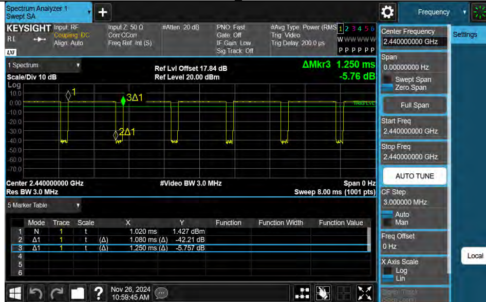
NTNV-BLE 2M-Ant1-2440
