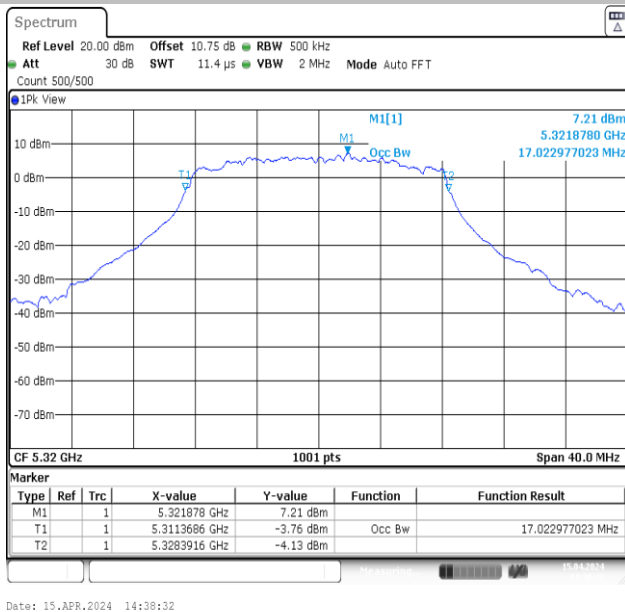
11A-Ant1-5320
