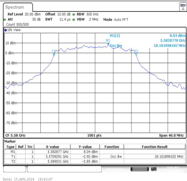
11N20MIMO-Ant2-5580
