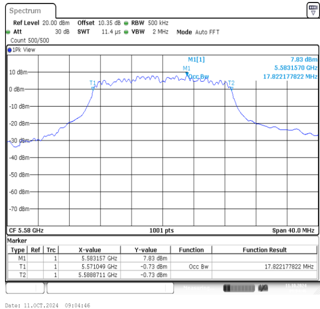
11AC20MIMO-Ant2-5580
