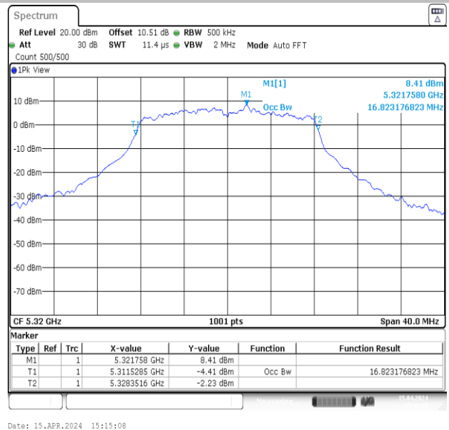
11A-Ant2-5320
