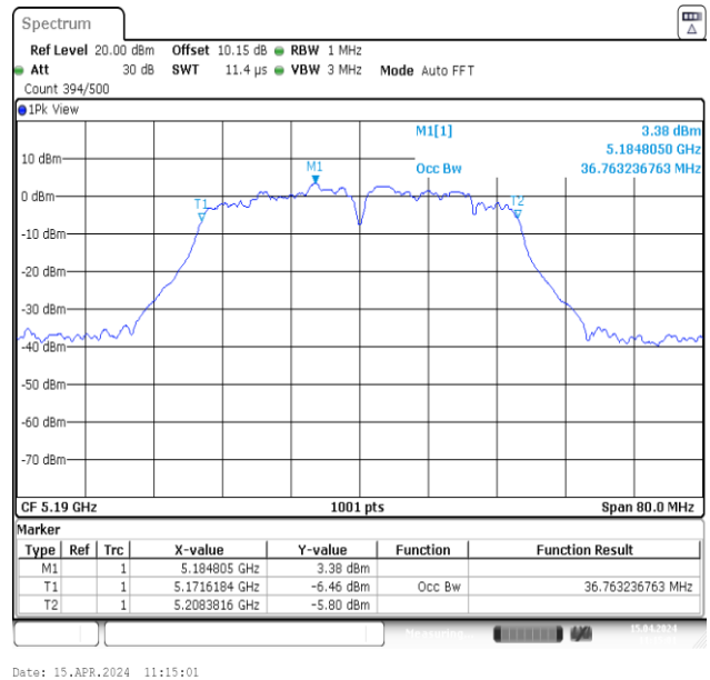
11N40MIMO-Ant2-5190
