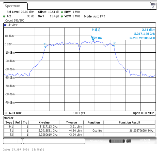
11N40MIMO-Ant2-5310
