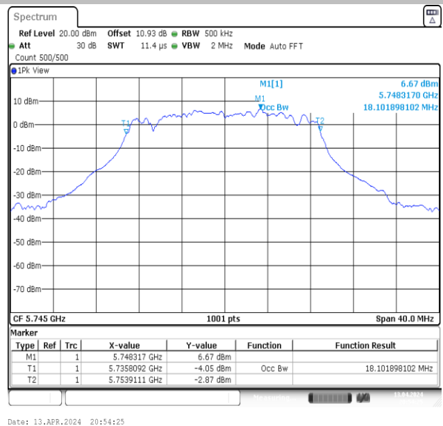
11N20MIMO-Ant2-5745
