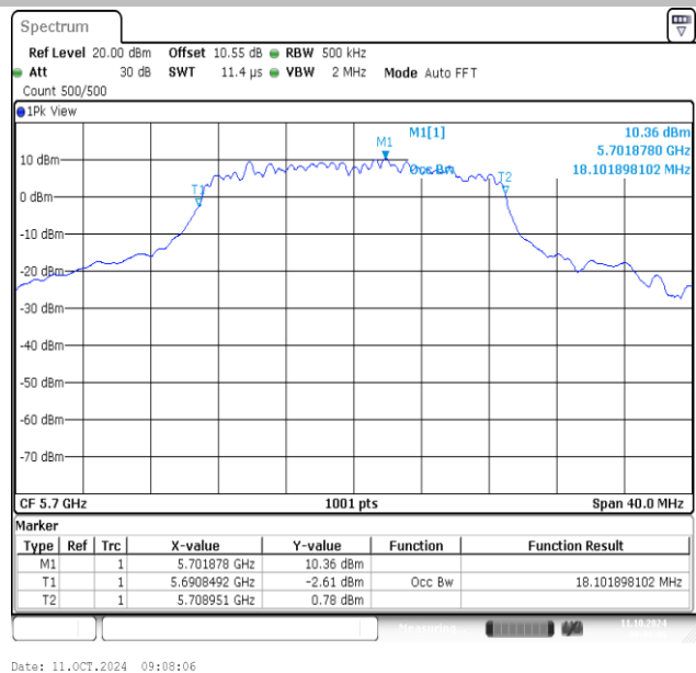
11AC20MIMO-Ant2-5700
