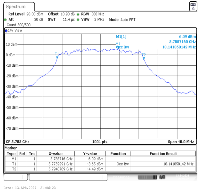
11N20MIMO-Ant2-5785
