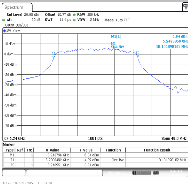
11AC20MIMO-Ant1-5240
