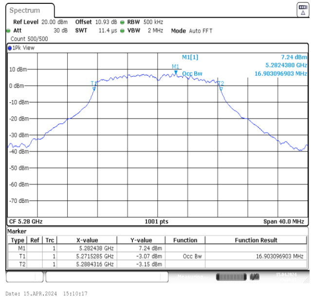
11A-Ant2-5280
