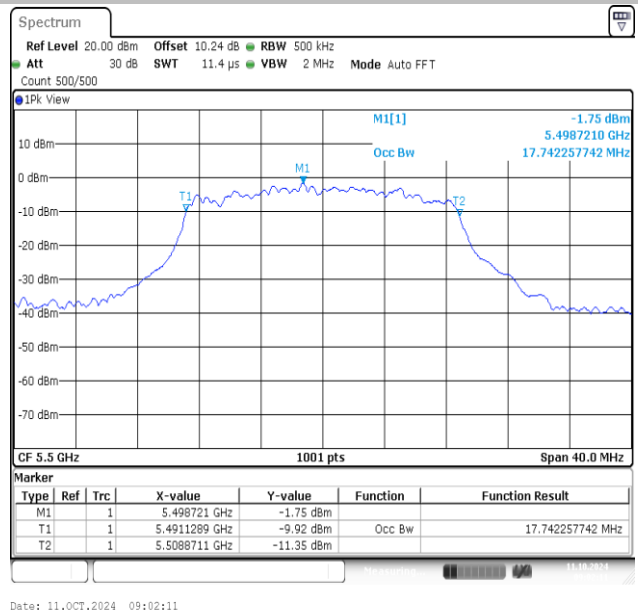
11AC20MIMO-Ant2-5500
