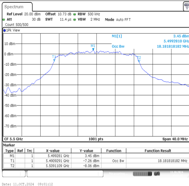
11AC20MIMO-Ant1-5500
