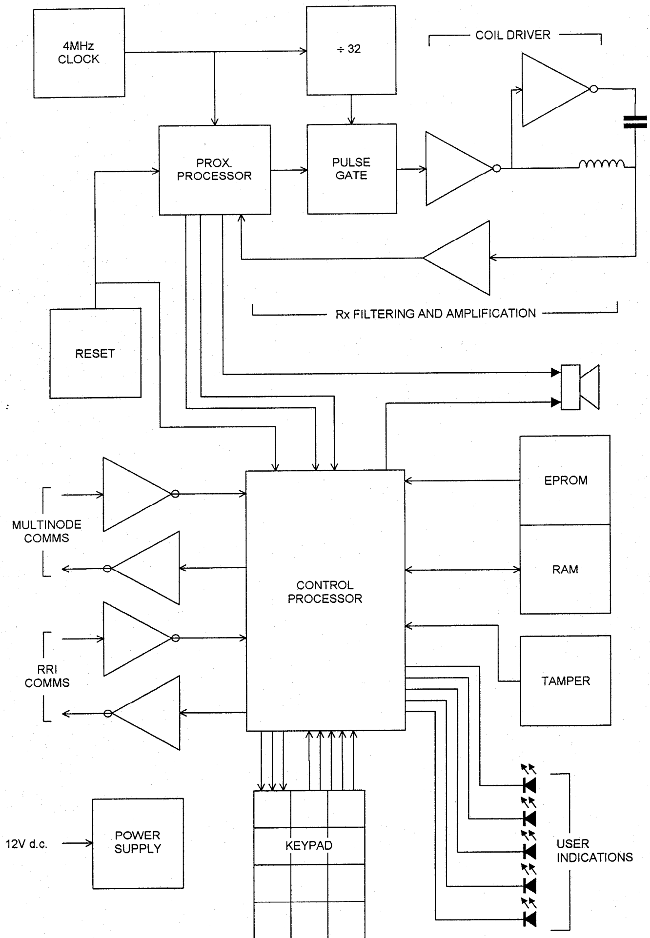
Figure 1: Type 0001 Proximity Reader Block Diagram
