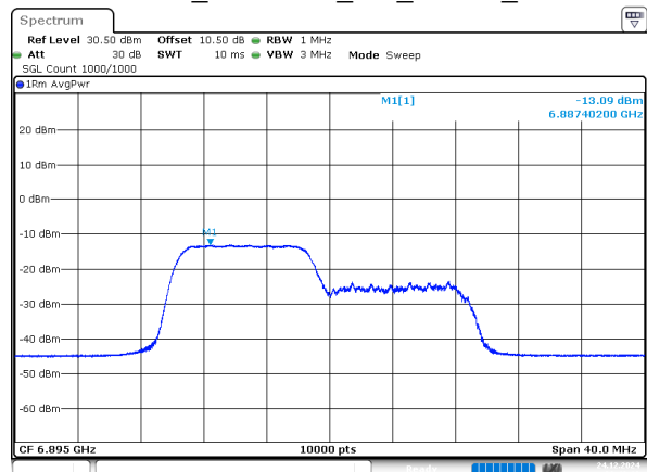
802.11ax20_6895MHz_RU_106/53_Chain 0
