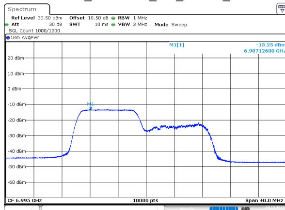
802.11ax20_6995MHz_RU_106/53_Chain 0
