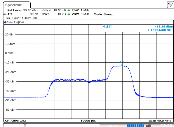
802.11ax20_7095MHz_RU_52/40_Chain 3
