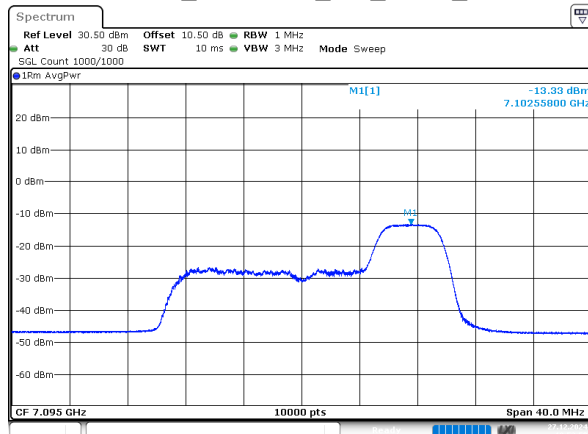
802.11ax20_7095MHz_RU_52/40_Chain 2
