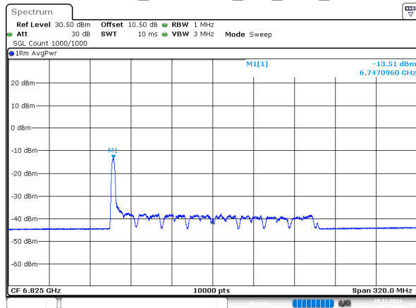
802.11ax160_6825MHz_RU_26/0_Chain 1
