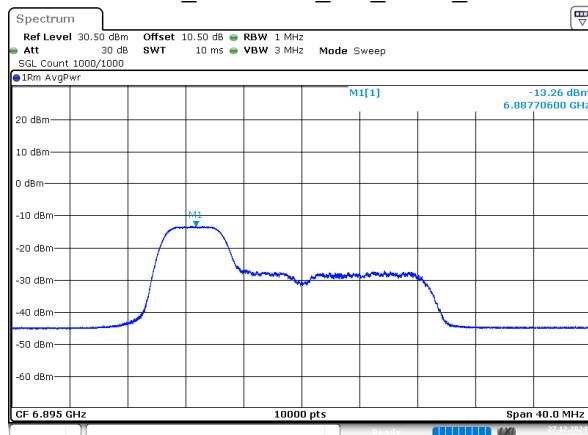
802.11ax20_6895MHz_RU_52/37_Chain 1
