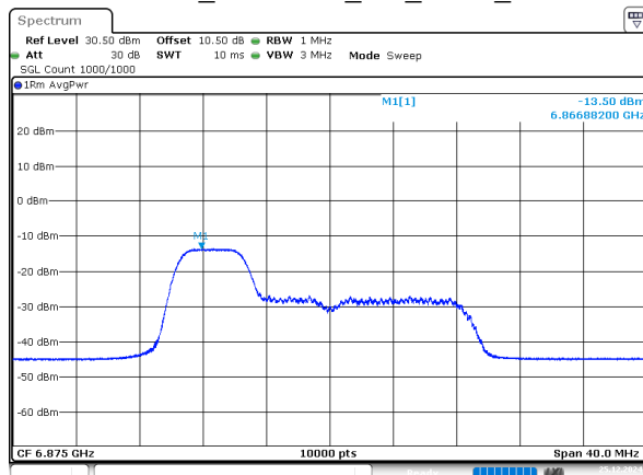
802.11ax20_6875MHz_RU_52/37_Chain 2
