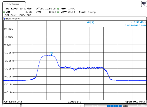
802.11ax20_6875MHz_RU_52/37_Chain 1
