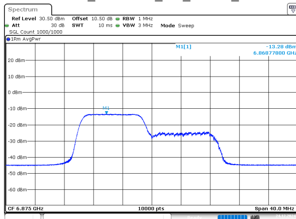
802.11ax20_6875MHz_RU_106/53_Chain 0
