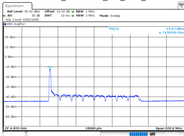
802.11ax160_6825MHz_RU_26/0_Chain 2
