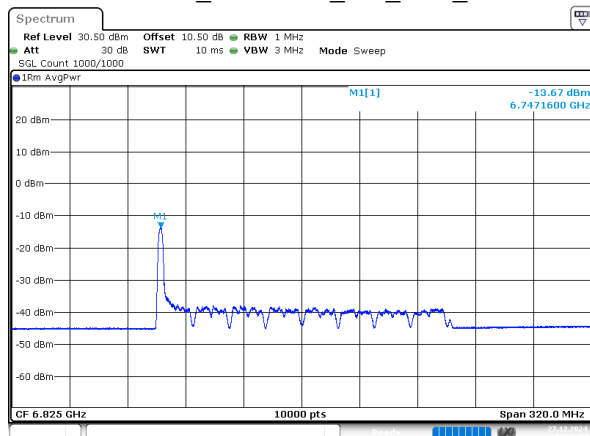
802.11ax160_6825MHz_RU_26/0_Chain 3
