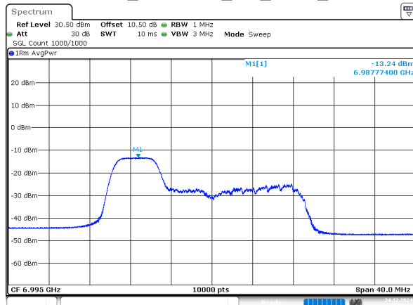
802.11ax20_6995MHz_RU_52/37_Chain 0
