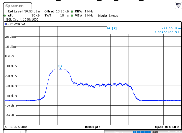
802.11ax20_6895MHz_RU_52/37_Chain 2
