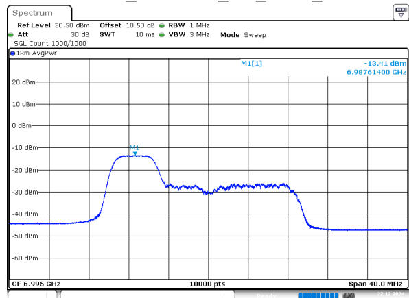
802.11ax20_6995MHz_RU_52/37_Chain 1
