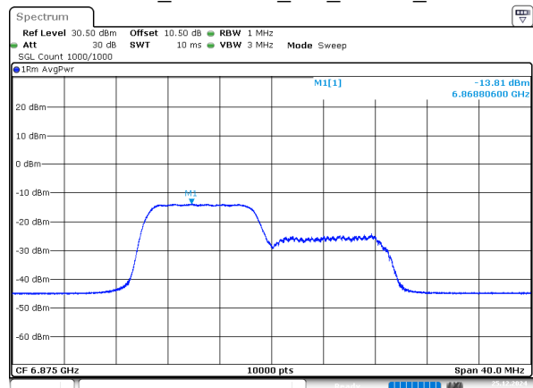
802.11ax20_6875MHz_RU_106/53_Chain 1
