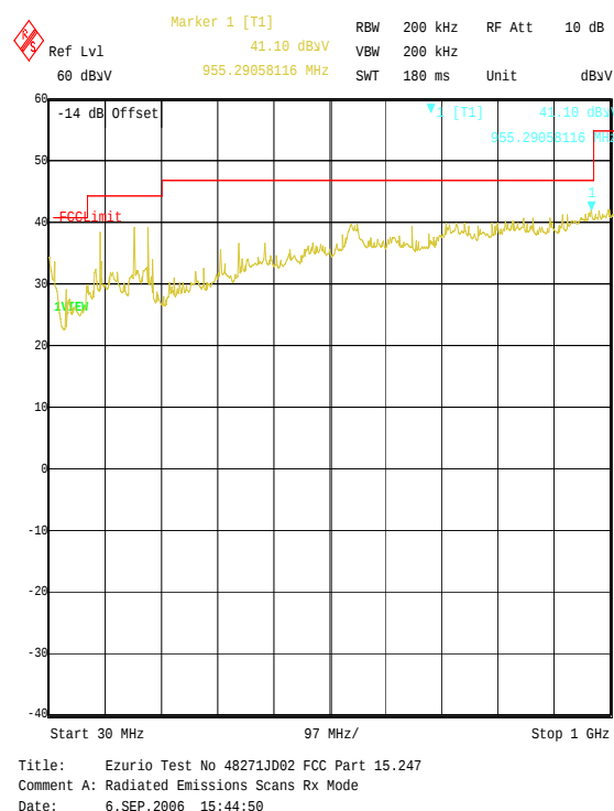
Pre-scan with 3 dBi antenna
