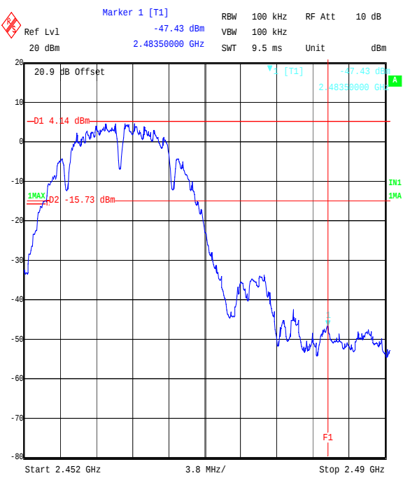
Title: EZURIO 2.4 GHz WLAN Module, FCC Part 15.247 Cond. BandEdge Comment A: 48271JD05 Top Channel DSSS BPSK Date: 8.SEP.2006 16:27:16
