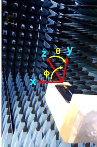
Figure 1: Geometry for SM-S911U for Radiation patterns.
