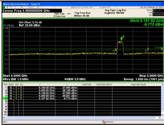
Out Of Band Emission IEEE 802.11ac Channel 38 40MHz Antenna 0
