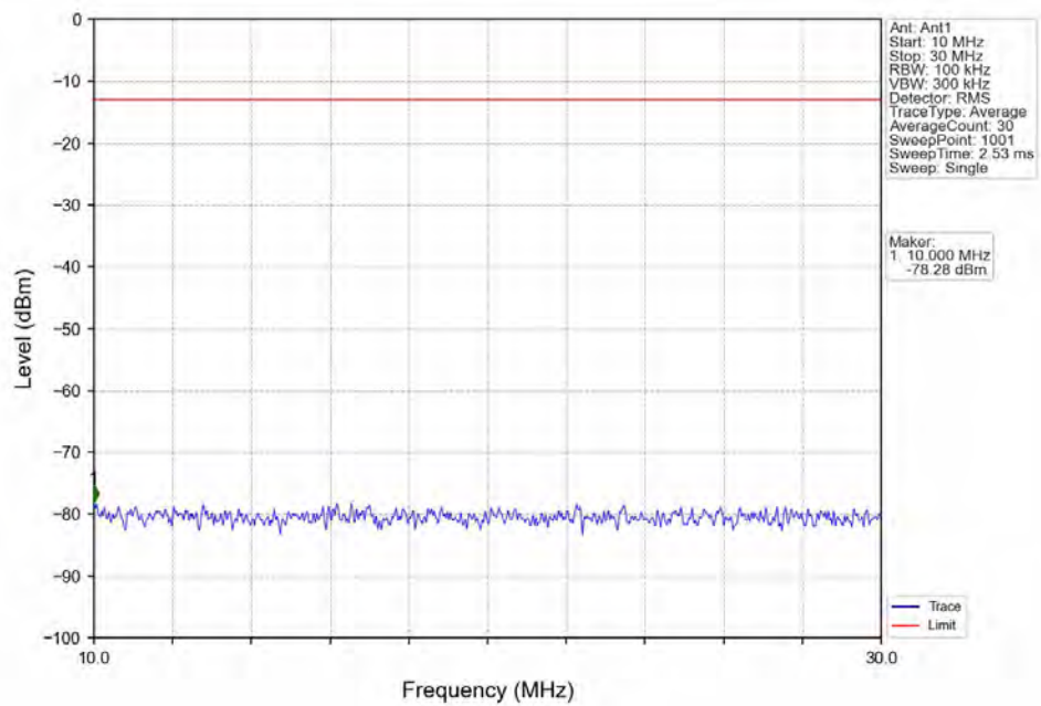
Band12_3MHz_16QAM_LCH_700.5MHz_RB_1_0_NTNV
