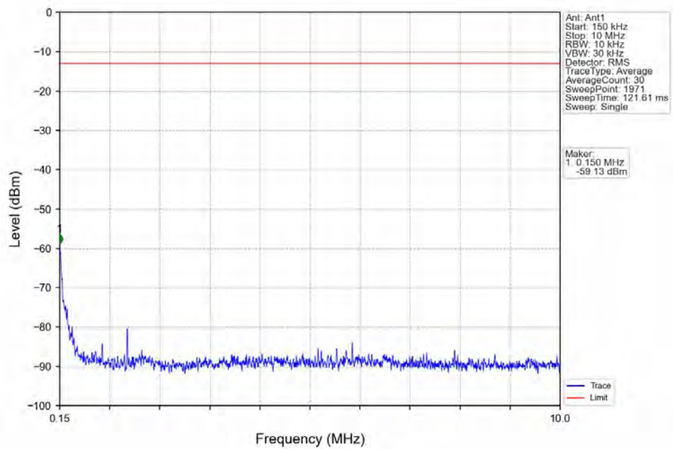
Band12_1.4MHz_QPSK_HCH_715.3MHz_RB_1_0_NTNV
