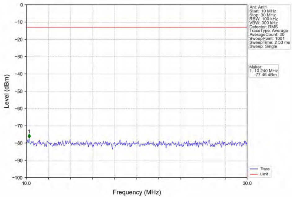
Band12_1.4MHz_16QAM_HCH_715.3MHz_RB_1_0_NTNV
