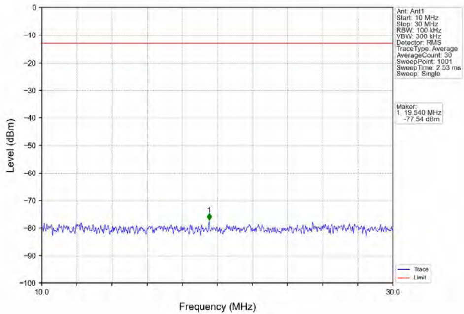
Band12_1.4MHz_16QAM_MCH_707.5MHz_RB_1_0_NTNV
