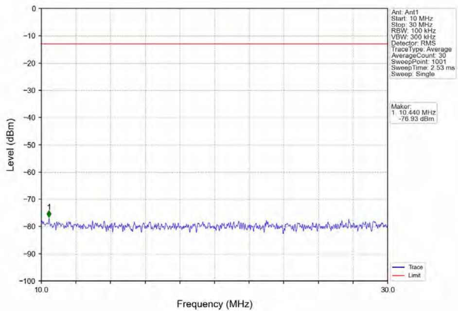
Band12_3MHz_QPSK_LCH_700.5MHz_RB_1_0_NTNV
