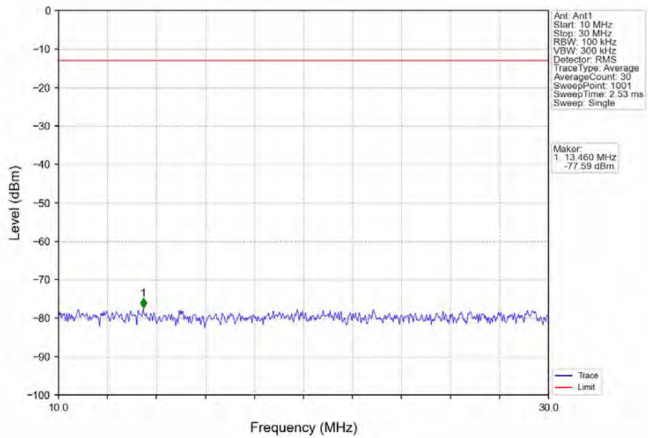
Band12_10MHz_QPSK_HCH_711MHz_RB_1_0_NTNV
