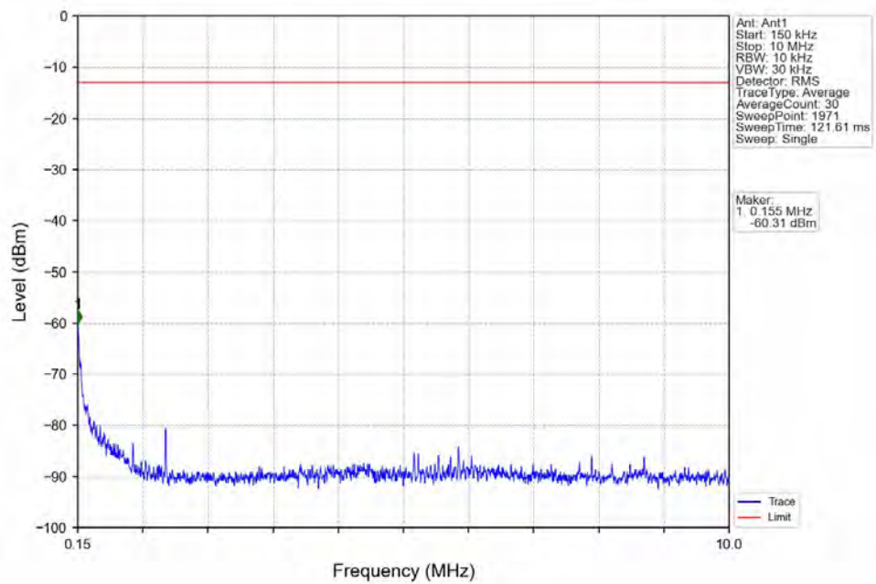
Band12_5MHz_16QAM_MCH_707.5MHz_RB_1_0_NTNV
