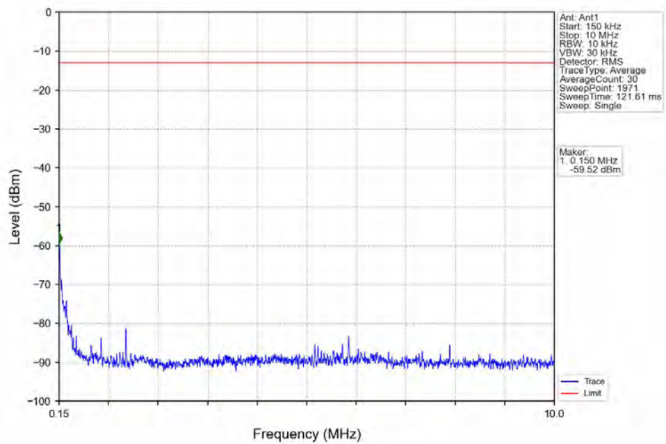
Band12_1.4MHz_16QAM_HCH_715.3MHz_RB_1_0_NTNV
