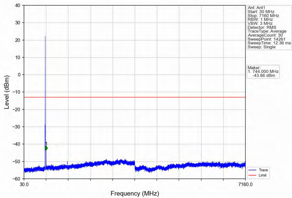
Band12_3MHz_QPSK_HCH_714.5MHz_RB_1_0_NTNV
