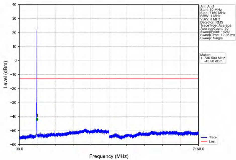
Band12_5MHz_16QAM_MCH_707.5MHz_RB_1_0_NTNV
