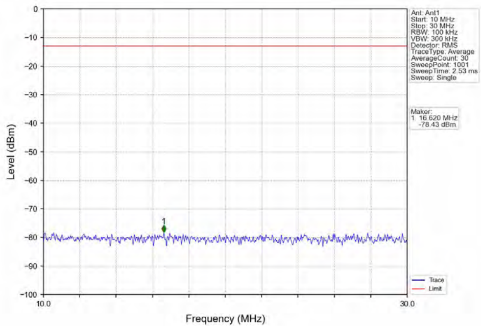
Band12_10MHz_16QAM_LCH_704MHz_RB_1_0_NTNV
