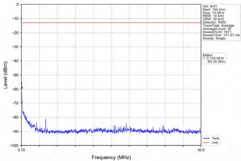
Band12_5MHz_16QAM_HCH_713.5MHz_RB_1_0_NTNV
