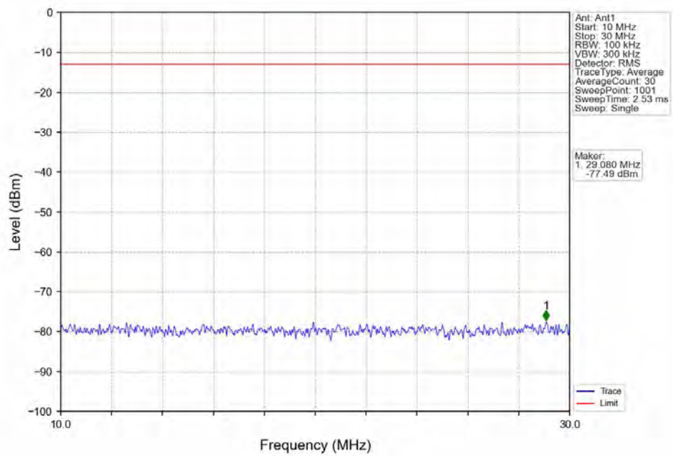
Band12_1.4MHz_QPSK_HCH_715.3MHz_RB_1_0_NTNV
