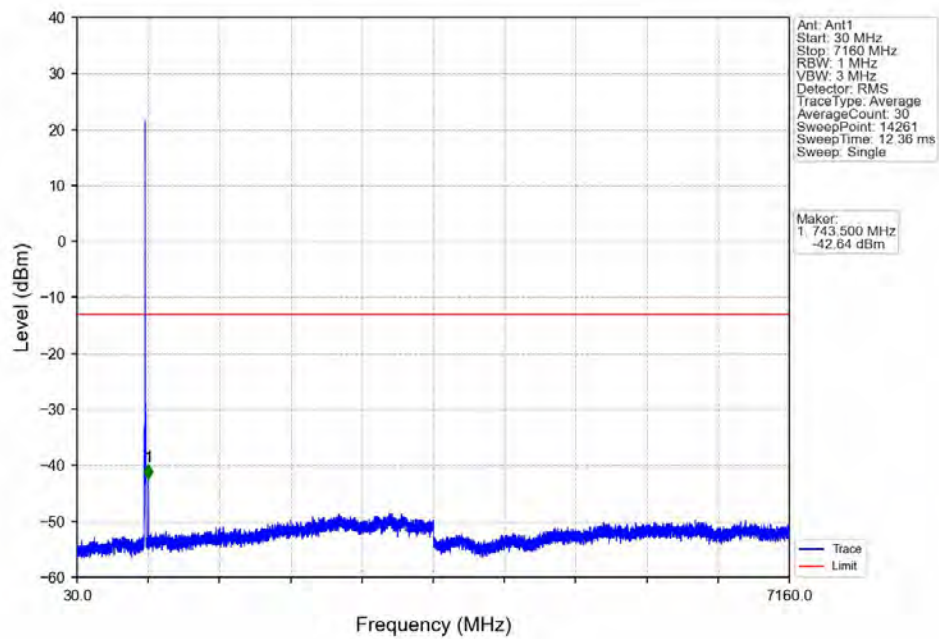
Band12_5MHz_QPSK_HCH_713.5MHz_RB_1_0_NTNV
