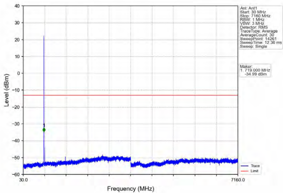
Band12_1.4MHz_QPSK_HCH_715.3MHz_RB_1_0_NTNV
