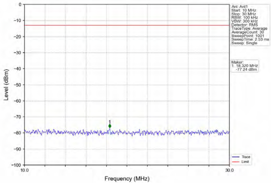
Band12_5MHz_QPSK_HCH_713.5MHz_RB_1_0_NTNV
