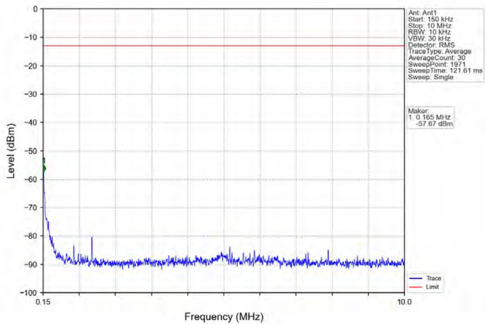
Band12_3MHz_QPSK_HCH_714.5MHz_RB_1_0_NTNV
