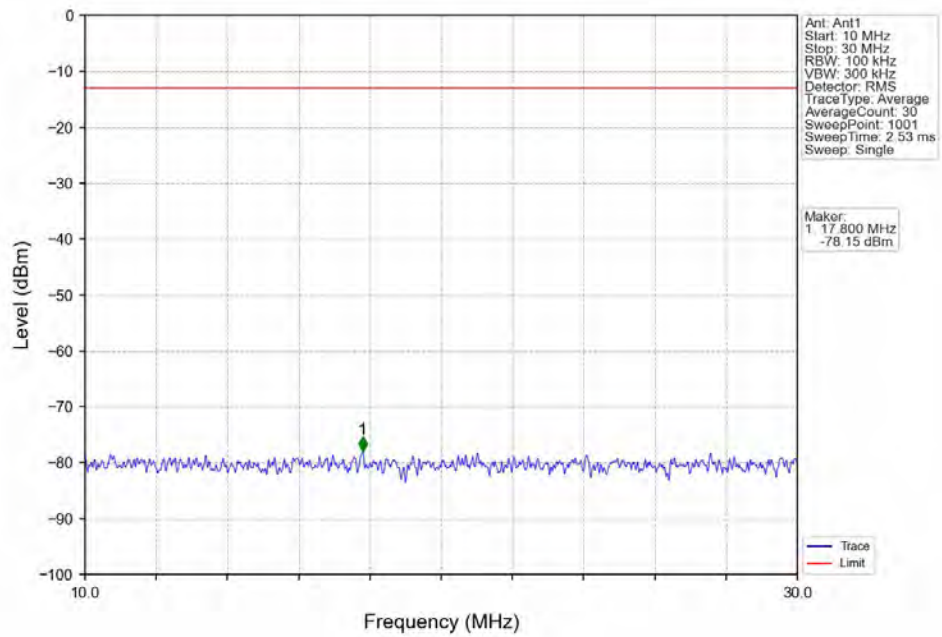
Band12_5MHz_16QAM_MCH_707.5MHz_RB_1_0_NTNV
