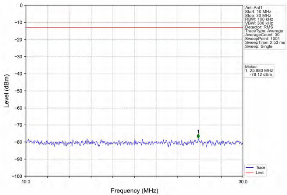
Band12_5MHz_16QAM_LCH_701.5MHz_RB_1_0_NTNV
