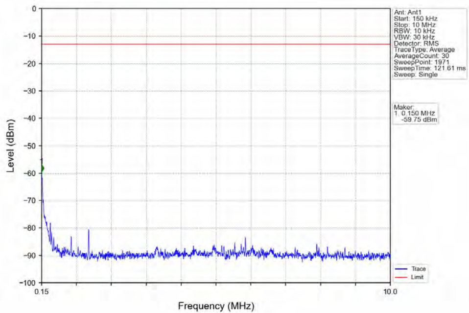
Band12_3MHz_16QAM_MCH_707.5MHz_RB_1_0_NTNV
