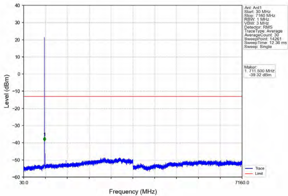
Band12_1.4MHz_QPSK_MCH_707.5MHz_RB_1_0_NTNV
