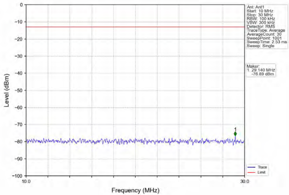
Band12_3MHz_QPSK_HCH_714.5MHz_RB_1_0_NTNV
