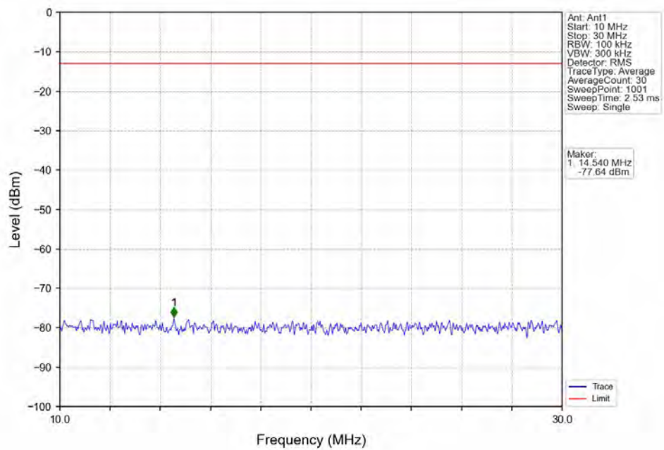
Band12_1.4MHz_QPSK_LCH_699.7MHz_RB_1_0_NTNV
