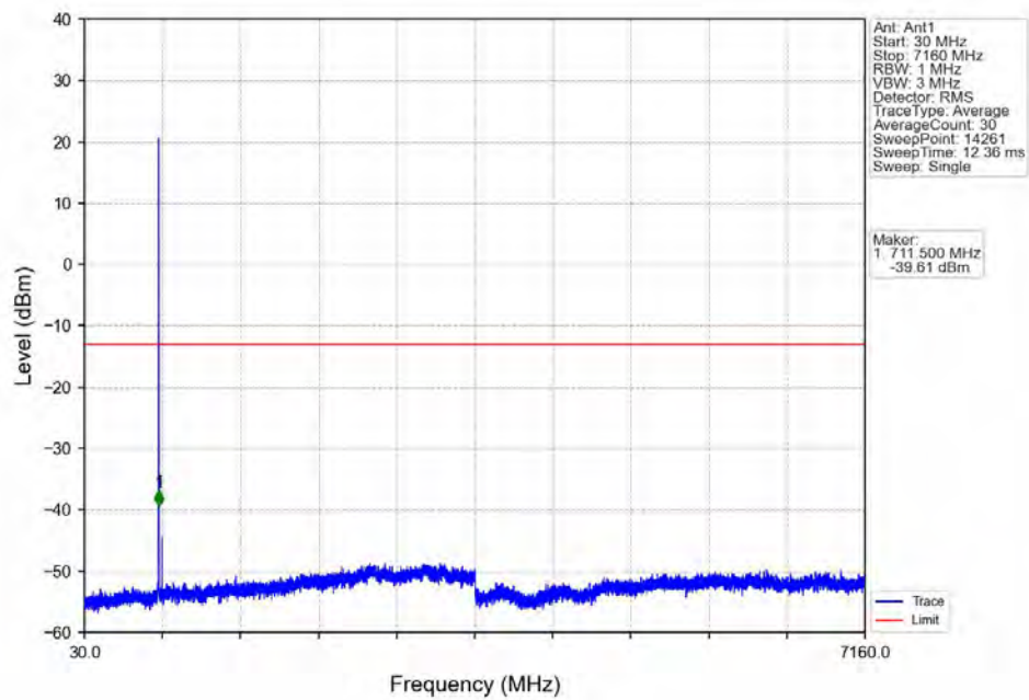
Band12_1.4MHz_16QAM_MCH_707.5MHz_RB_1_0_NTNV
