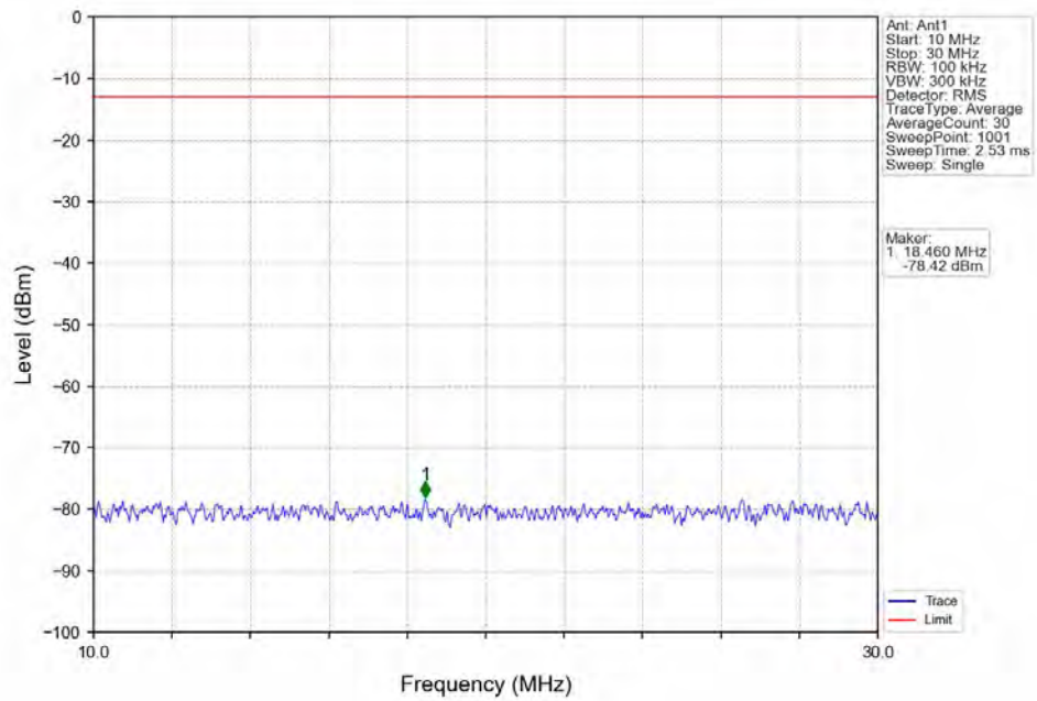
Band12_10MHz_16QAM_MCH_707.5MHz_RB_1_0_NTNV
