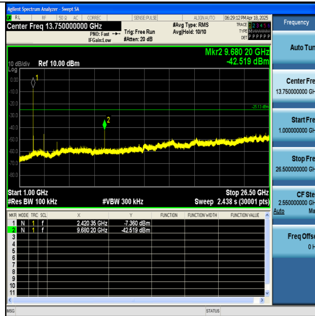
SRD-Ant1-2420-1000~26500-PASS
