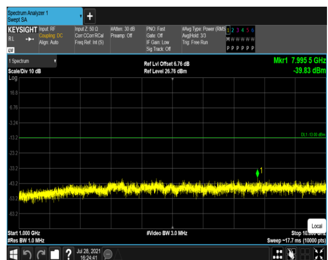
Band26-15MHz-16QAM-26915:1000~10000MHz
