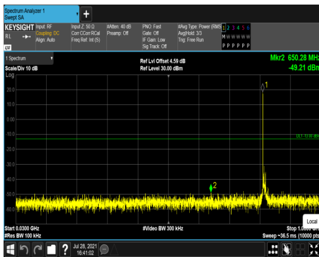
Band26-15MHz-QPSK-26765:30~1000MHz
