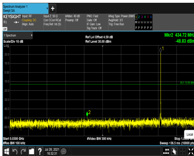
Band26-1.4MHz-16QAM-26783:30~1000MHz
