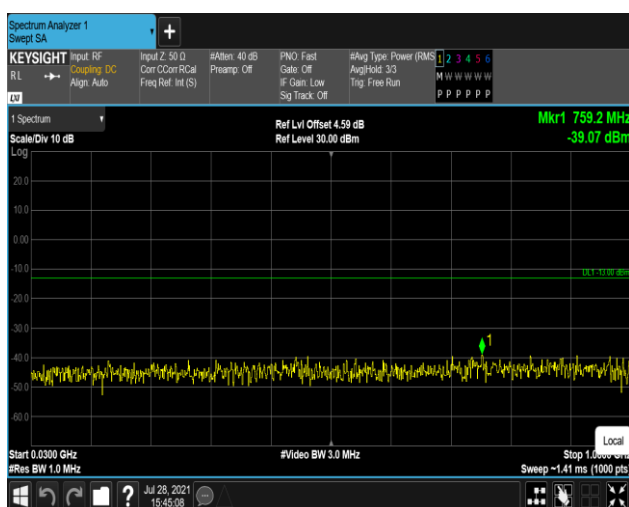
Band25-1.4MHz-16QAM-26683:30~1000MHz
