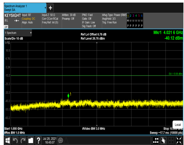
Band26-15MHz-16QAM-26865:1000~10000MHz
