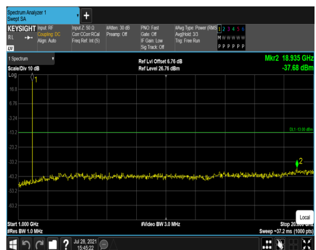
Band25-1.4MHz-16QAM-26683:1000~20000MHz
