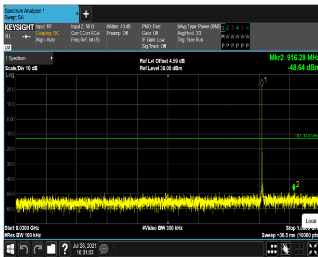
Band26-1.4MHz-QPSK-26740:30~1000MHz
