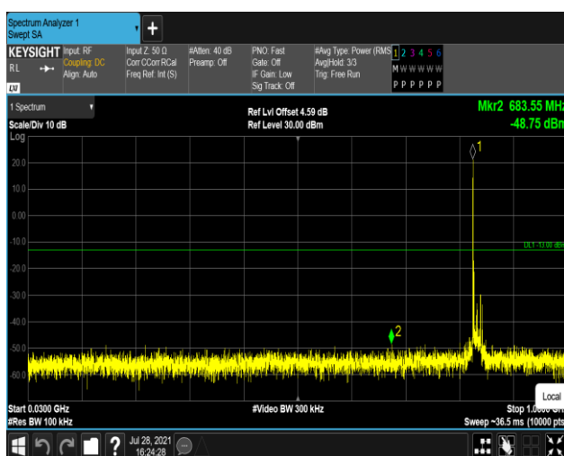
Band26-15MHz-16QAM-26915:30~1000MHz
