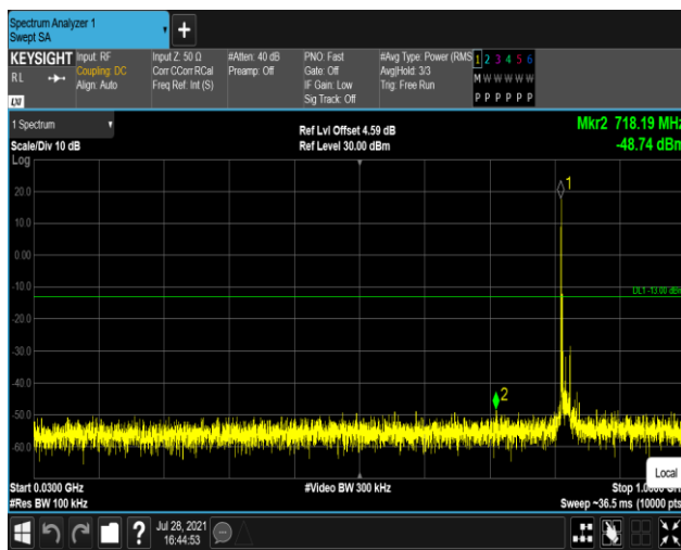
Band26-15MHz-16QAM-26865:30~1000MHz
