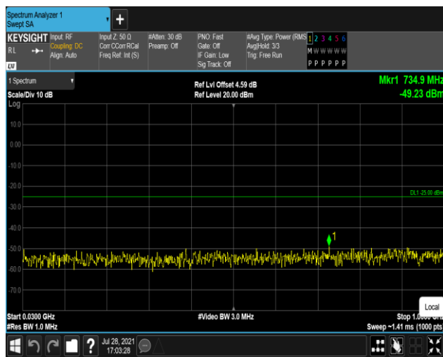
Band41-5MHz-16QAM-40065:30~1000MHz
