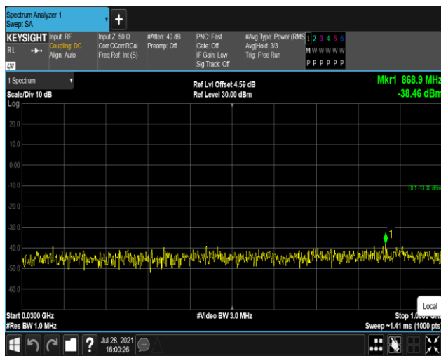
Band25-20MHz-16QAM-26365:30~1000MHz
