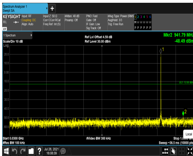
Band26-1.4MHz-QPSK-26915:30~1000MHz
