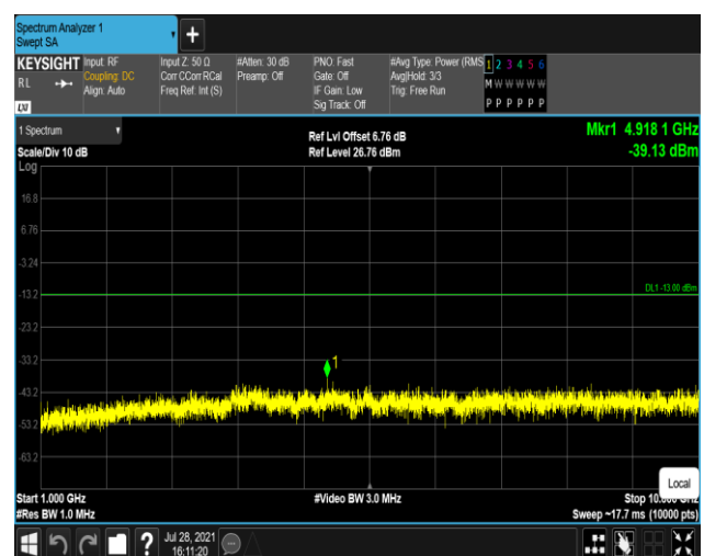
Band26-1.4MHz-16QAM-27033:1000~10000MHz
