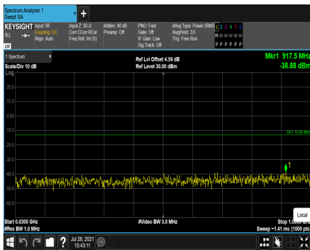
Band25-1.4MHz-16QAM-26365:30~1000MHz
