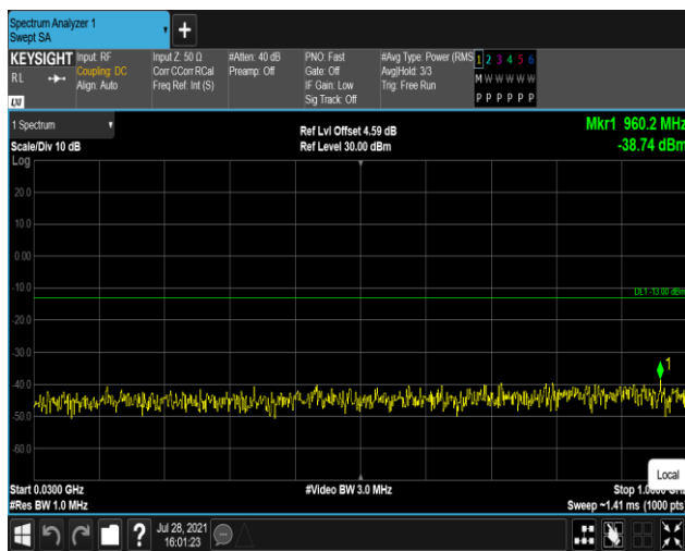
Band25-20MHz-16QAM-26590:30~1000MHz
