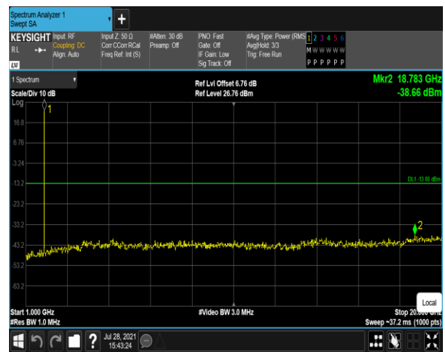
Band25-1.4MHz-16QAM-26365:1000~20000MHz
