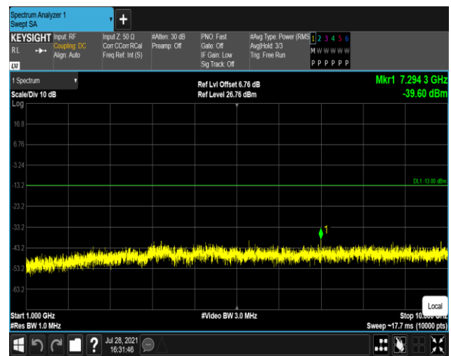
Band26-1.4MHz-16QAM-26740:1000~10000MHz
