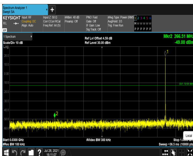
Band26-1.4MHz-16QAM-27033:30~1000MHz
