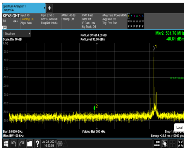
Band26-15MHz-QPSK-26965:30~1000MHz
