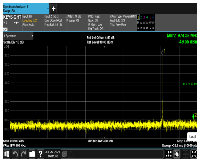
Band26-1.4MHz-16QAM-26740:30~1000MHz
