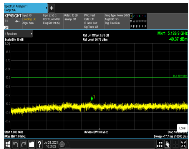
Band26-1.4MHz-16QAM-26915:1000~10000MHz
