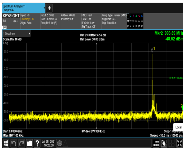
Band26-15MHz-QPSK-26915:30~1000MHz
