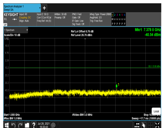
Band26-1.4MHz-16QAM-26783:1000~10000MHz
