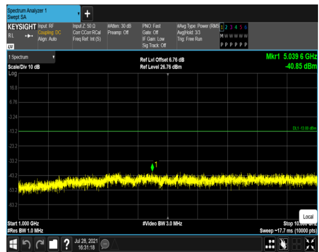
Band26-1.4MHz-QPSK-26740:1000~10000MHz
