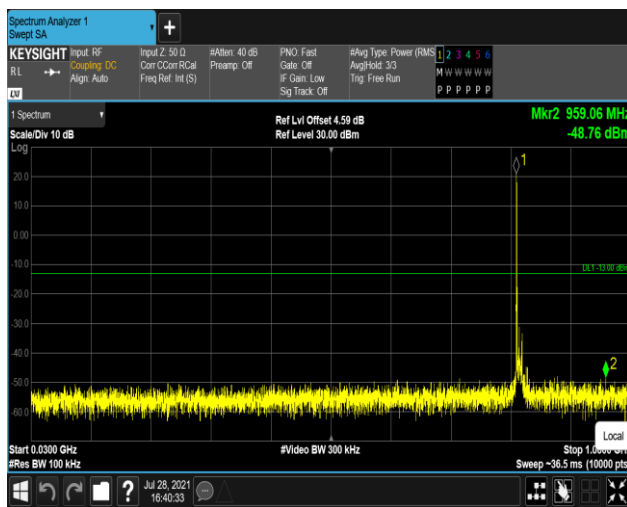
Band26-10MHz-16QAM-26740:30~1000MHz
