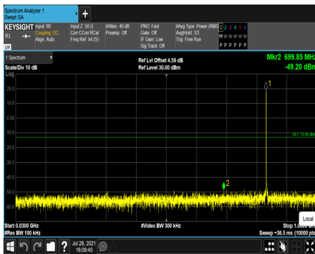
Band26-1.4MHz-QPSK-27033:30~1000MHz
