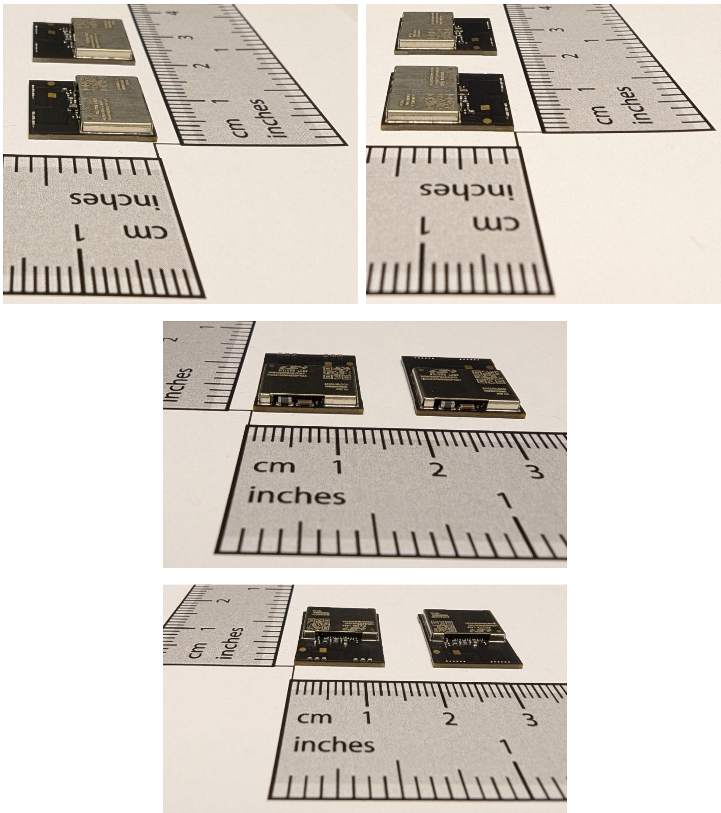
Figure 3: Side Views of the MGM260P32A and MGM260P32N Modules
