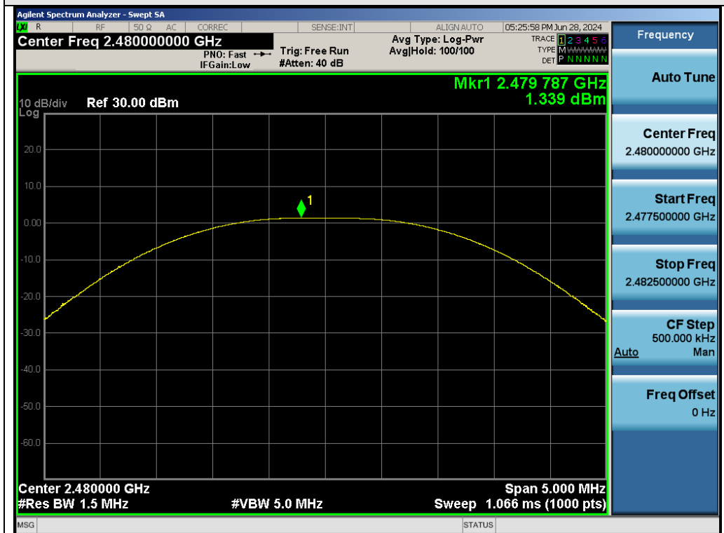
Test_Graph_GFSK_ANT2_2480_Peak Power
