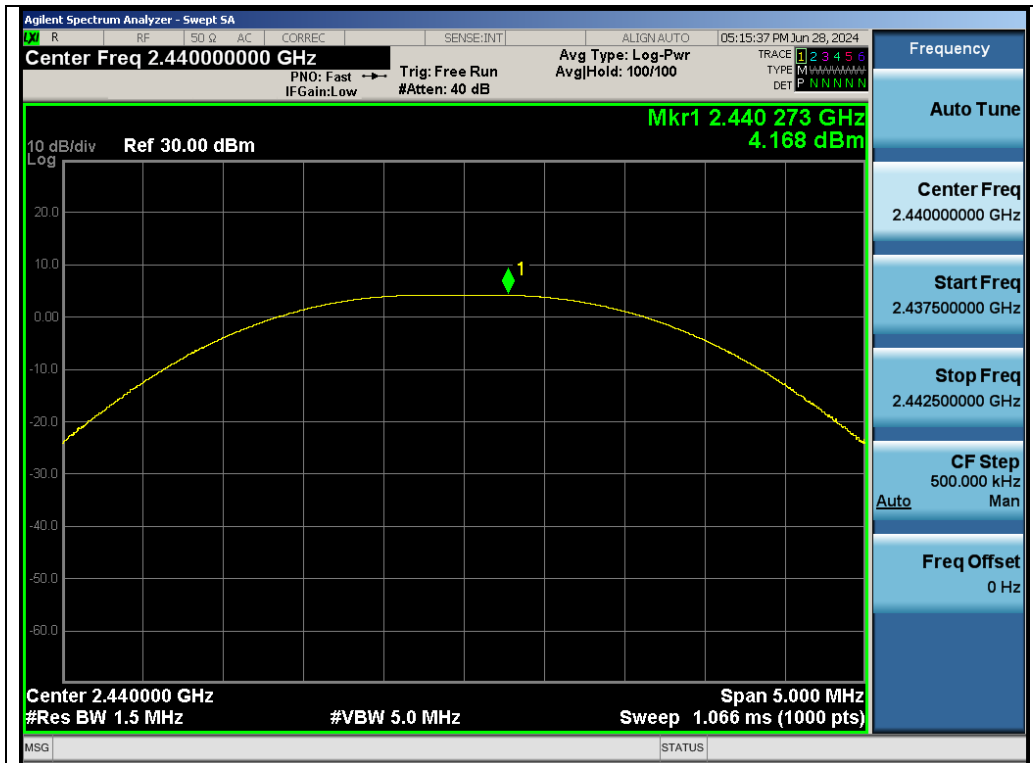
Test_Graph_GFSK_ANT2_2440_Peak Power
