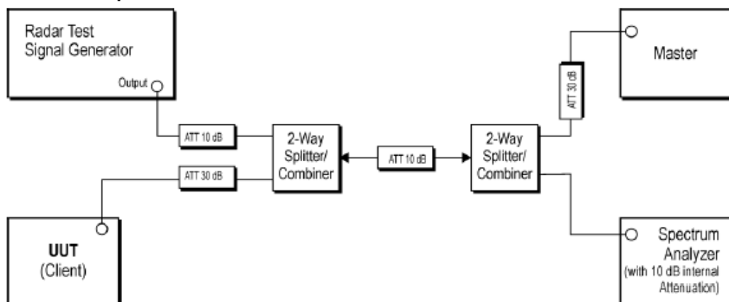
Figure 17: Channel Closing Transmission Time, Channel Move Time and Non-Occupancy Period Conducted test setup
