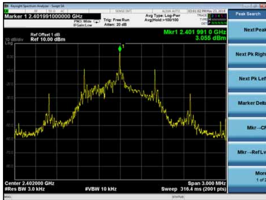
Mode 1 CH00(2402MHz)
