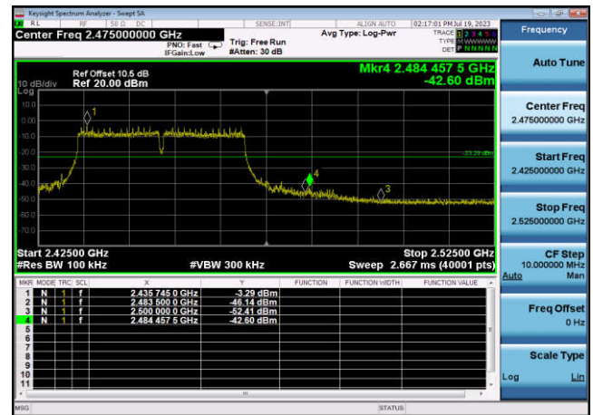
,Plot 2,Band Edge-802.11n(HT40) ,2452MHz,Ant2
