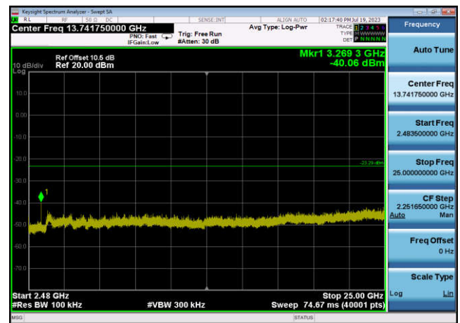
,Plot 4,2483.5MHz~25000MHz-802.11n(HT 40),2452MHz,Ant2
