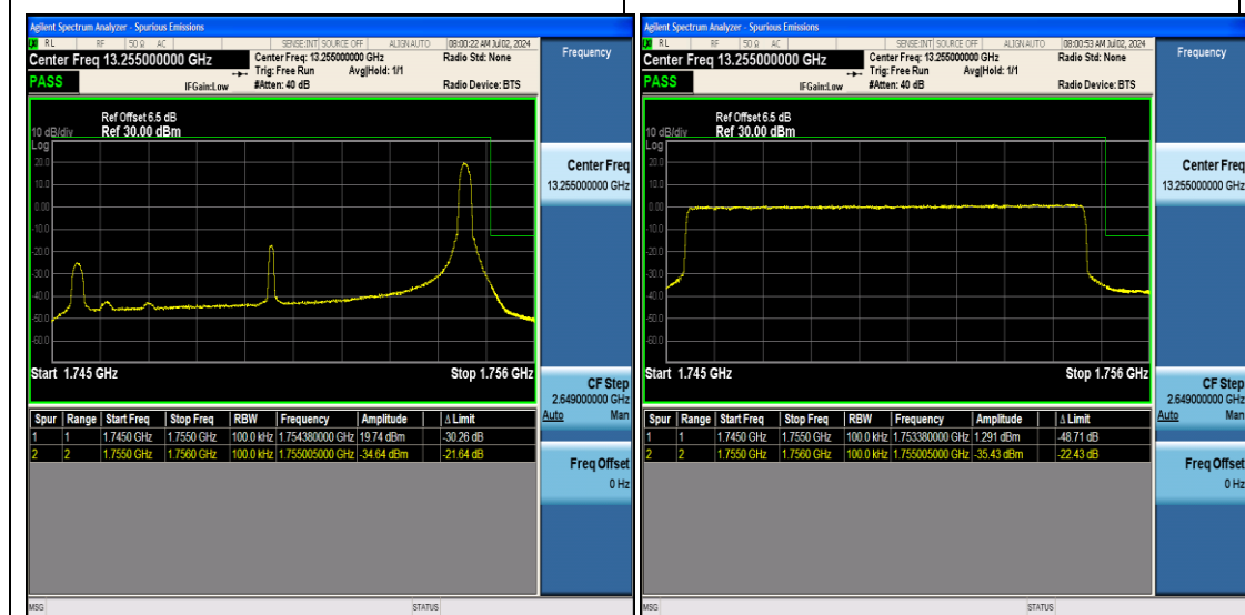
Band4_10MHz_16QAM_20000_50RB#0
