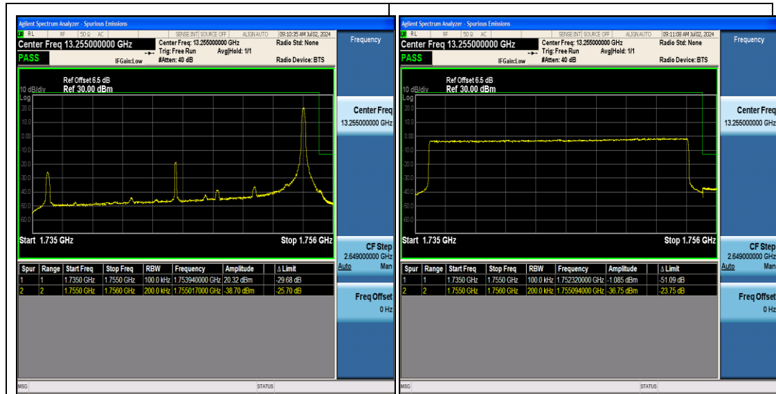
Band4_20MHz_16QAM_20300_1RB#99
