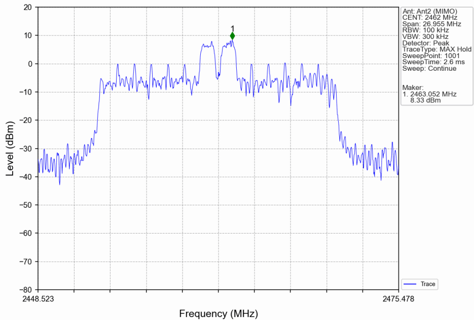
802.11ax(HEW20)_HCH_2462MHz_RU26_Mid_Ant2 (MIMO)_NTNV
